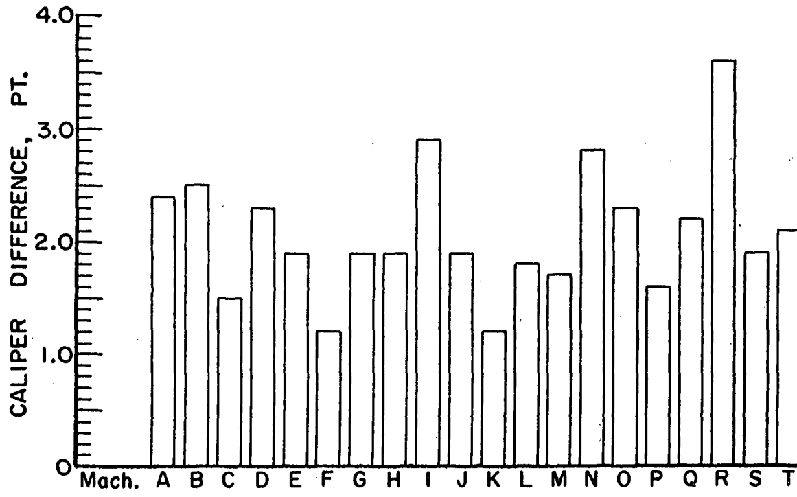
Figure 2. Comparison of the Caliper Differences Between Consecutive Flutes of Single-Faced Board, November, 1960
