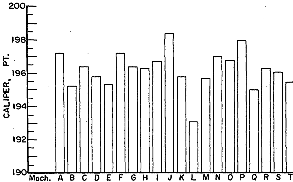
Figure 1. Comparison of Caliper Results on Single-Faced Board November, 1960
