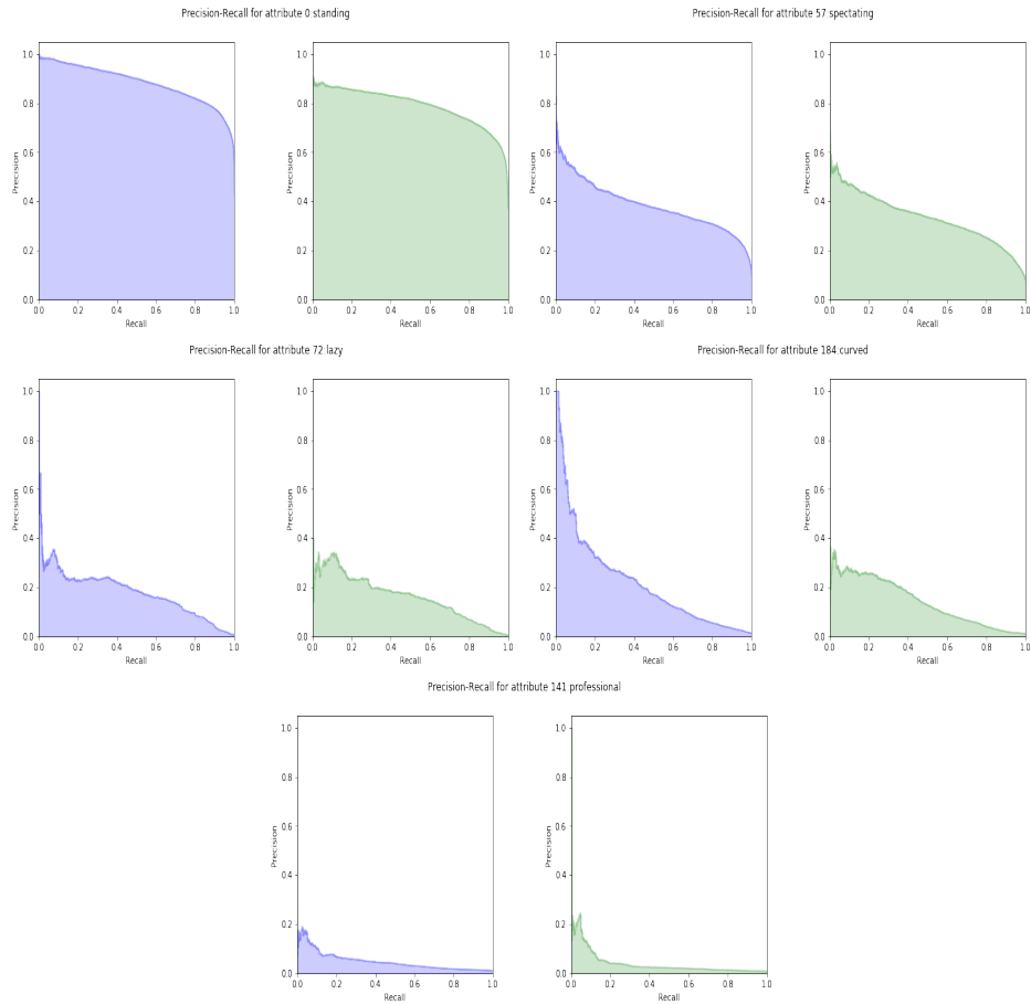
Figure 4.1: Precision Recall Curves of Attribute labels with different number of samples in the training set. Attribute Module Network predictions are represented as the purple curves, while the baseline ResNet101 model predictions are represented as green curves.
