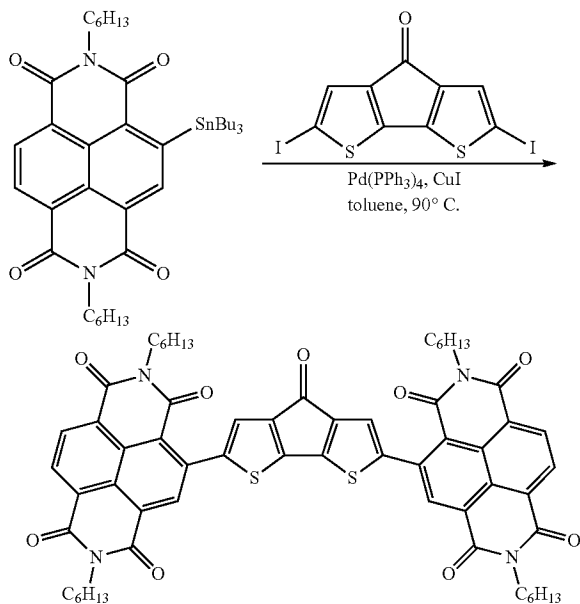
NDI-DTO-NDI
