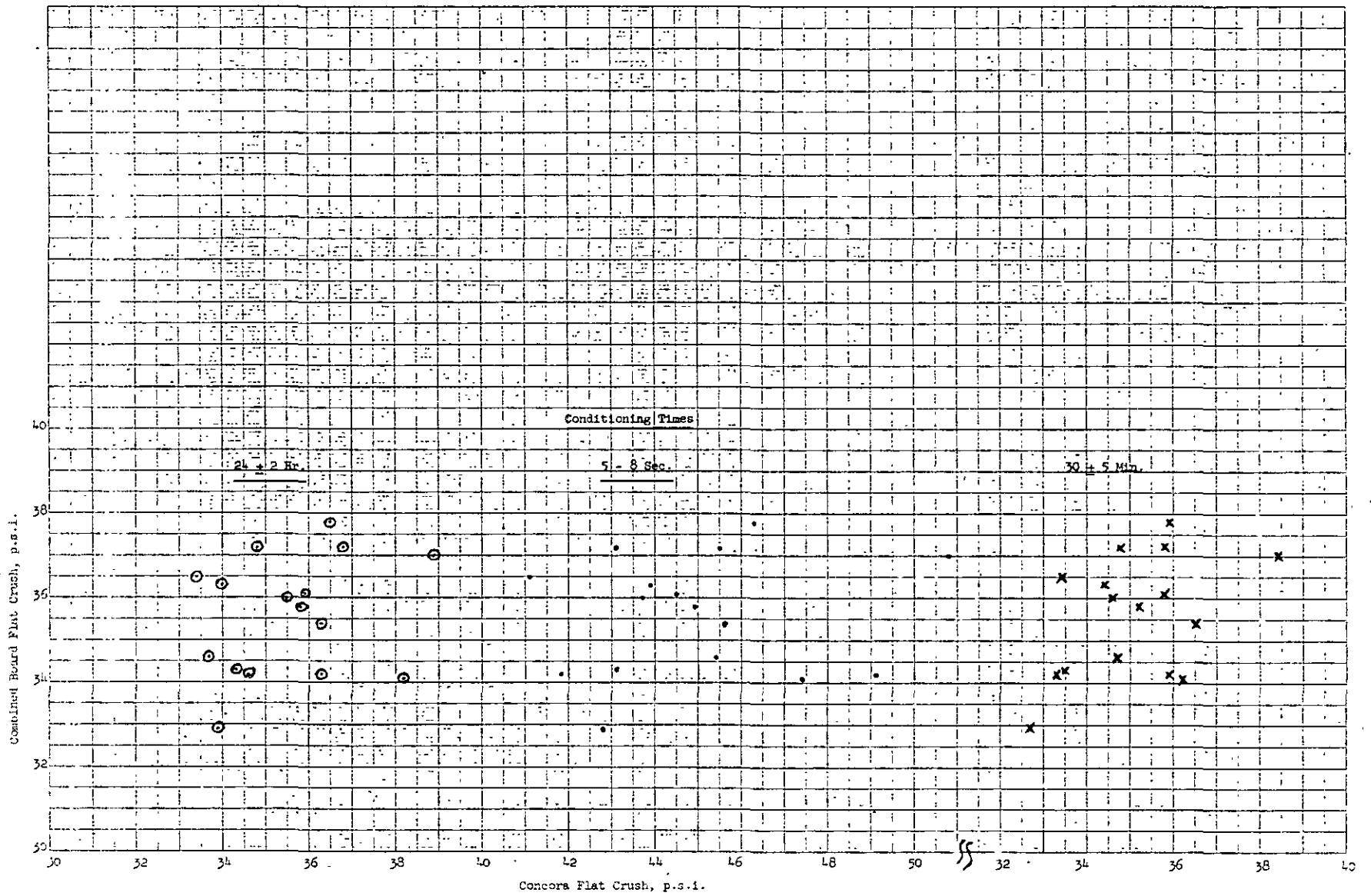
Figure 2. Mill B: Mill Test Results
