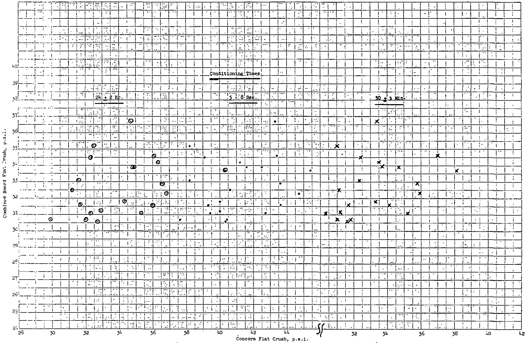
Figure 6. Mill D: Mill Test Results
