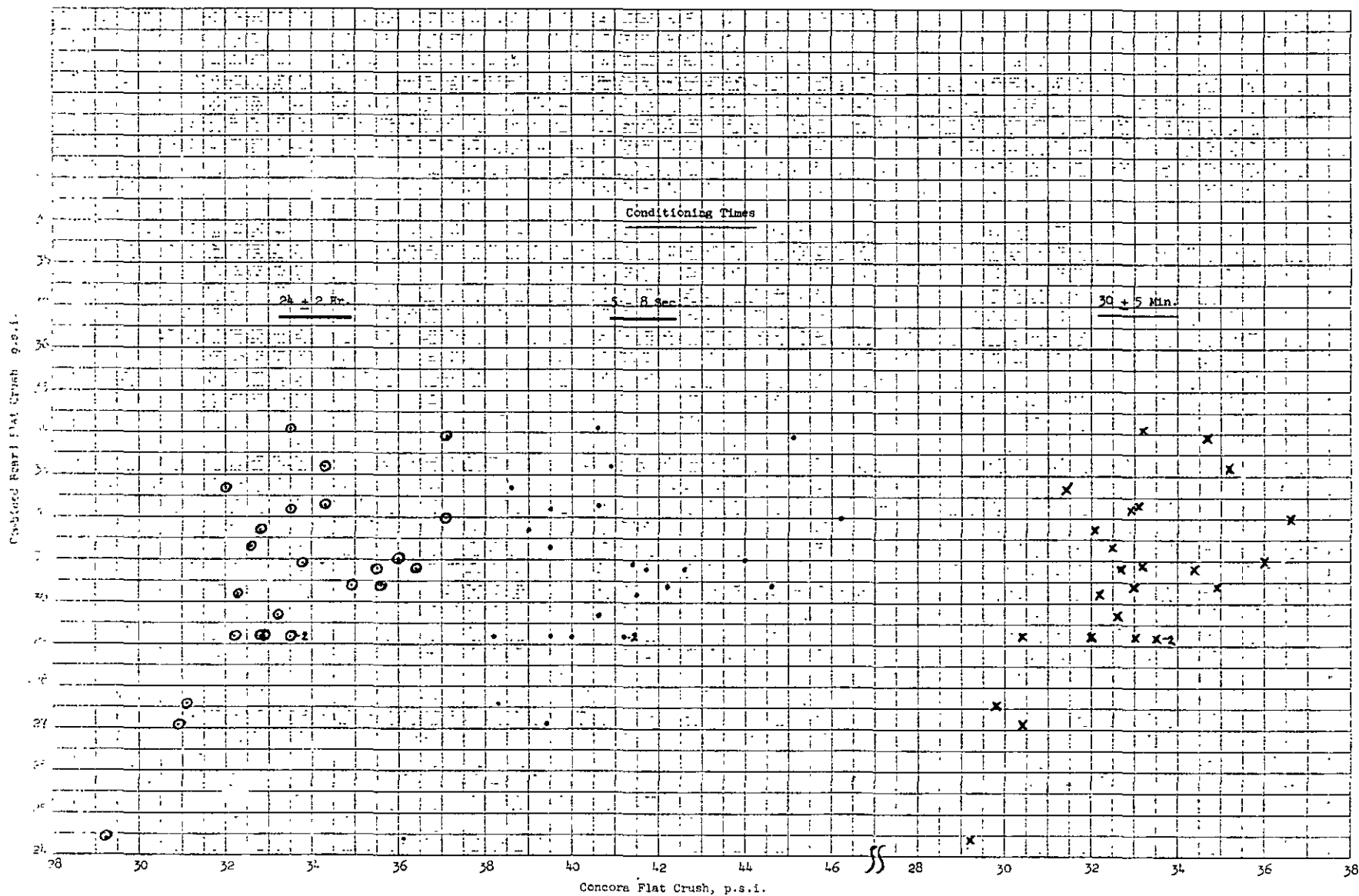
Figure 7. Mill D: Institute Test Results
