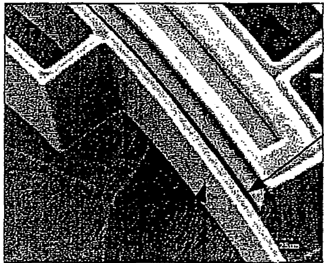
POLYSILICON RING FIG. 10F
