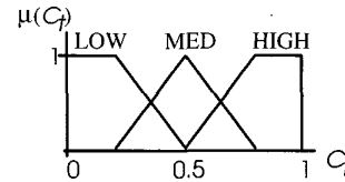
Figure 5. Fuzzy sets for traction coefficient.
