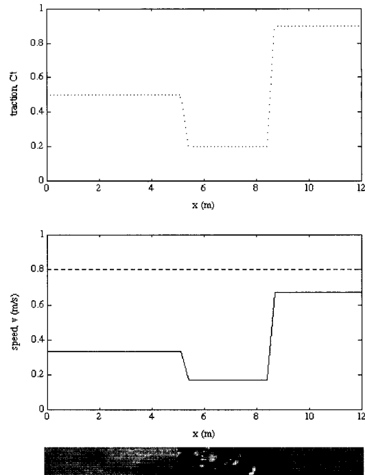
Figure 11. Speed modulation for traction management.
