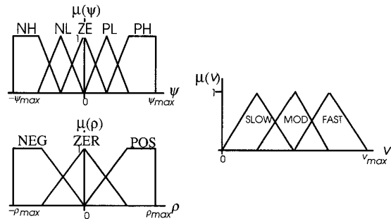
Figure 1. Membership functions for safe attitude.
