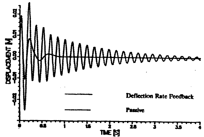
Figure 5c. Deflection Of RALF's Link 2 For The Commanded Motion In 5a.
