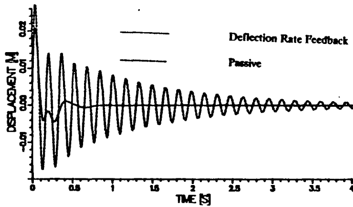
Figure 5b. Deflection Of RALF's Link 1 For The Commanded Motion In 5a.
