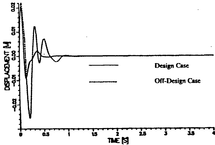
Figure 4b. Deflection Of Link 1 For Design And Off-Design Nominal Angles ( \theta_3 And \theta_4 ). (RALF Has Initial Deflection Rates.)
