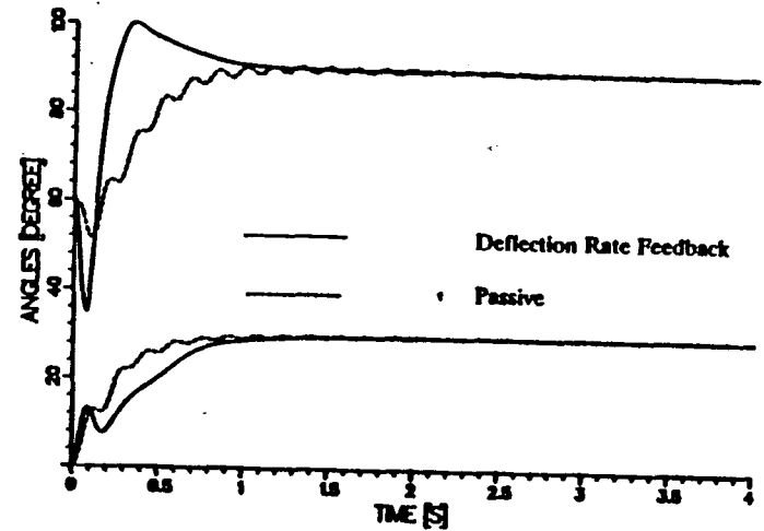
Figure 5a. Joint Response To A Step Command In Position of \theta_3 and \theta_4 For Two Control Schemes. (RALF's Initial Conditions Are Zero.)
