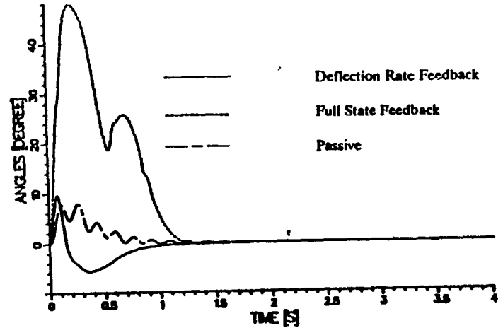
Figure 2. Motion Of SAM's First Joint ( \theta_3 ) For 3 Control Schemes. (RALF Has Initial Deflection Rates).
