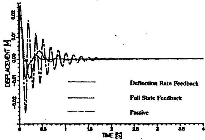
Figure 3. Deflection Of RALF's Link 1 For 3 Control Schemes. (RALF Has Initial Deflection Rates).
