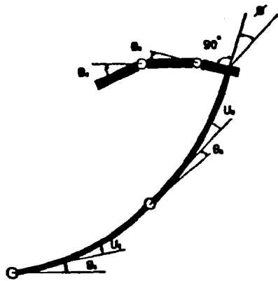
Figure 1. The System Of This Study: The Robotic Arm, Large And Flexible (RALF), Joints 1 And 2; Carrying The Small Articulated Manipulator (SAM), Joints 3 And 4.
