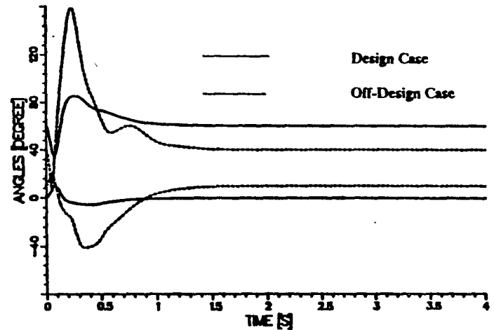
Figure 4a. Excursions Of SAM's Joints For Design And Off-Design Nominal Angles ( \theta_3 And \theta_4 ). (RALF Has Initial Deflection Rates).
