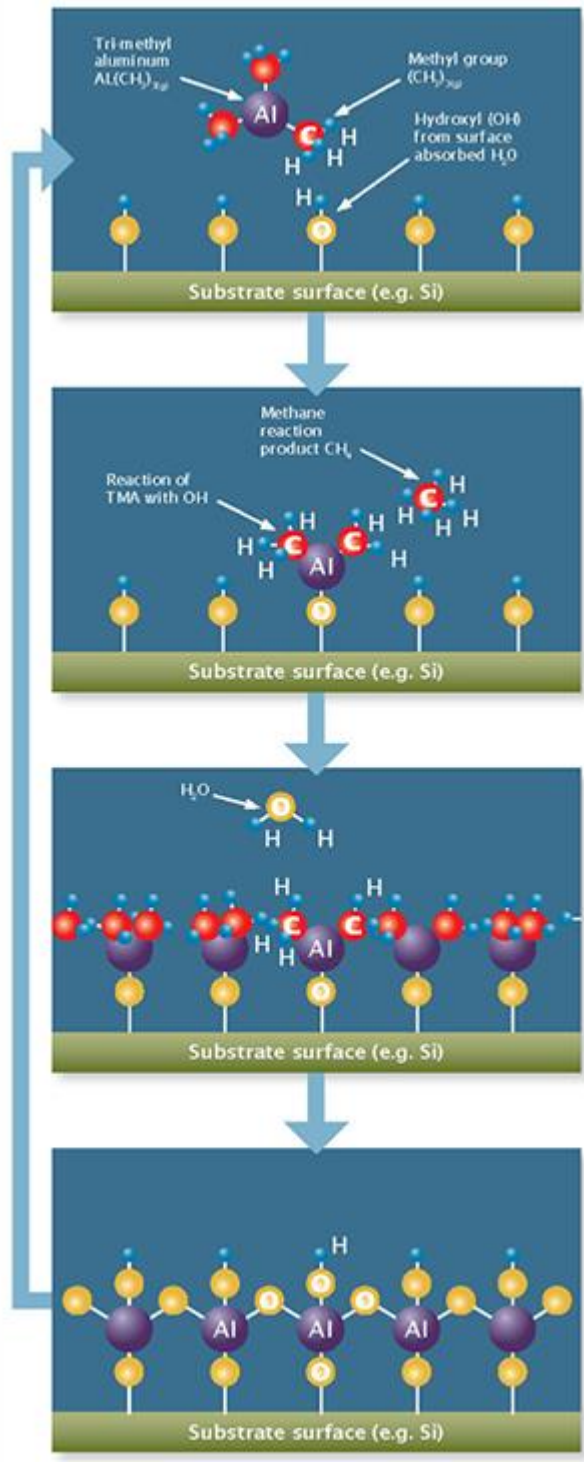
Figure 9. An illustration of ALD process of Al 2 O 3 (Ultratech Inc.) [43].
