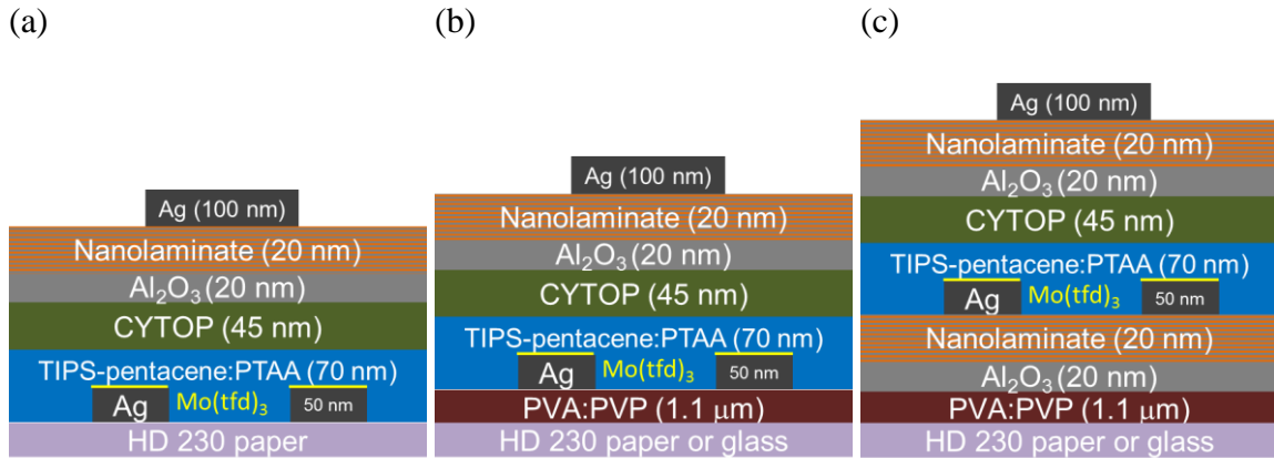
Figure 47. (a) The OFET structure of type 1. (b) The OFET structure of type 2 and 3. (c) The OFET structure of type 4 and 5.
