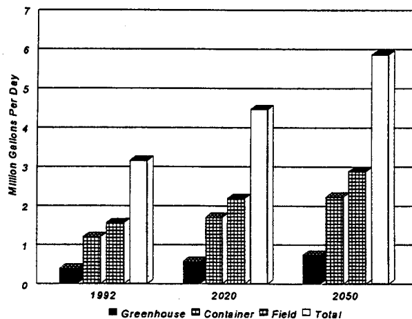
Figure 3. Projected water demand for irrigation - Georgia nurseries and turf.
