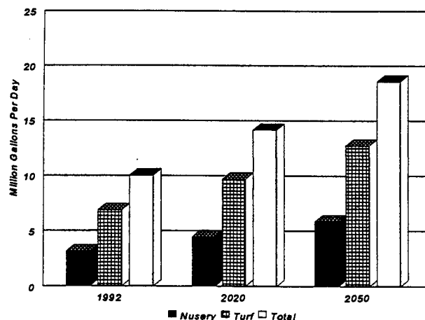
Figure 2. Projected water demand for irrigation - Georgia nurseries.
