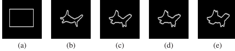
Figure 3. Influence of \sigma for the Kernel PCA method (exponential kernel) applied on binary maps. Morphing results of an arbitrary shape are presented for the “Shark” training set. (a): Initial shape, (b): Morphing result for \sigma = 3 , (c): \sigma = 7 , (d): \sigma = 9 , (e): \sigma = 15 .
