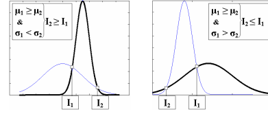
Figure 4. Probability density functions. Thick line: p(I \in \text{Object}) ; Thin line: p(I \in \text{background}) . It is straightforward to see that p(I \in \text{Object}) > p(I \in \text{Object}) for I_1 \leq I \leq I_2 , when \sigma_1 < \sigma_2 and for I \geq I_1 and I \leq I_2 , when \sigma_1 > \sigma_2 .
