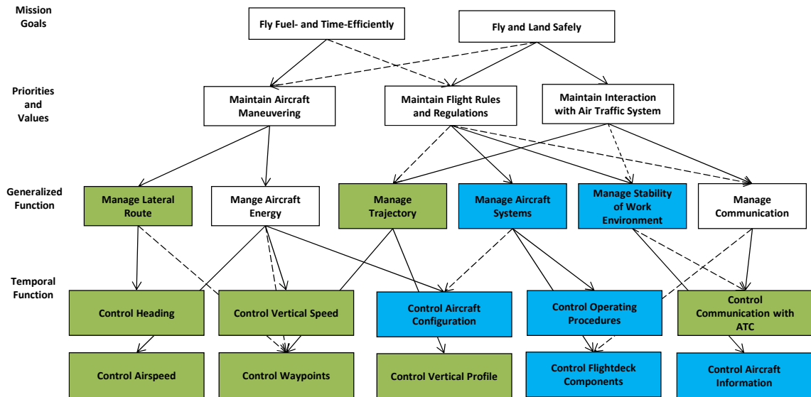
Figure 35 Highly-automated function allocation (FA1, functions entirely allocated to the automation are green-coded and to the pilot are blue-coded)
