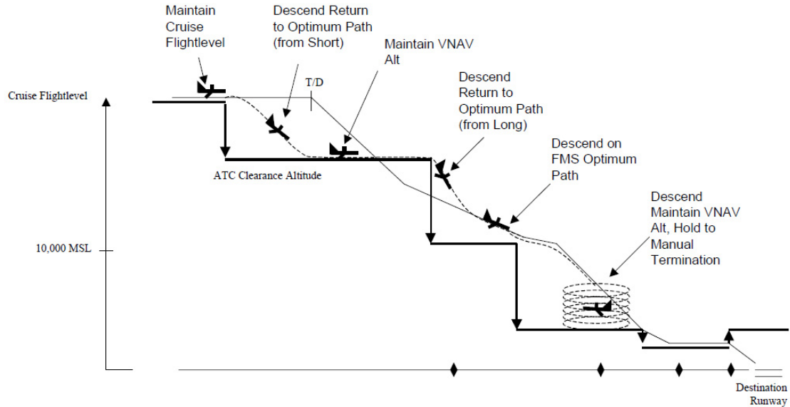
Figure 9 Selecting the VNAV button during a STAR invokes one of the VNAV commanded behaviors depending on the position of the aircraft relative to the FMS optimal path, the ATC clearance altitude, holding pattern at a fix, etc. (figure copied from Sherry, et al., 2001)
