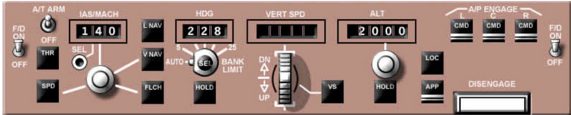
Figure 8 Mode control panel (MCP) in Boeing 747 (photo retrieved from http://www.meriweather.com/747/fd-747.html )
