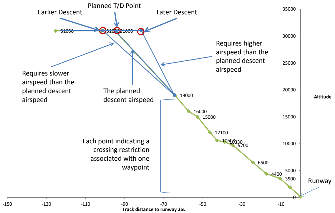
Figure 5 An example of a vertical profile of the arrival and approach phases with three potential initiation of descent (early, normal, and late descents) assuming the air traffic instruction is given as “descend to flight level 190”)
