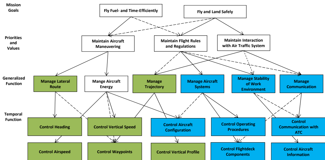
Figure 36 Mostly-automated function allocation (FA2, functions entirely allocated to the automation are green-coded and to the pilot are blue-coded)
