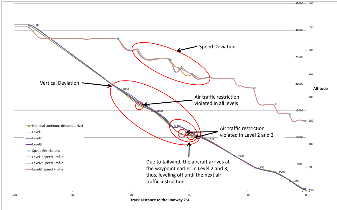
Figure 25 Vertical profile of three levels of unexpected tailwind scenario (SC3)
