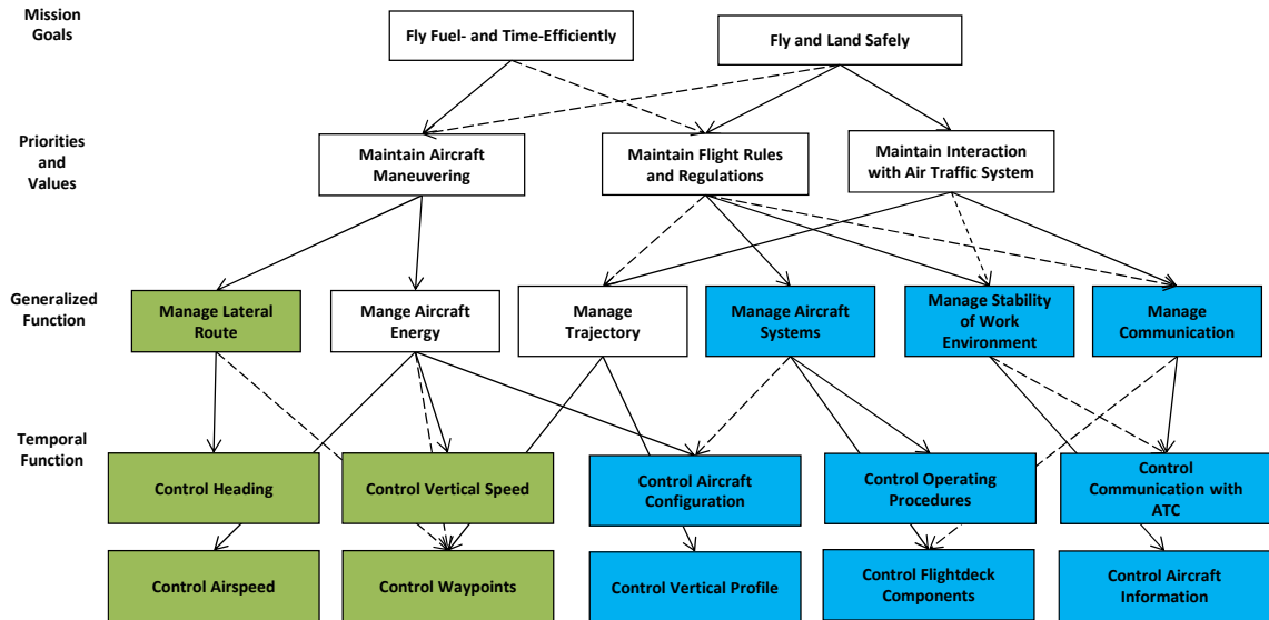
Figure 18 Assessing coherency: high level of coherency (functions assigned to automation are green-coded while functions assigned to the pilot are blue-coded)
