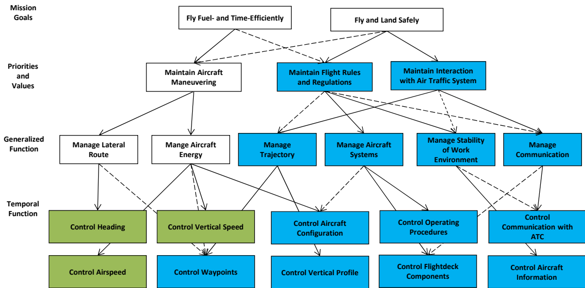
Figure 38 Mostly-manual function allocation (FA4, functions entirely allocated to the automation are green-coded and to the pilot are blue-coded)
