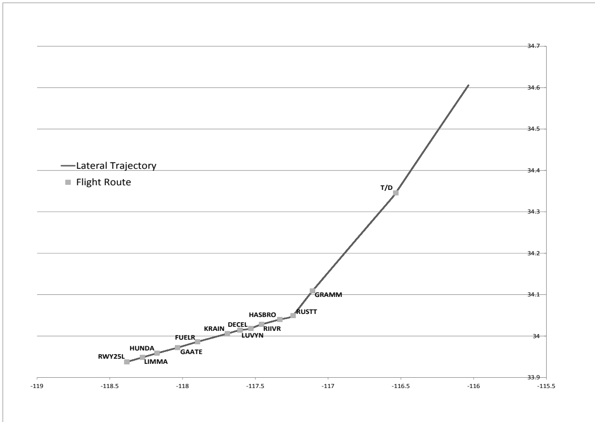
Figure 20 Lateral profile of nominal (continuous descent) arrival and approach scenario
