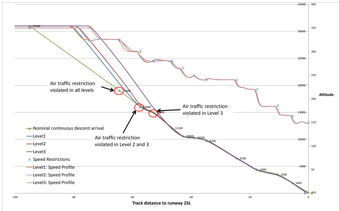
Figure 23 Vertical profile of three levels of the late descent scenario (SC1) with violated air traffic restrictions at each level highlighted
