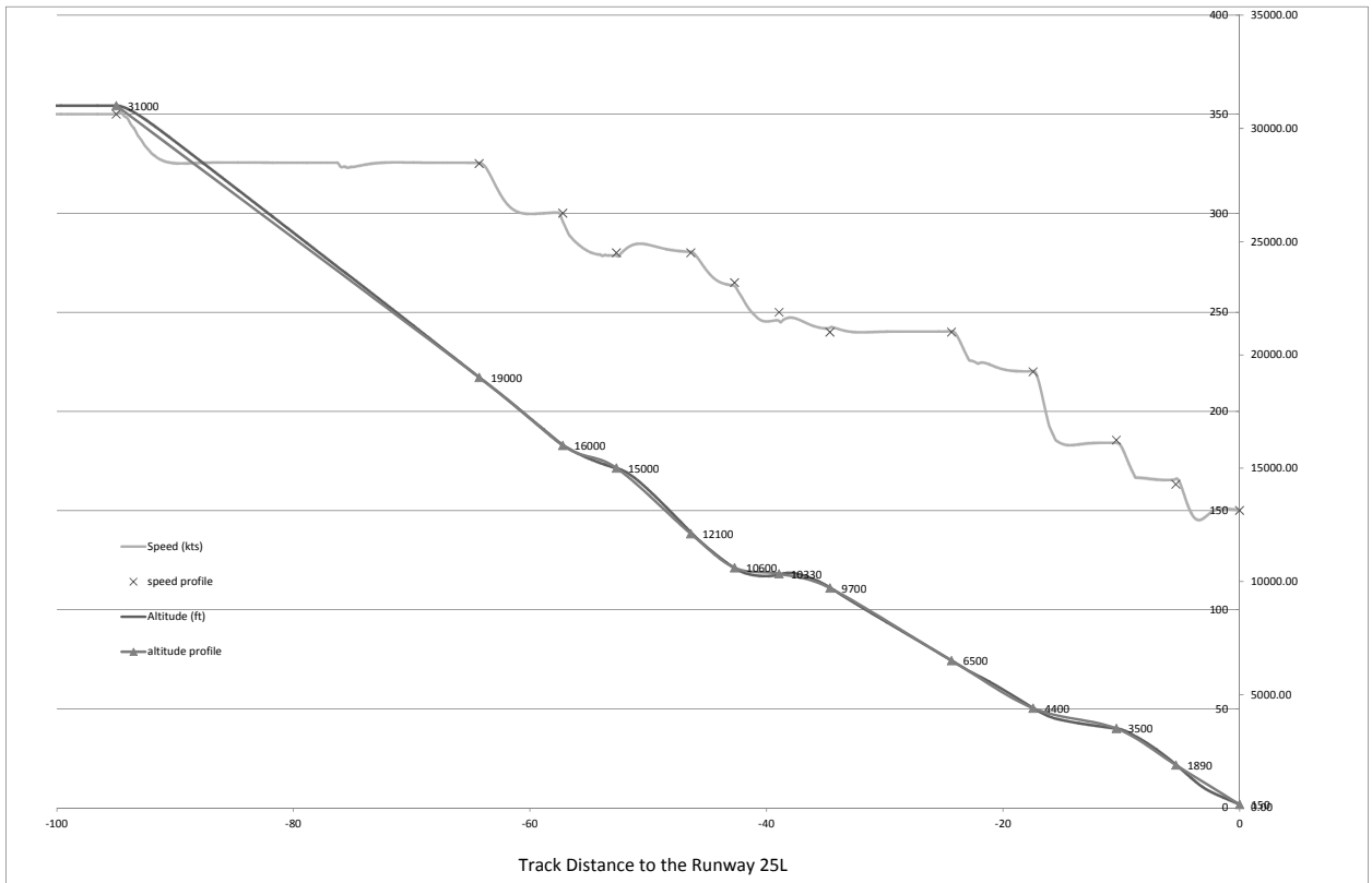
Figure 21 Vertical profile of a nominal (continuous descent) arrival and approach with associated altitude and airspeed restrictions of the STAR and the approach procedure
