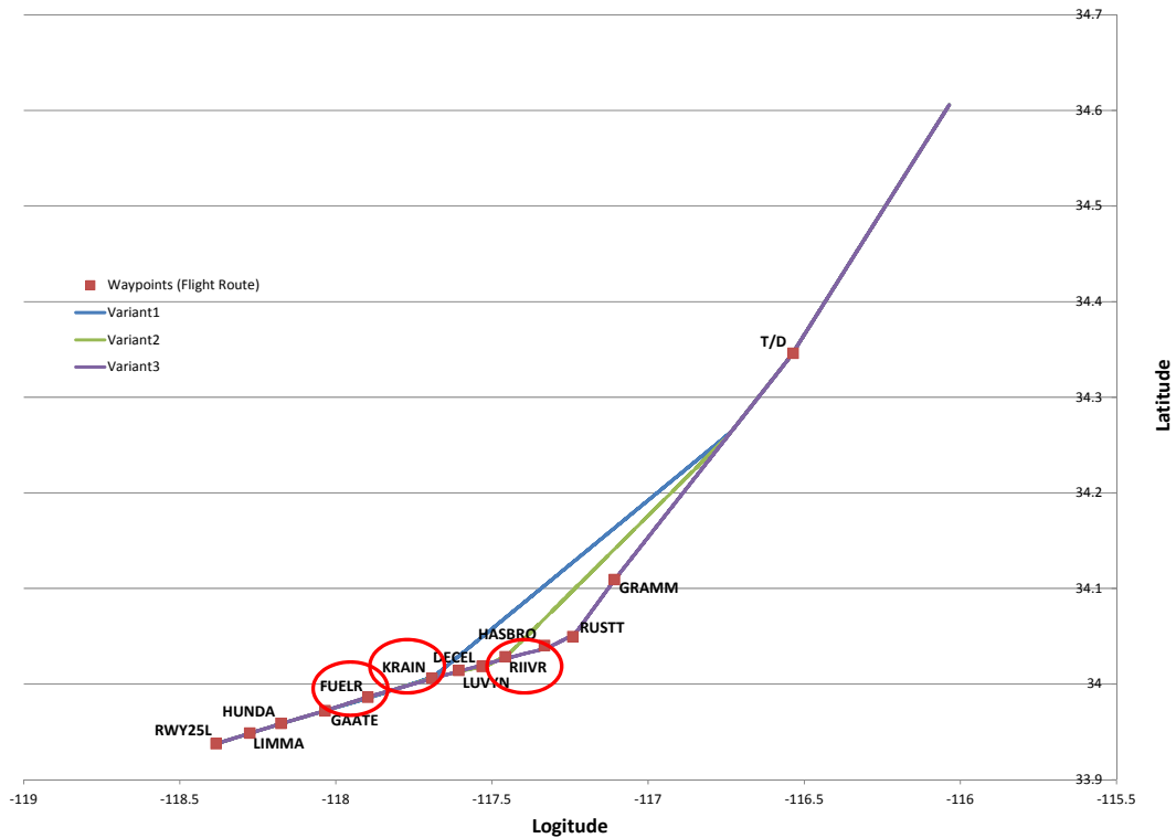
Figure 24 Lateral profile of three variants of the unpredicted re-routing scenario (SC2), re-routed waypoints for each variant highlighted
