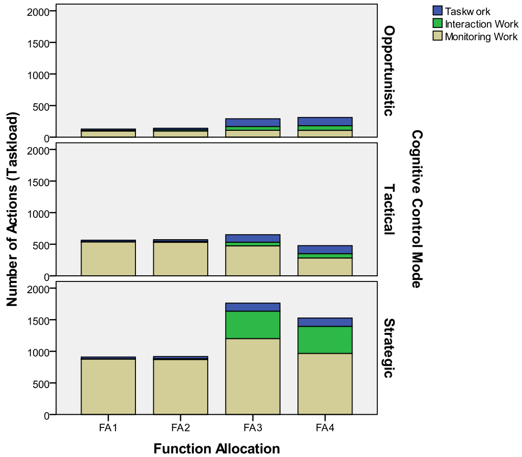
Figure 26 Number of actions (taskload) per simulated flight by function allocation and cognitive control mode averaged across all scenarios in cases with “Unlimited” maximum human taskload
