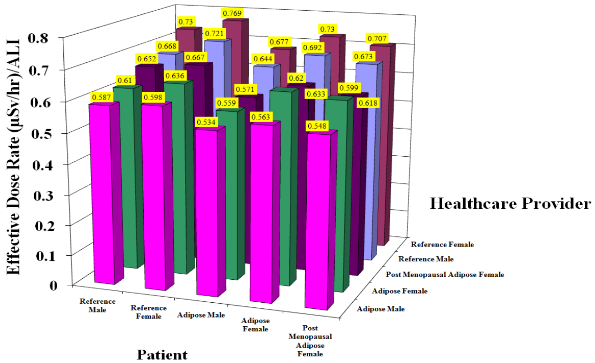
Figure 4.3 Effective Dose Rate to Healthcare Provider Due to 60 Co (moderate)
