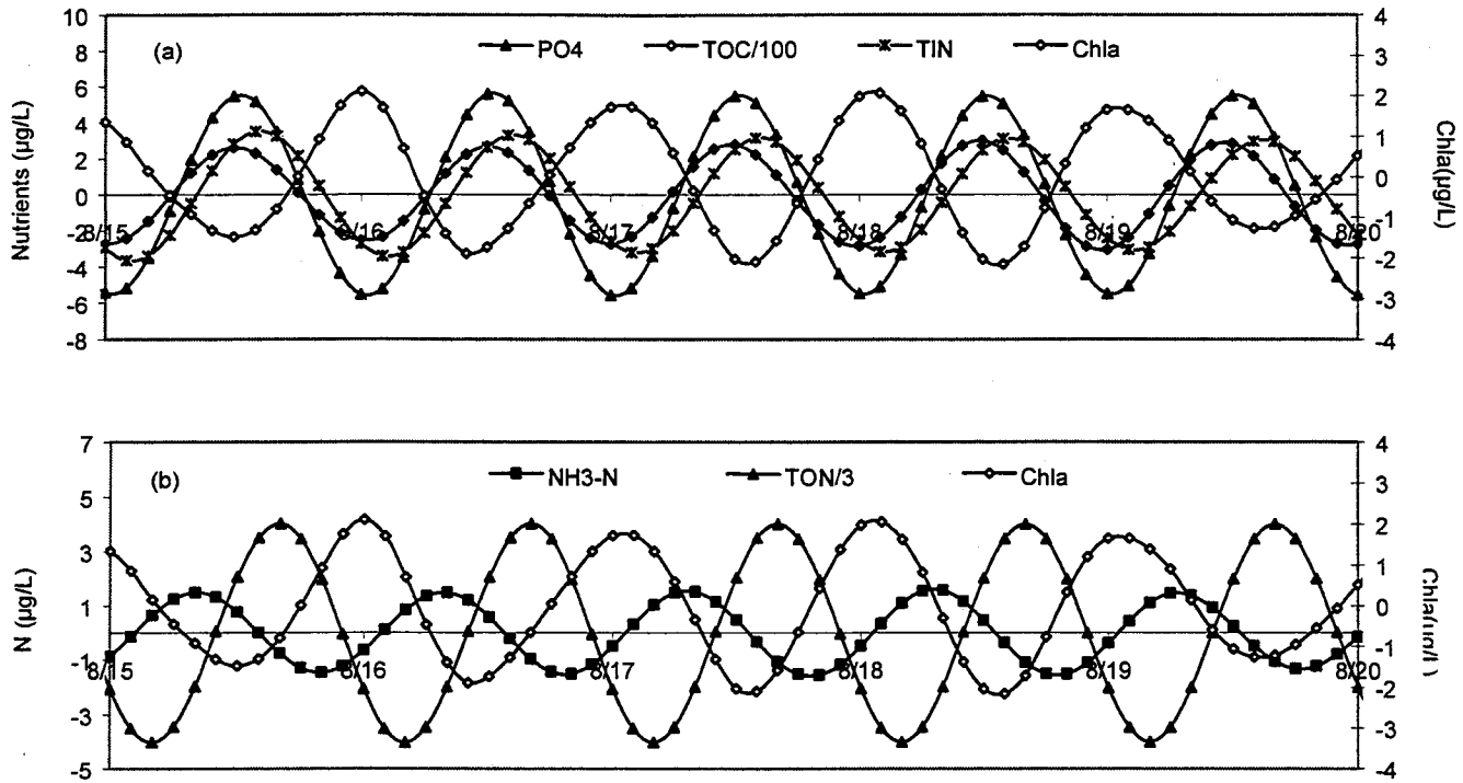
Figure 4. Phase lags between diurnal signals of chlorophyll- a and nutrients
