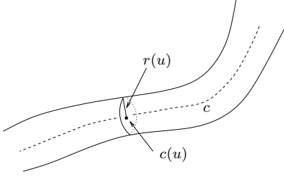
Fig. 1: Illustration of Tubular Surface model
