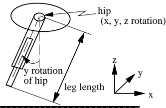
Figure 4: The reference angles for the degrees of freedom of the one-legged robot. The controlled degrees of freedom are the three degrees of freedom at the hip and the length of the leg.
