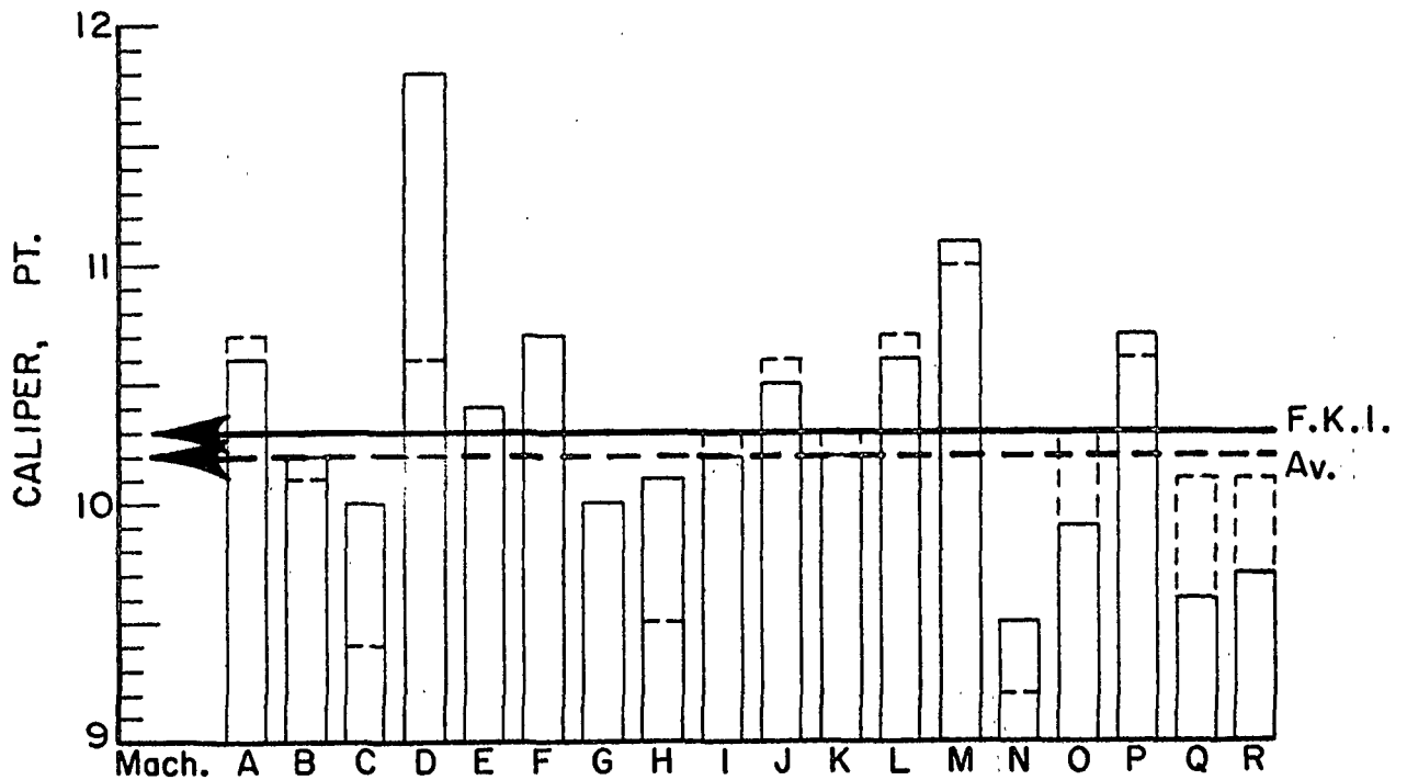
Figure 2. Comparison of Caliper Results for August, 1960
