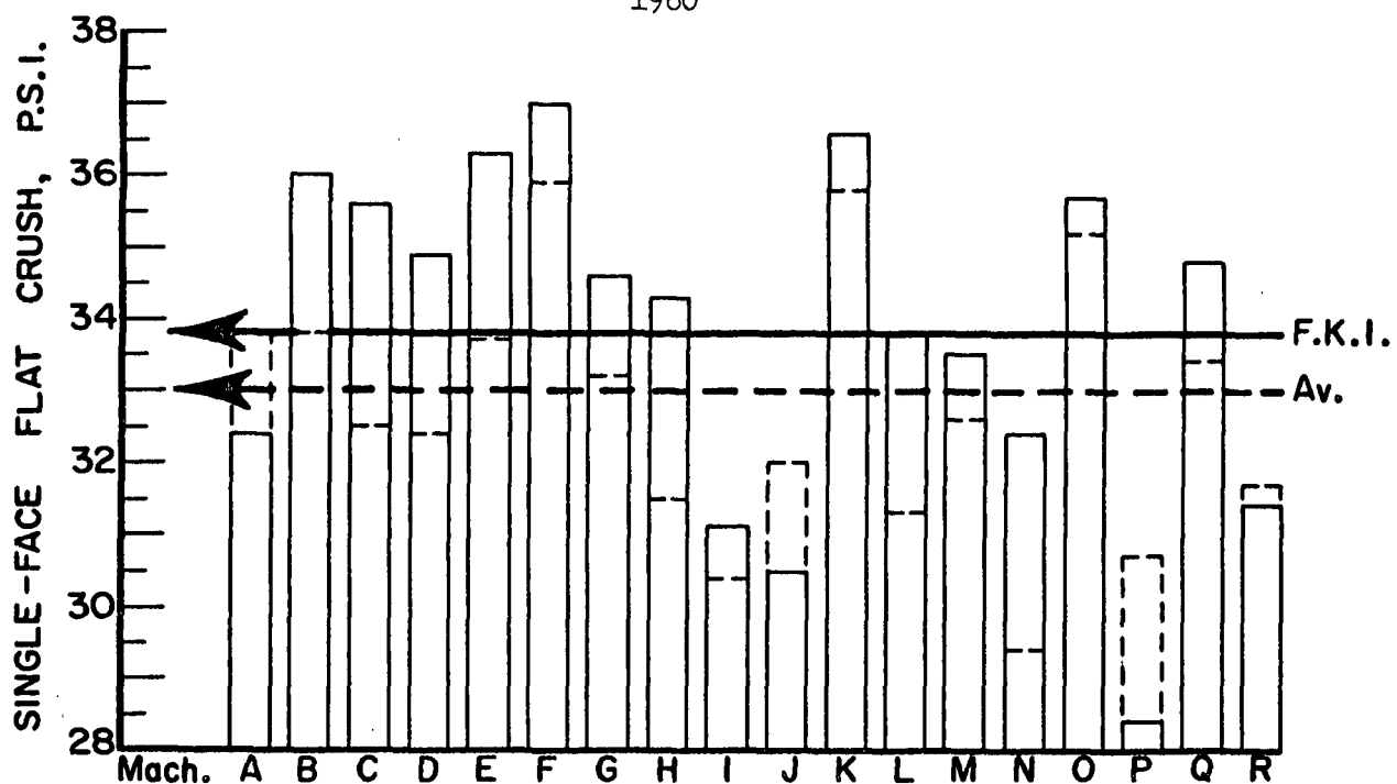
Figure 3. Comparison of Concora Flat Crush Results for August, 1960
