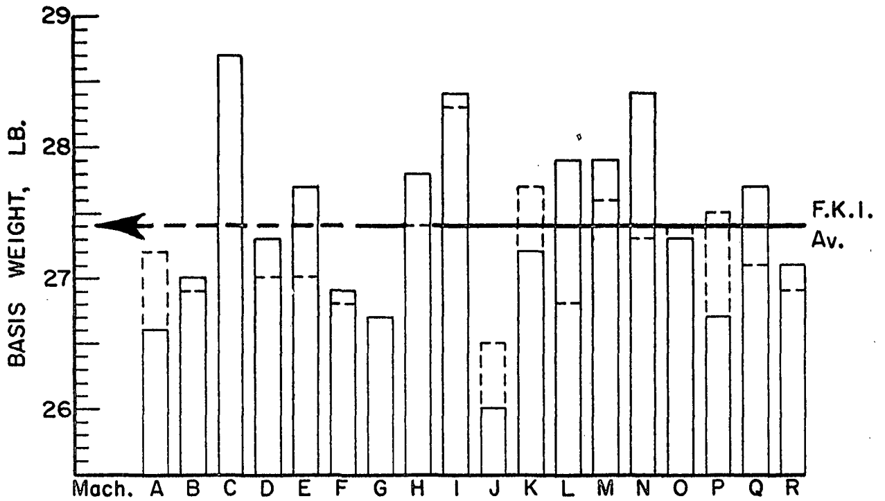
Figure 1. Comparison of Basis Weight Results for August, 1960
