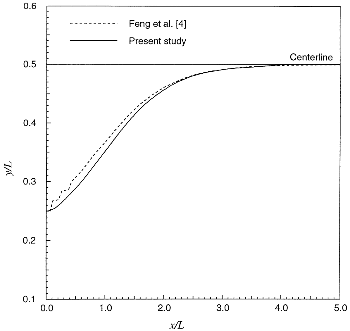
Fig. 4: Settling trajectories for particles with Reynolds number of 1.03 released from different initial positions in the narrow channel with the width of L . Comparison with the simulation result of Feng et al. [4] is also shown.
