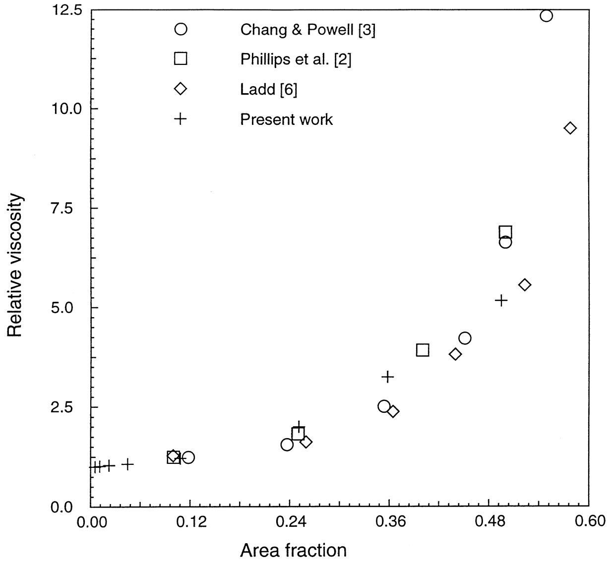
Fig. 6: Relative viscosity of 2-D suspensions in a Couette flow as a function of area ratio. The simulations are carried out for the system of 128 \times 128 and 512 \times 512 lattice nodes. The number of particles ranges from 16 to 64.
