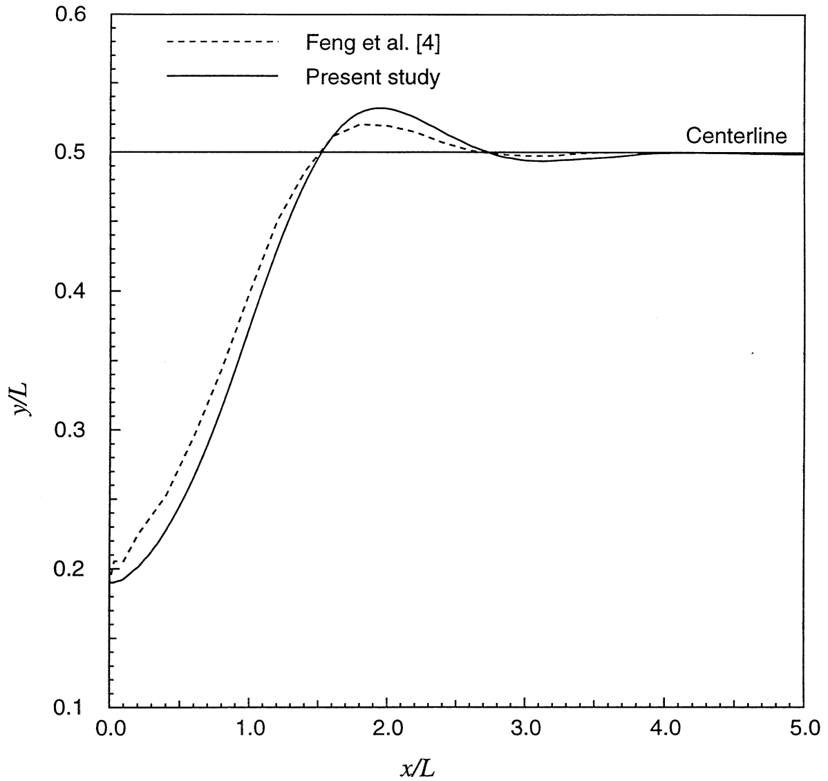
Fig. 5: Settling trajectories for particles with Reynolds number of 3.23 released from different initial positions in the narrow channel with the width of L . There is an overshoot across the centerline. Comparison with the simulation result of Feng et al. [4] is also shown.
