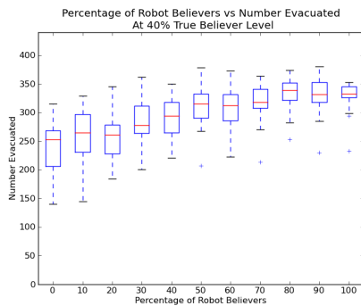
Fig. 6. Results of Robot to Human Tests at 40% True Believer Level
