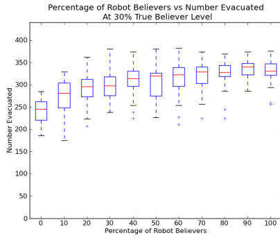
Fig. 5. Results of Robot to Human Tests at 30% True Believer Level
