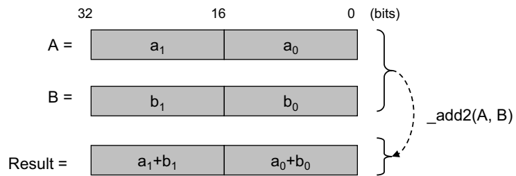
Figure 47: _add2 takes single cycle
