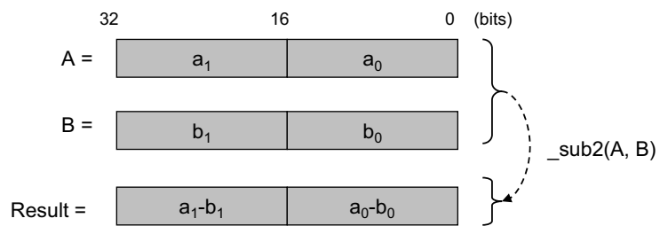
Figure 48: _sub2 takes single cycle
