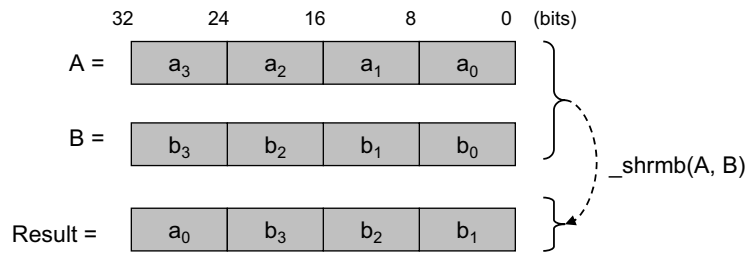
Figure 45: _shrmb takes single cycle
