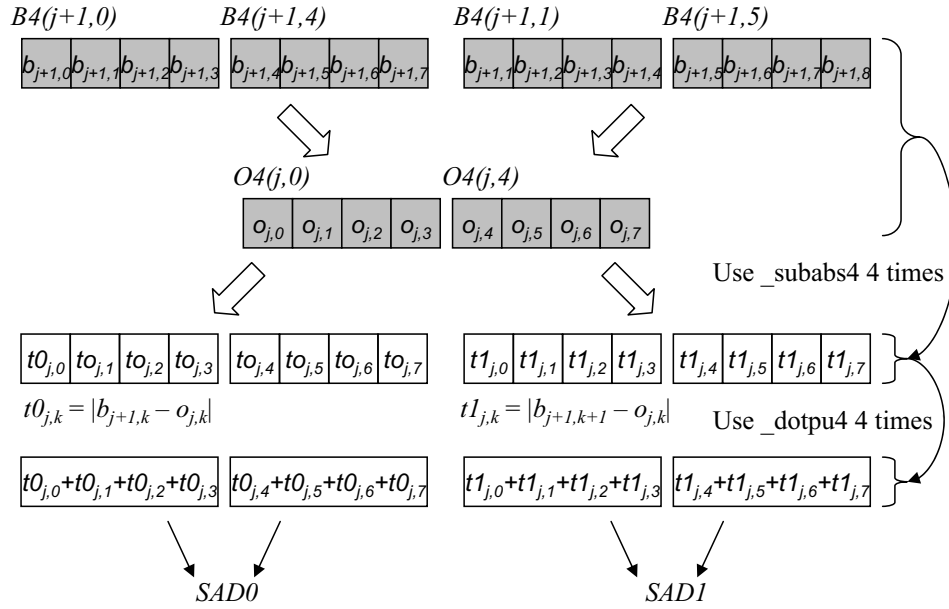
Figure 36: SAD calculation for the b-image
