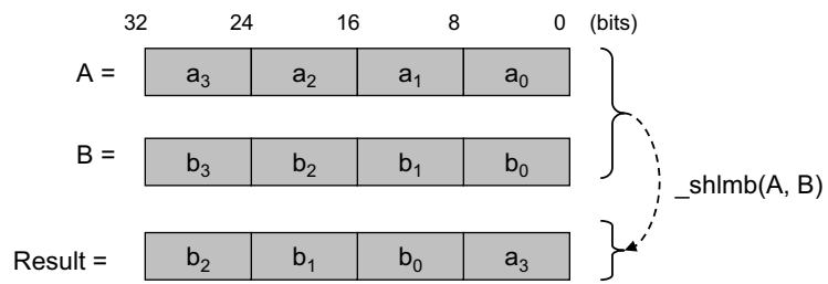
Figure 46: _shlmb takes single cycle
