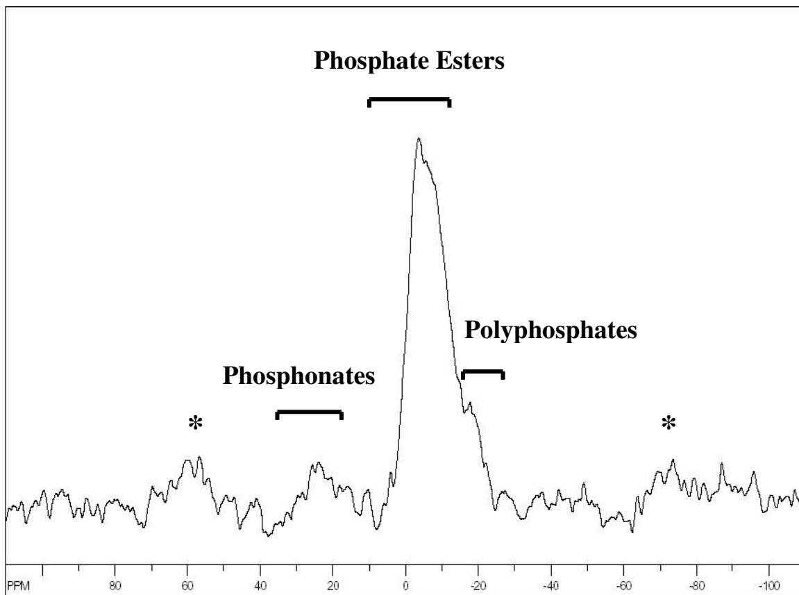
Figure 1 The ^{31}\text{P} NMR chemical shifts corresponding to different P compound classes, superimposed on the ^{31}\text{P} NMR spectrum of an Effingham Inlet sample taken at 78m. Asterisks denote spinning side bands
