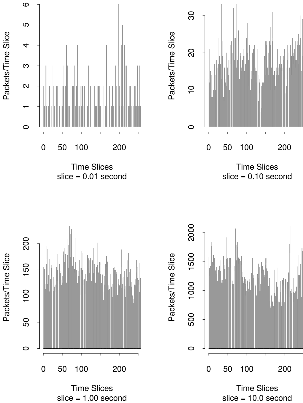
Figure 2: A section of traffic showing number of packets per time unit at four different time scales.
