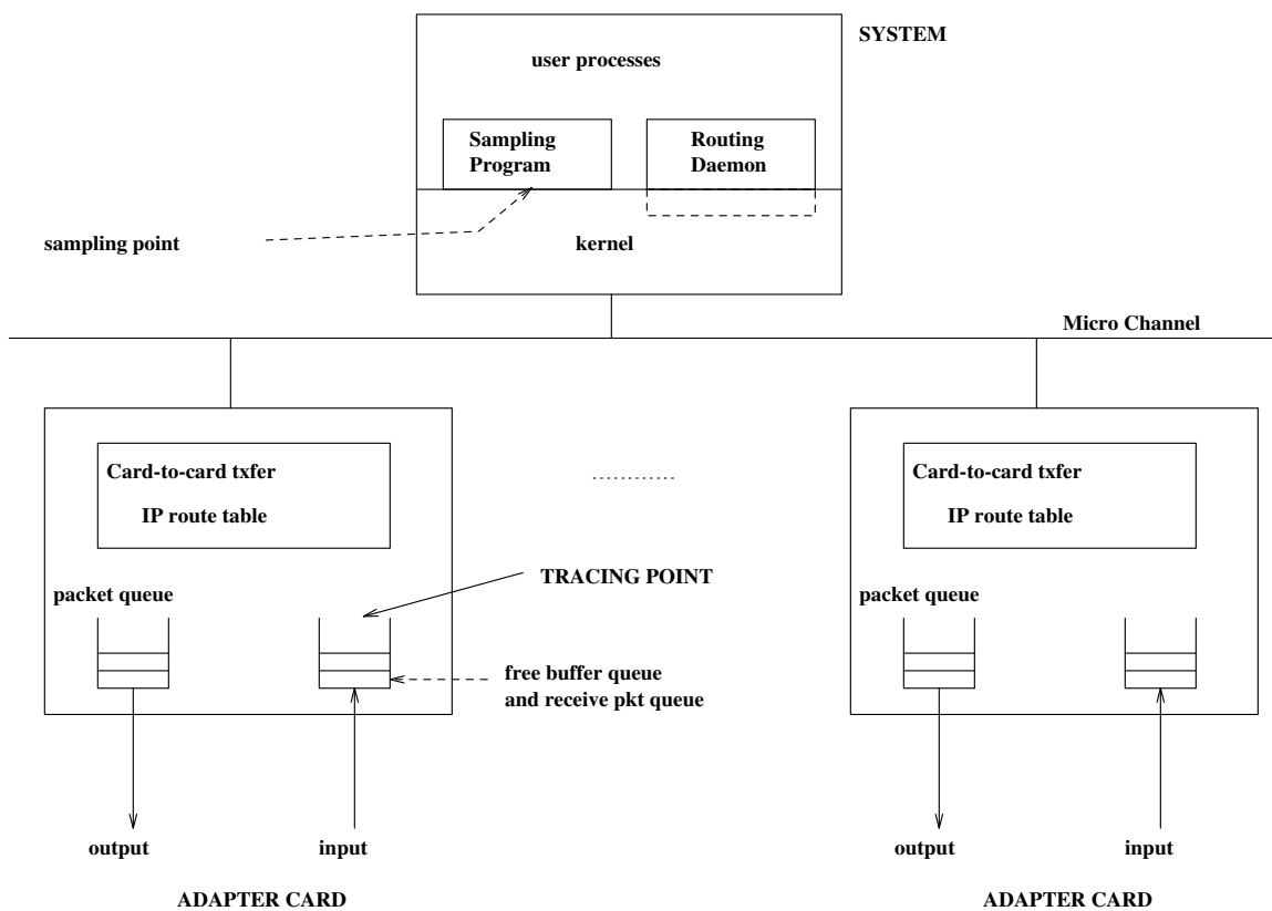
Figure 1: CNSS router architecture and trace points.
