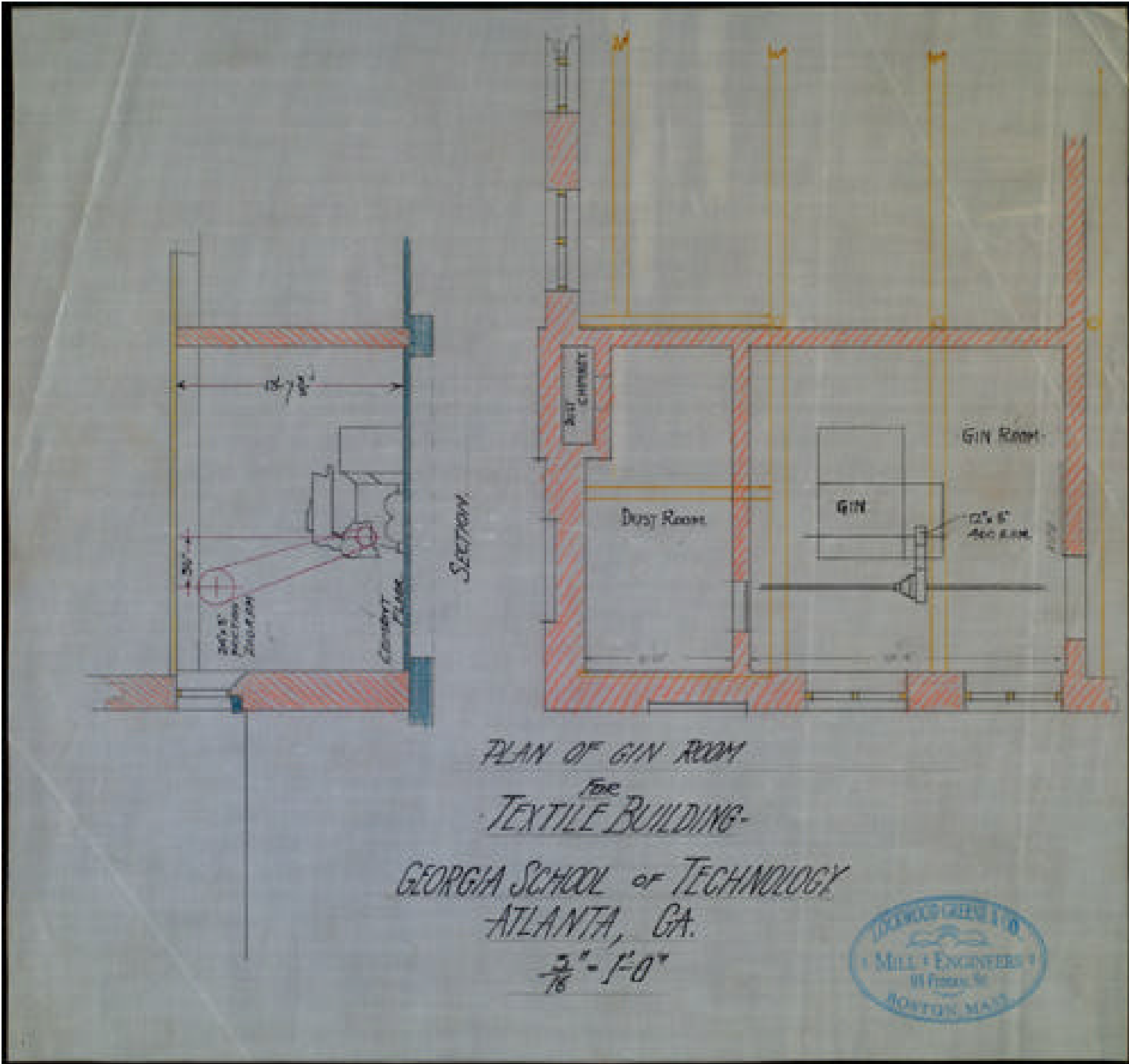
Sheet 24 - Gin room
