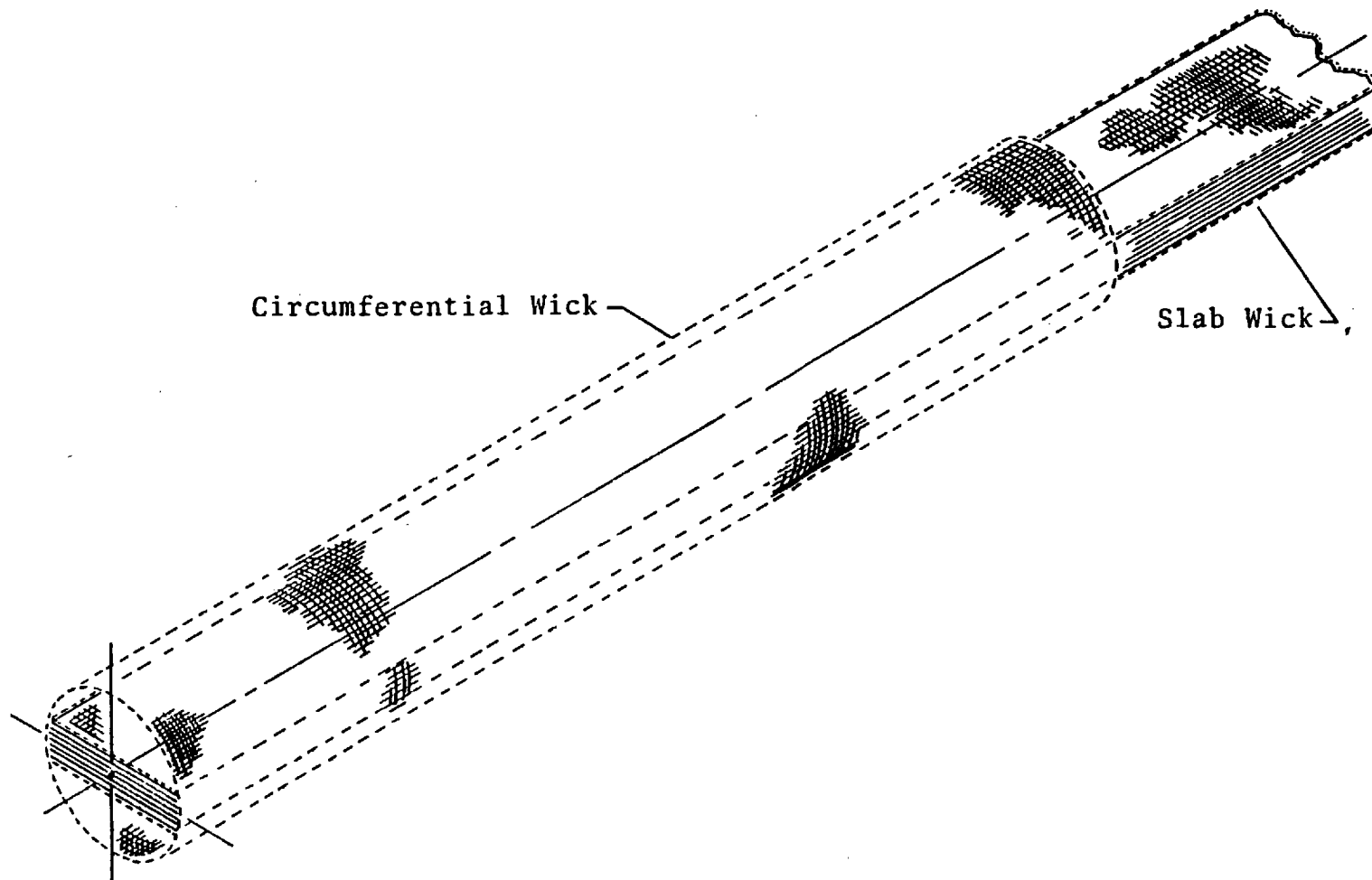
Figure 9. Close-Up of Composite Slab and Circumferential Wick at Heat Transfer Section
