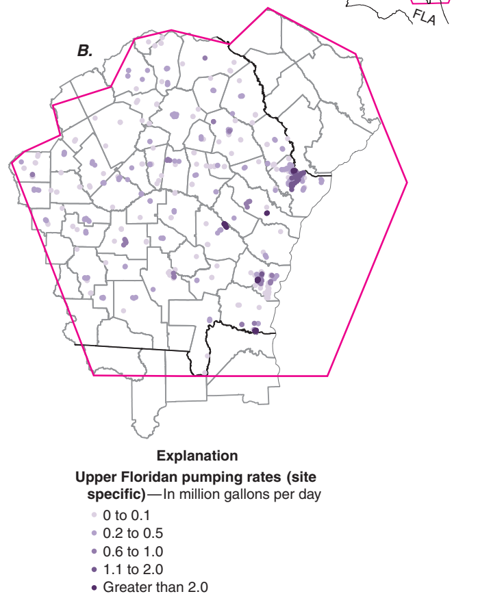
Figure 1. Geographic extent of regional ground-water flow models (A) model grid and boundary areas; (B) specific-site data; and (C) spatially distributed data.
