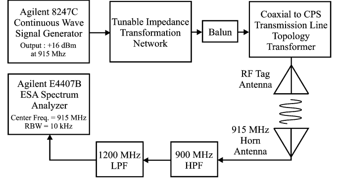
Fig. 1. The radio assay experimental setup for measurement of GP, the RF tag antenna gain penalty when attached to a material.
