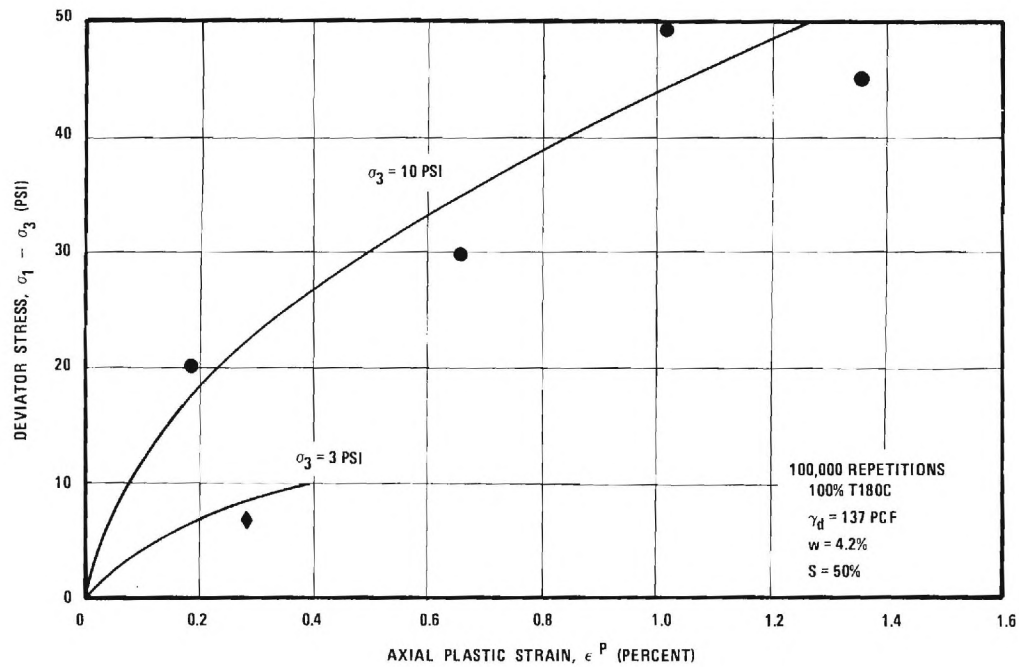
FIGURE 37. INFLUENCE OF DEVIATOR STRESS AND CONFINING PRESSURE ON PLASTIC STRAIN AFTER 100,000 REPETITIONS IN A CRUSHED BIOTITE GRANITE GNEISS WITH 3 PERCENT FINES-BASE 8
