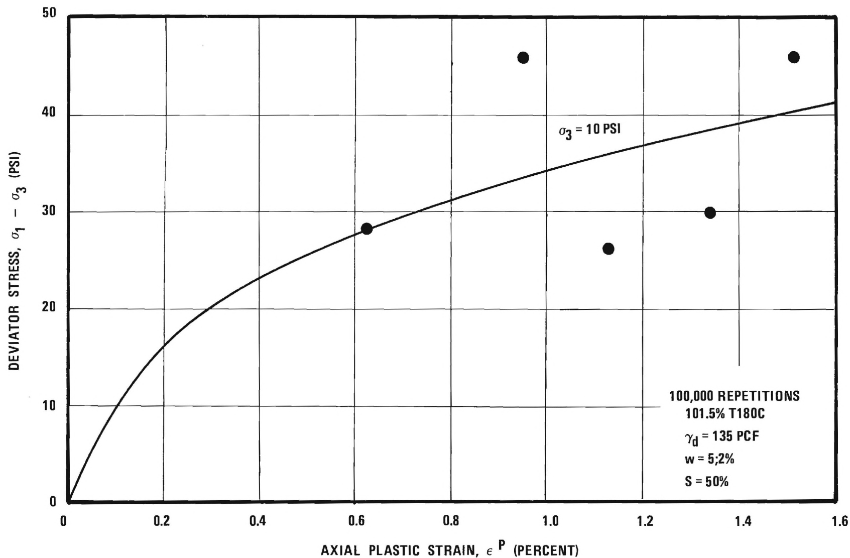
FIGURE 39. INFLUENCE OF DEVIATOR STRESS AND CONFINING PRESSURE ON PLASTIC STRAIN AFTER 100,000 REPETITIONS IN A CRUSHED BIOTITE GRANITE GNEISS WITH 22 PERCENT FINES-BASE 10
