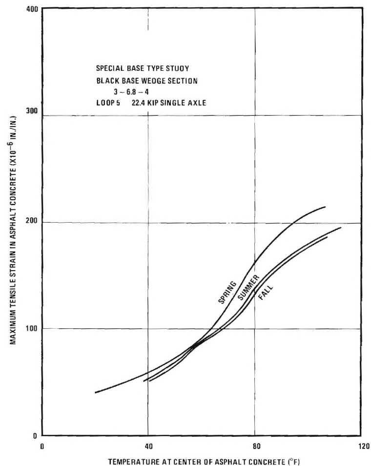
FIGURE 53. VARIATION OF MAXIMUM TENSILE STRAIN IN ASPHALT CONCRETE WITH TEMPERATURE AND SEASON.
