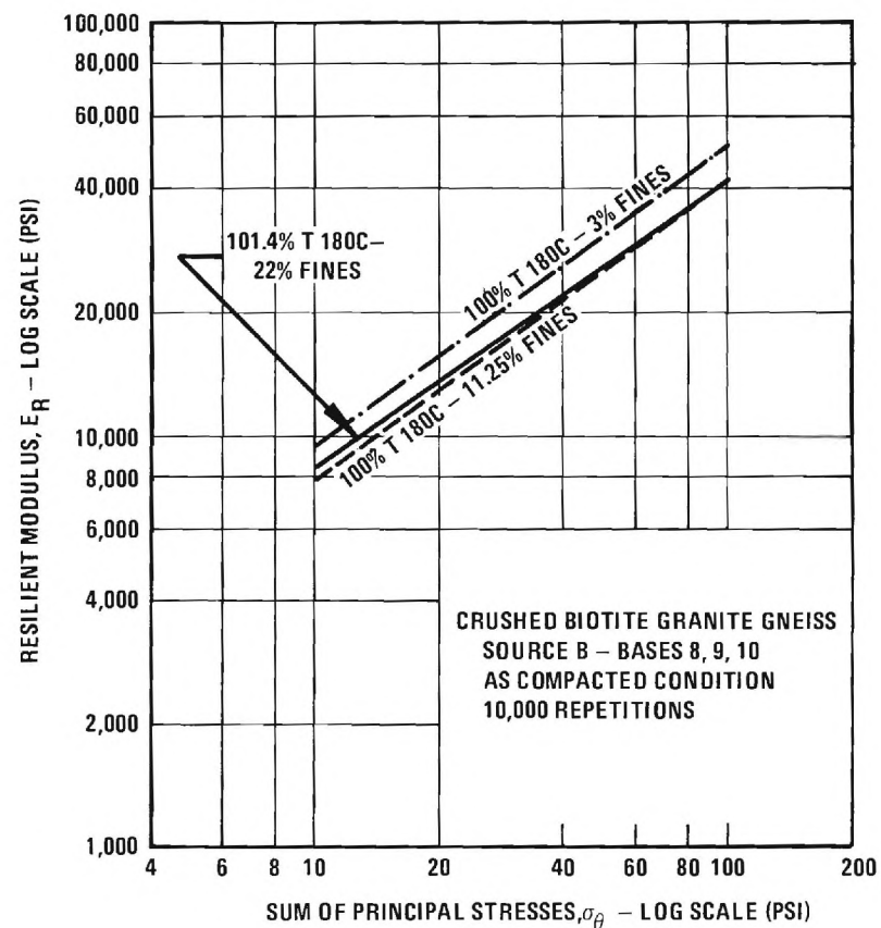
FIGURE 19. INFLUENCE OF FINES ON RESILIENT MODULUS FOR A CRUSHED BIOTITE GRANITE GNEISS
