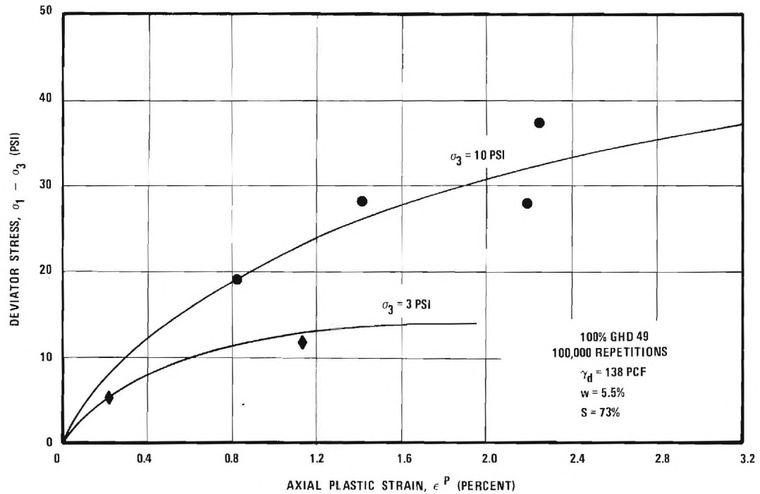
FIGURE 26. INFLUENCE OF DEVIATOR STRESS AND CONFINING PRESSURE ON PLASTIC STRAIN AFTER 100,000 REPETITIONS IN A 40-60 BLEND SOIL AGGREGATE-BASE 2
