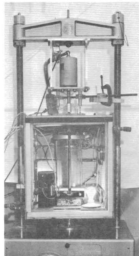
FIGURE 3(B). TEST SET-UP FOR ASPHALT
