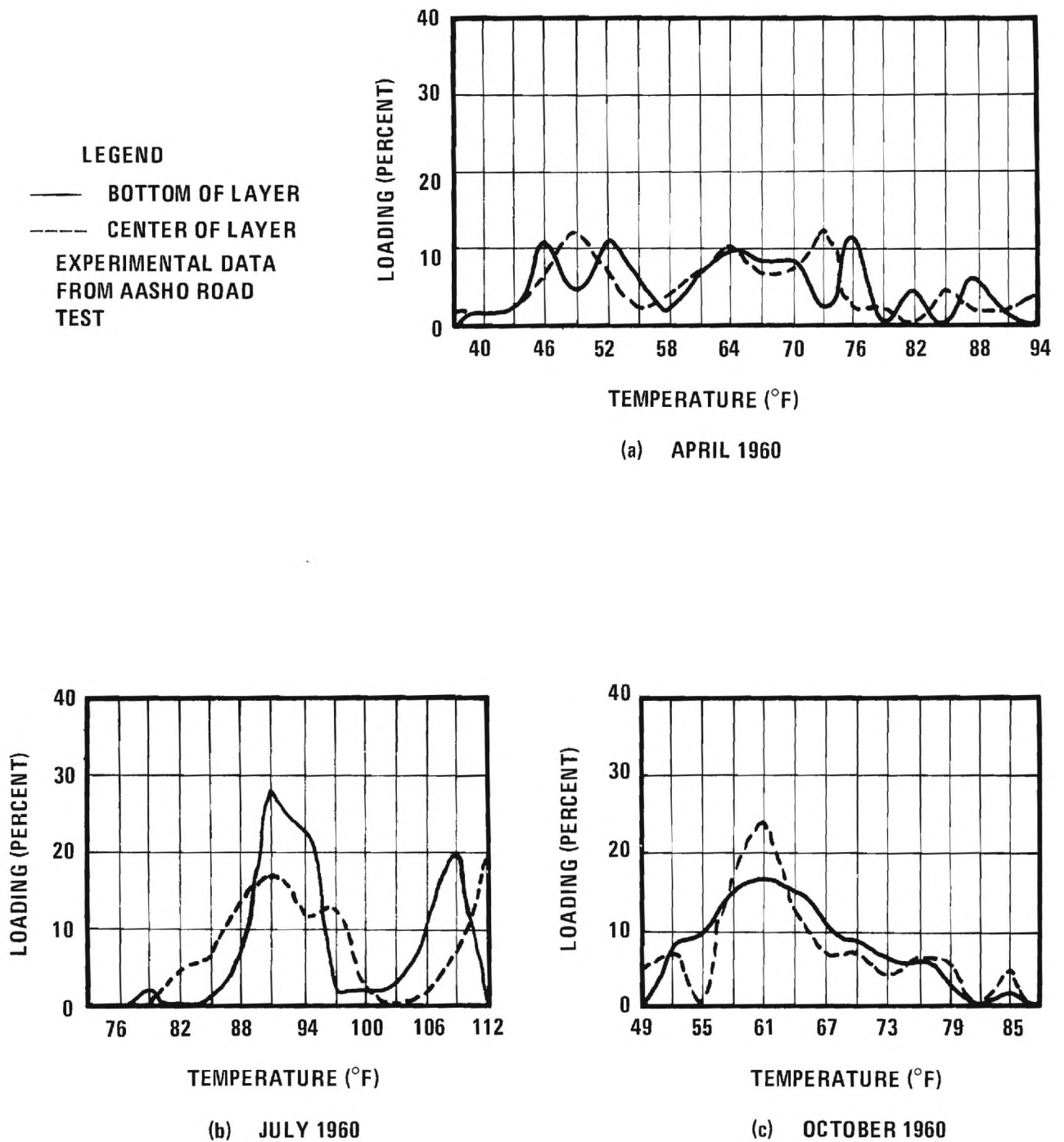
FIGURE 49. RELATIONSHIP BETWEEN APPLIED LOADING AND TEMPERATURE IN THE ASPHALT CONCRETE FOR THREE SELECTED MONTHS- EXPERIMENTAL DATA FROM THE AASHO ROAD TEST
