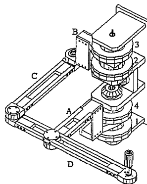
Fig. 1. Passive Trajectory Enhancing Robot (PTER)
