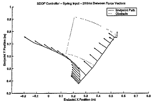
Fig. 7. SDOF Control; 4 SDOF Obstacle; Low Penetration Speed
