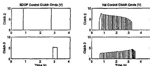
Fig. 13. Clutch Commands
