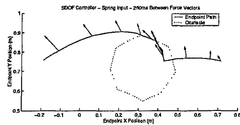
Fig. 9. SDOF Control; 8 SDOF Obstacle; High Penetration Speed
