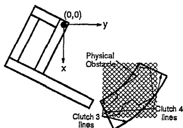
Fig. 4. An Obstacle Defined for use with the SDOF Controller
