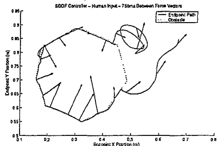
Fig. 14. Performance of Controllers with Human Input
