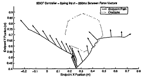
Fig. 10. SDOF Control; 8 SDOF Obstacle; High Penetration Speed
