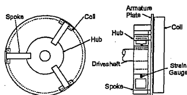
Fig. 2. Torque Sensing Clutch — Schematic
