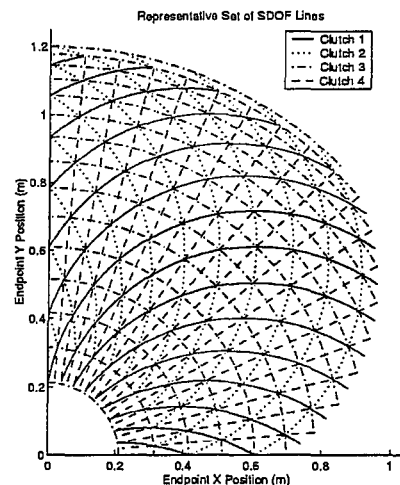
Fig. 5. Set of SDOF Lines
