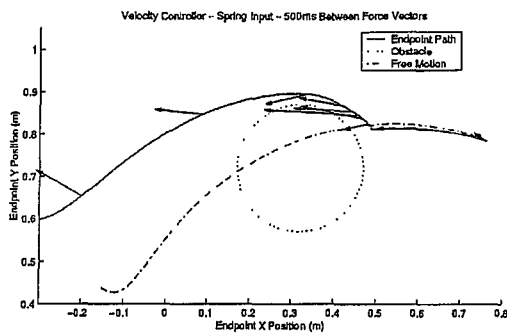
Fig. 11. Velocity Control; Path Redirection
