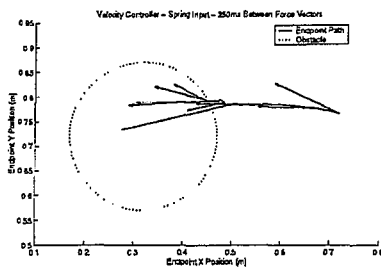
Fig. 8. Velocity Controller; Tip Locking Condition
