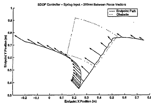
Fig. 6. SDOF Control; 4 SDOF Obstacle; High Penetration Speed
