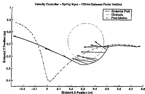
Fig. 12. Velocity Control; Path Redirection
