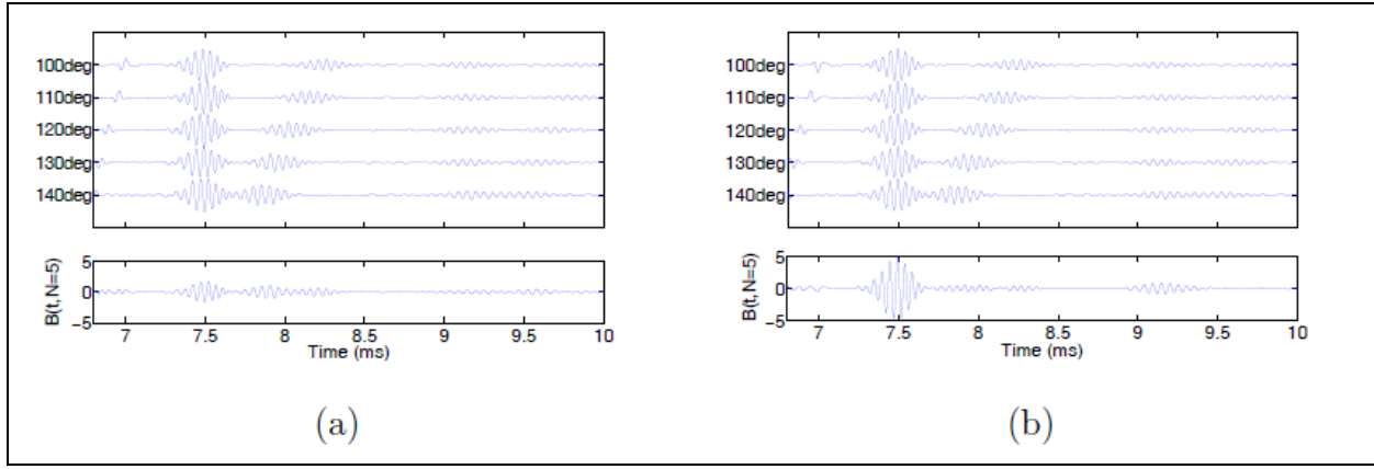
FIG. 5. (a) Upper Panel: Stacked representation of the time-aligned arrivals of counter-clockwise propagating A0 waves recorded at five different bistatic angles. The relative bistatic time-shifts, with respect to first bistatic angle \theta = 100\text{deg} were obtained from the SPWV analysis (see Fig. 4). Lower Panel: Coherent addition of the five time-shifted waveforms using a conventional time-delay beamformer (i.e. when setting the companding parameter as j = 1 - see Eq. 8). (b) Upper Panel: same as (a), but each waveform was also companded to account for the apparent frequency shift of the bistatic counter-clockwise propagating A0 arrival with respect to the first bistatic angle \theta = 100\text{deg} -based on the measured frequency-shifts values from the SPWV analysis (see Fig. 4). Lower Panel: Coherent addition of the five time-frequency shifted waveforms using a generalized time-frequency beamformer. Note that each bistatic waveform, in both upper panels, was normalized to its maximum, such that one would expect a maximum beamformer output of 5 when an optimal coherent addition of these waveforms is achieved.
