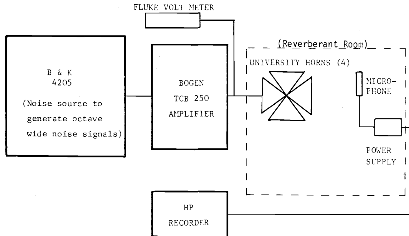
FIGURE 5.2 EQUIPMENT ARRANGEMENT
