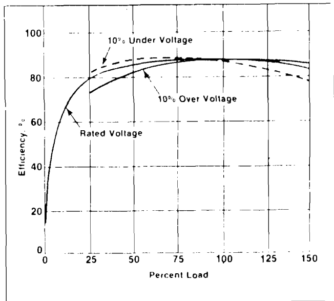
Fig 1.3 Efficiency Sensitivity
