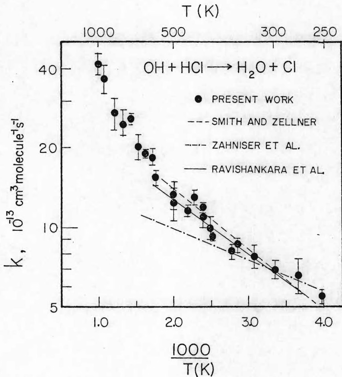
Figure 2. Plot of \ln k_2 vs. \frac{1000}{T} .
