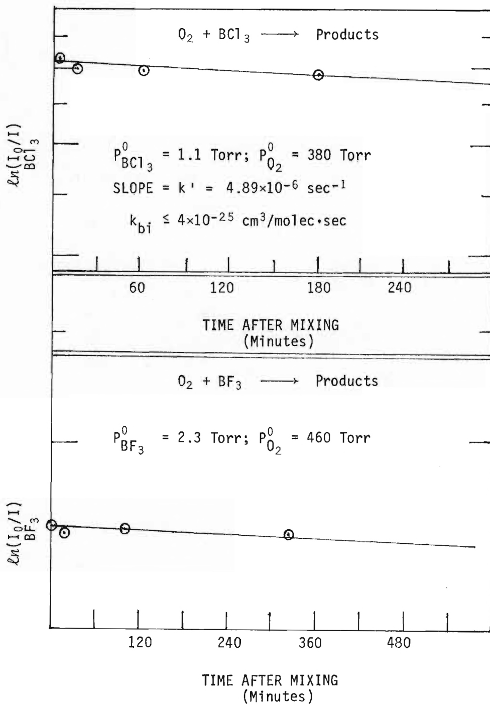
Figure 6. Time-Resolved Infrared Spectroscopy
