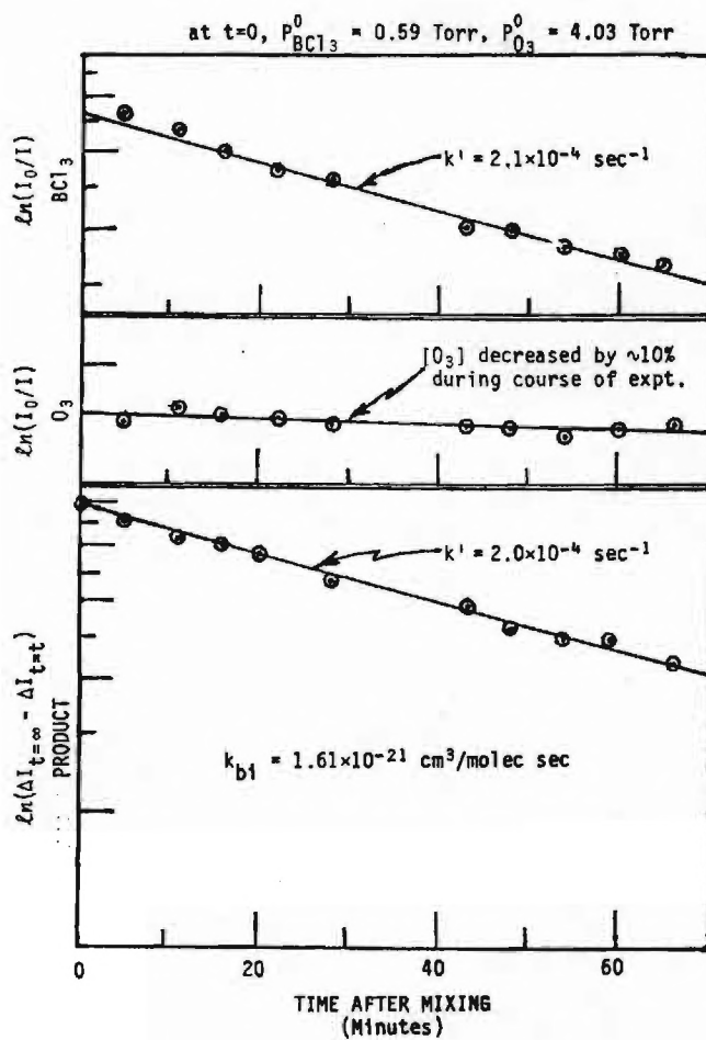
Figure 7a. Time-Resolved Infrared Spectroscopy
