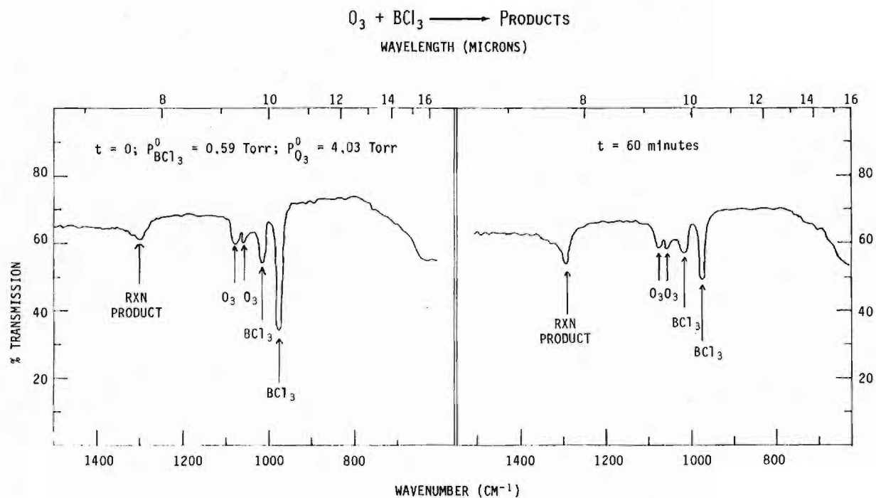
Figure 7a. Time-Resolved Infrared Spectroscopy
