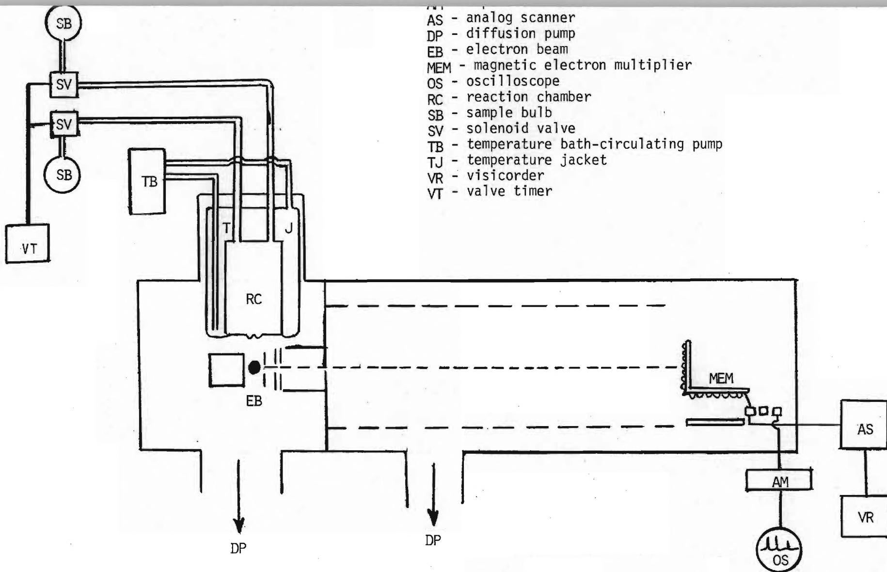
FIGURE 5 - STOP-FLOW TOF MASS SPECTROMETER SYSTEM
