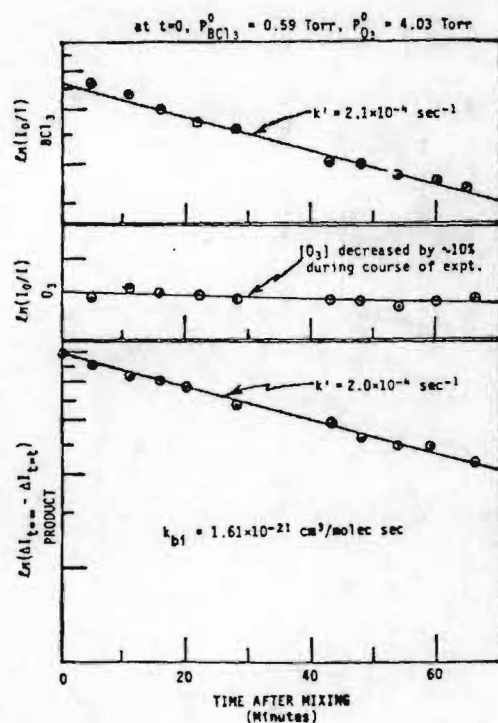
Figure 3b. First Order Decay Plot for the Disappearance of BCl_3 and Appearance of Reaction Product in the Reaction of BCl_3 with O_3 \cdot [O_3] > [BCl_3] .
