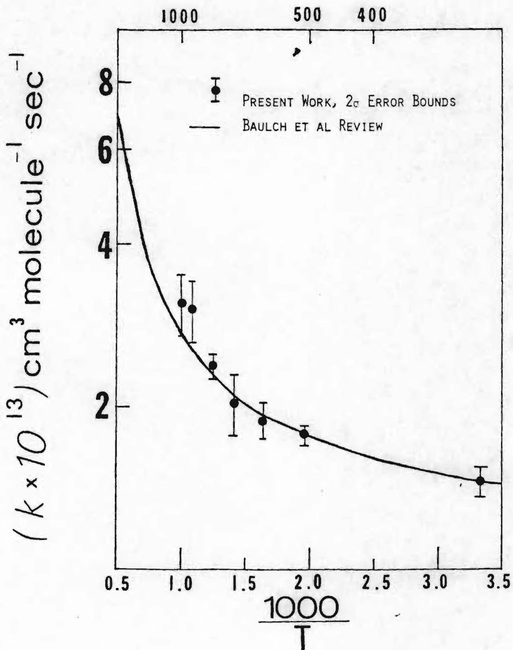
Figure 1. Plot of \ln k_1 vs. \frac{1000}{T} .
