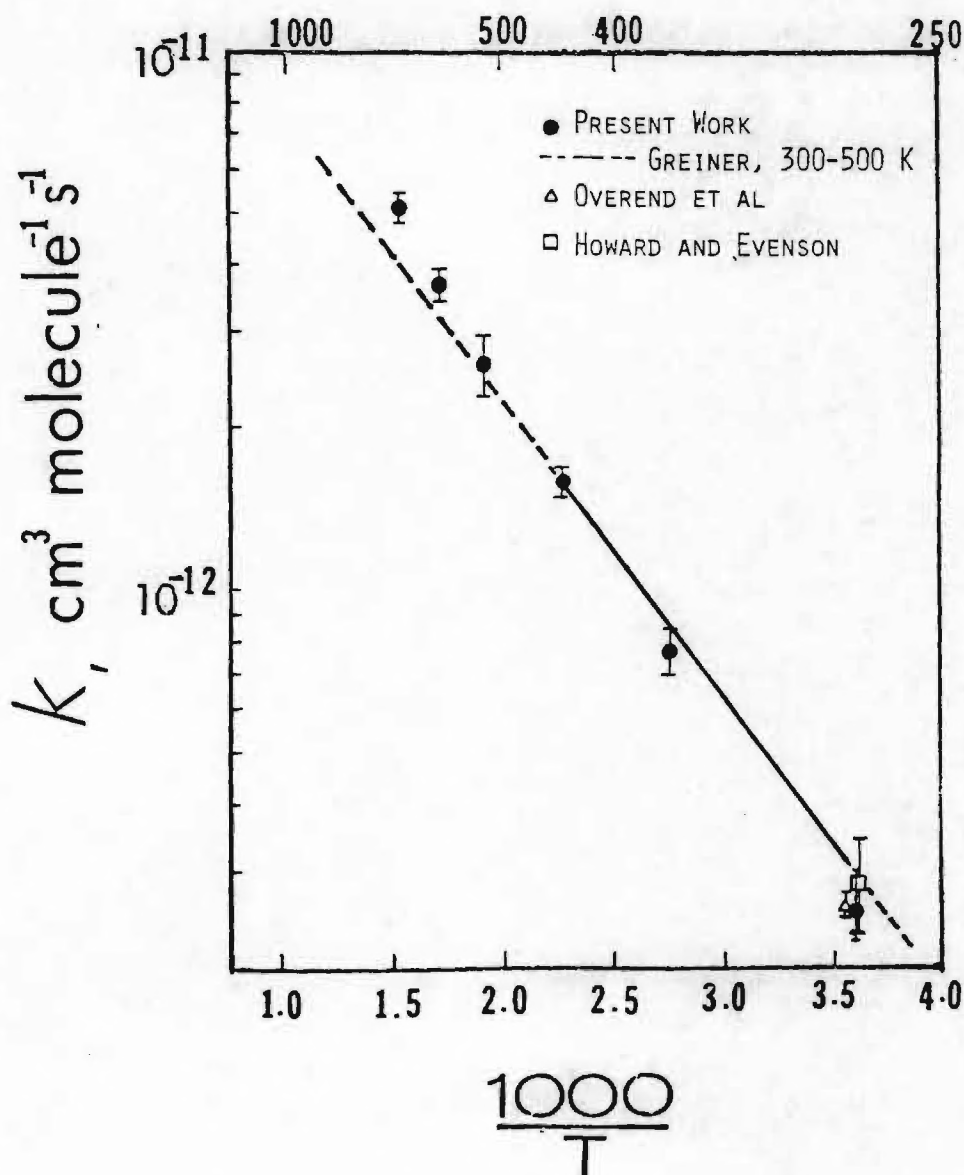
Figure 3. Plot of \ln k_3 vs. \frac{1000}{T} .
