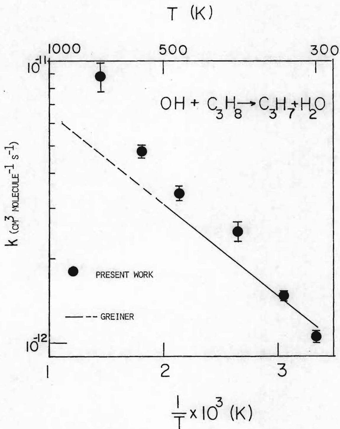
Figure 4. Plot of \ln k_4 vs. \frac{1000}{T} .
