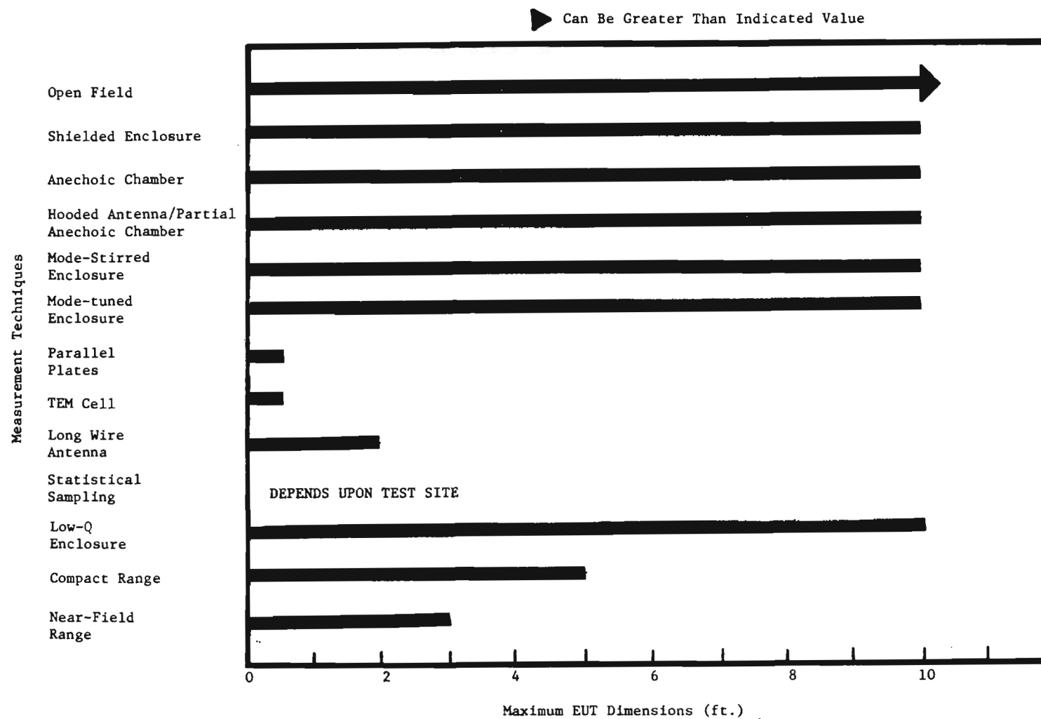
Figure 12. Maximum Dimension of the EUT for Various Measurement Techniques.
