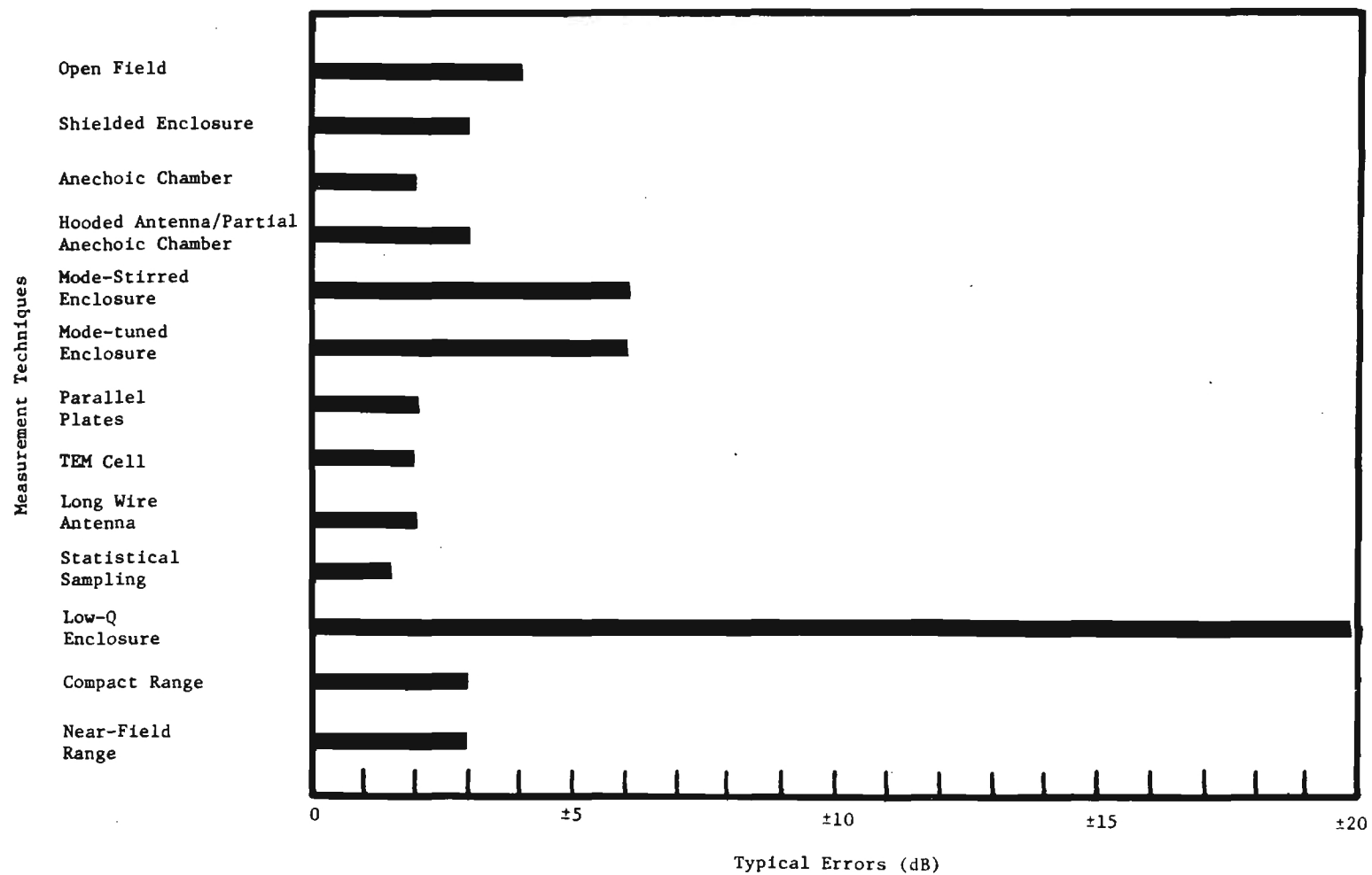
Figure 11. Range of Errors Typically Encountered for Various Measurement Techniques.
