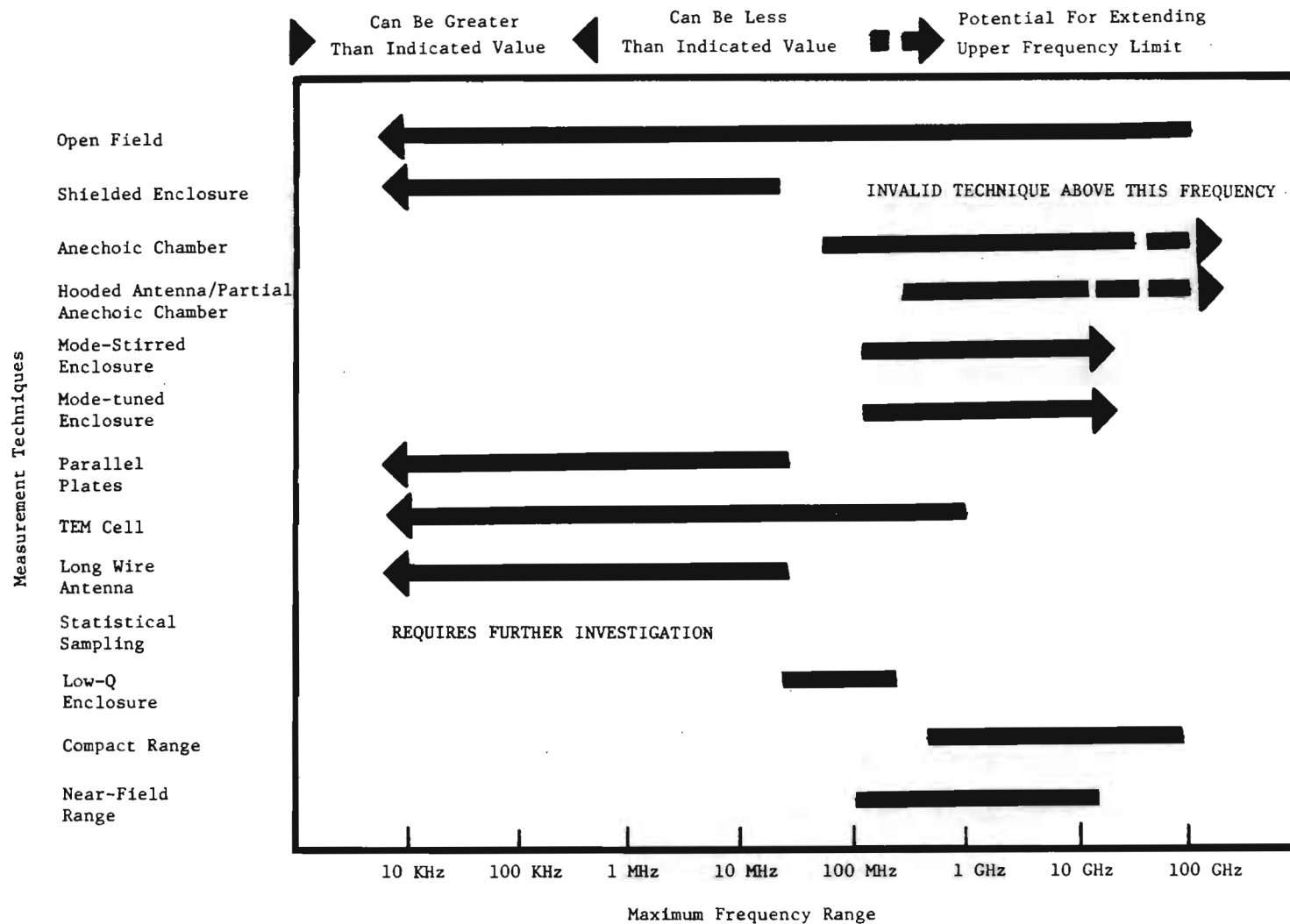
Figure 13. Comparison of Maximum Frequency Range for Various Measurement Techniques.
