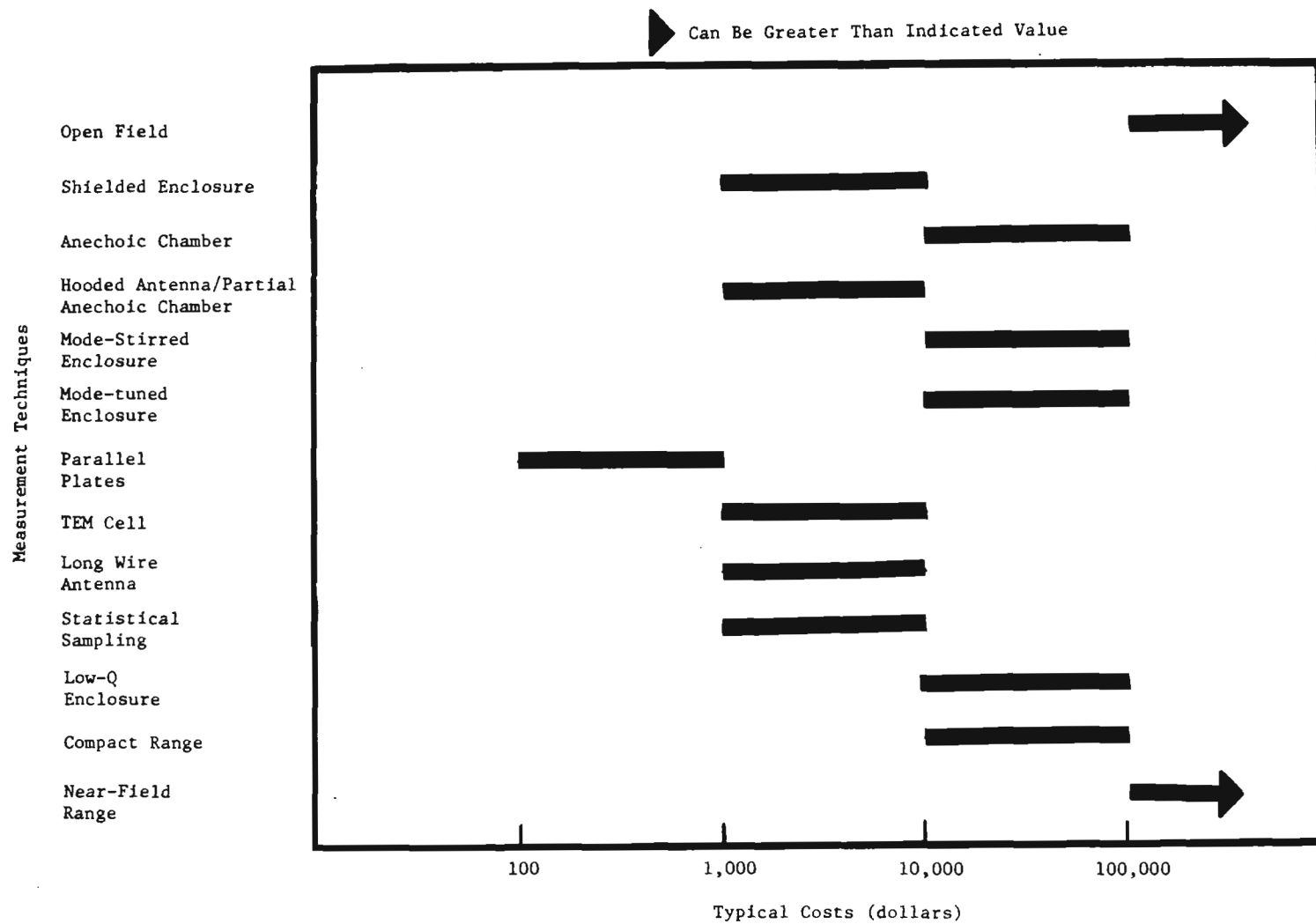
Figure 16. Comparison of Typical Costs for Various Measurement Techniques.
