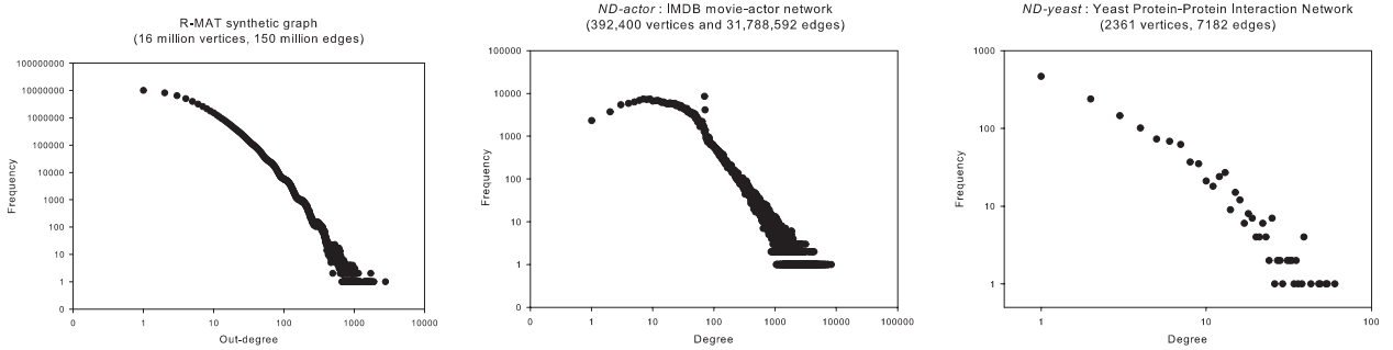
Figure 1: Degree distributions of some network instances
