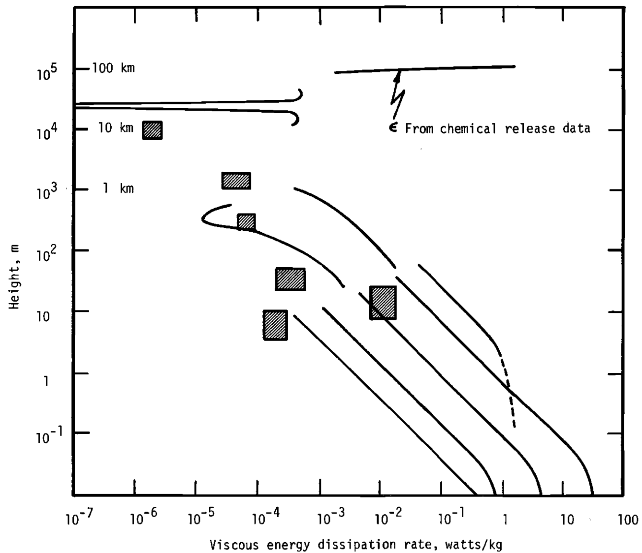
Figure 5. Summary of Viscous Energy Dissipation Rate Determinations from Altitudes of One cm to 110 km.
