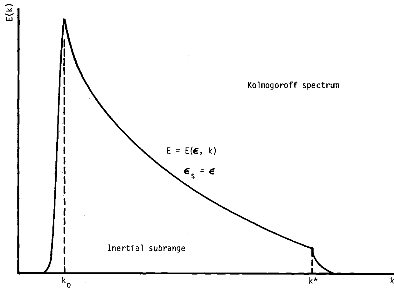
Figure 7a. Schematic Graph of the Energy Spectrum Function for Kolmogoroff Type Homogeneous Turbulence.
