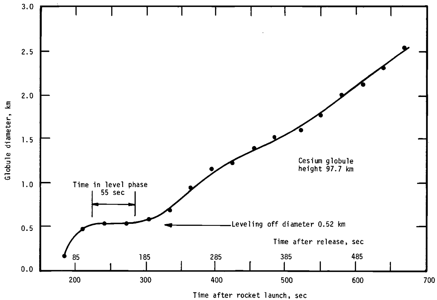
Figure 2. Sample Globule Growth Curve - Diameter versus Time after Rocket Launch.
