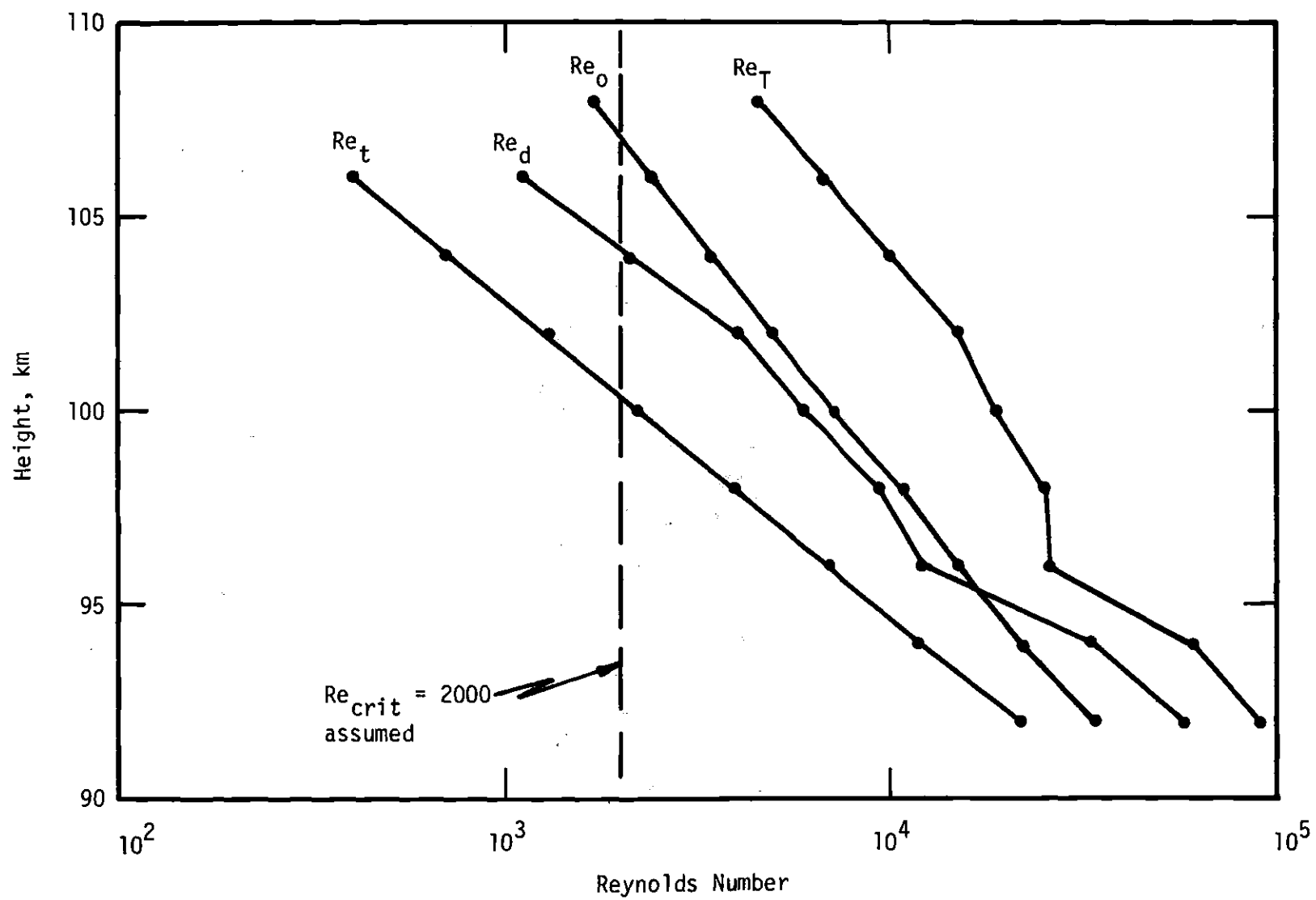
Figure 17. Calculated Reynolds Numbers versus Altitude.
