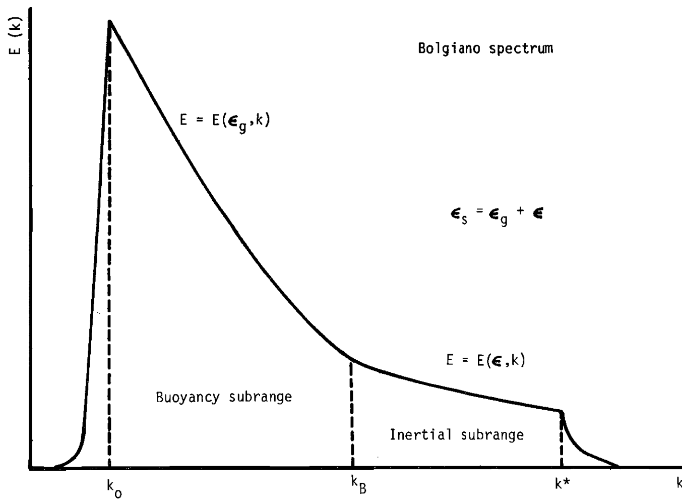
Figure 7b. Schematic Graph of the Energy Spectrum Function for Bolgiano Type Buoyancy Turbulence.
