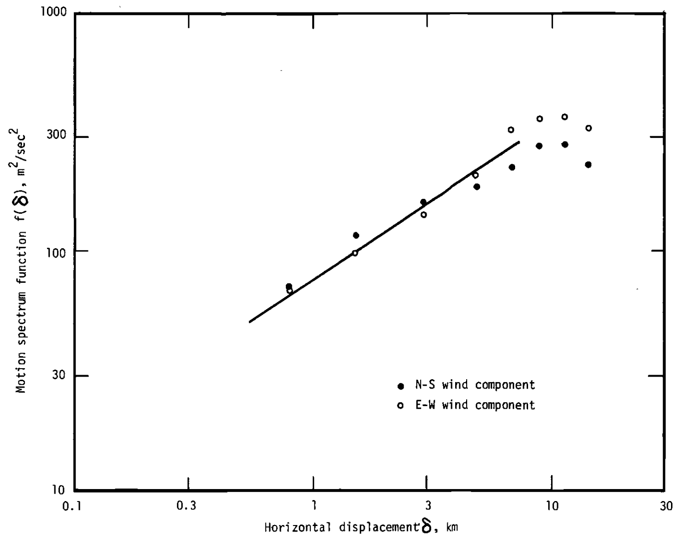
Figure 10. Average Horizontal Motion Spectrum of the Turbulent Winds.
