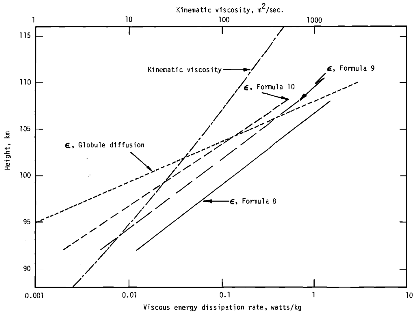
Figure 1. Viscous Dissipation Parameter \epsilon and the Kinematic Viscosity \eta versus Altitude.
