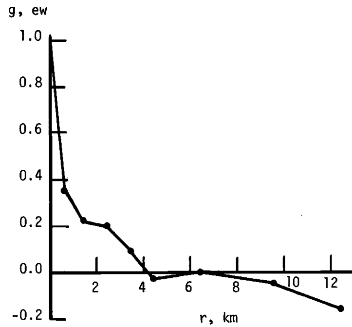
Figure 16. Spatial Correlation Function for North-South and East-West Turbulent Wind Components versus Horizontal Spatial Displacement.
