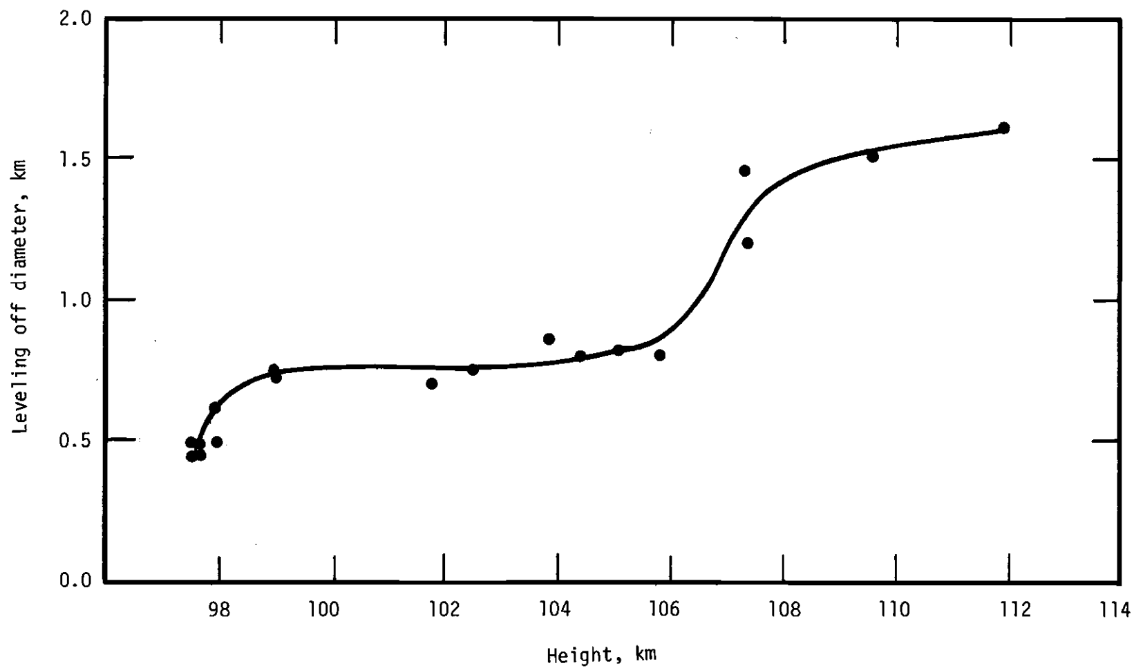
Figure 3. Height Variation of the Globule Leveling off Diameter.
