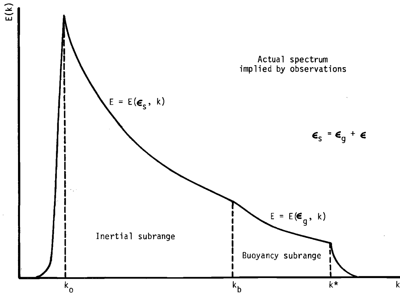
Figure 7c. Schematic Graph of the Energy Spectrum Function for the Observed Turbulence.
