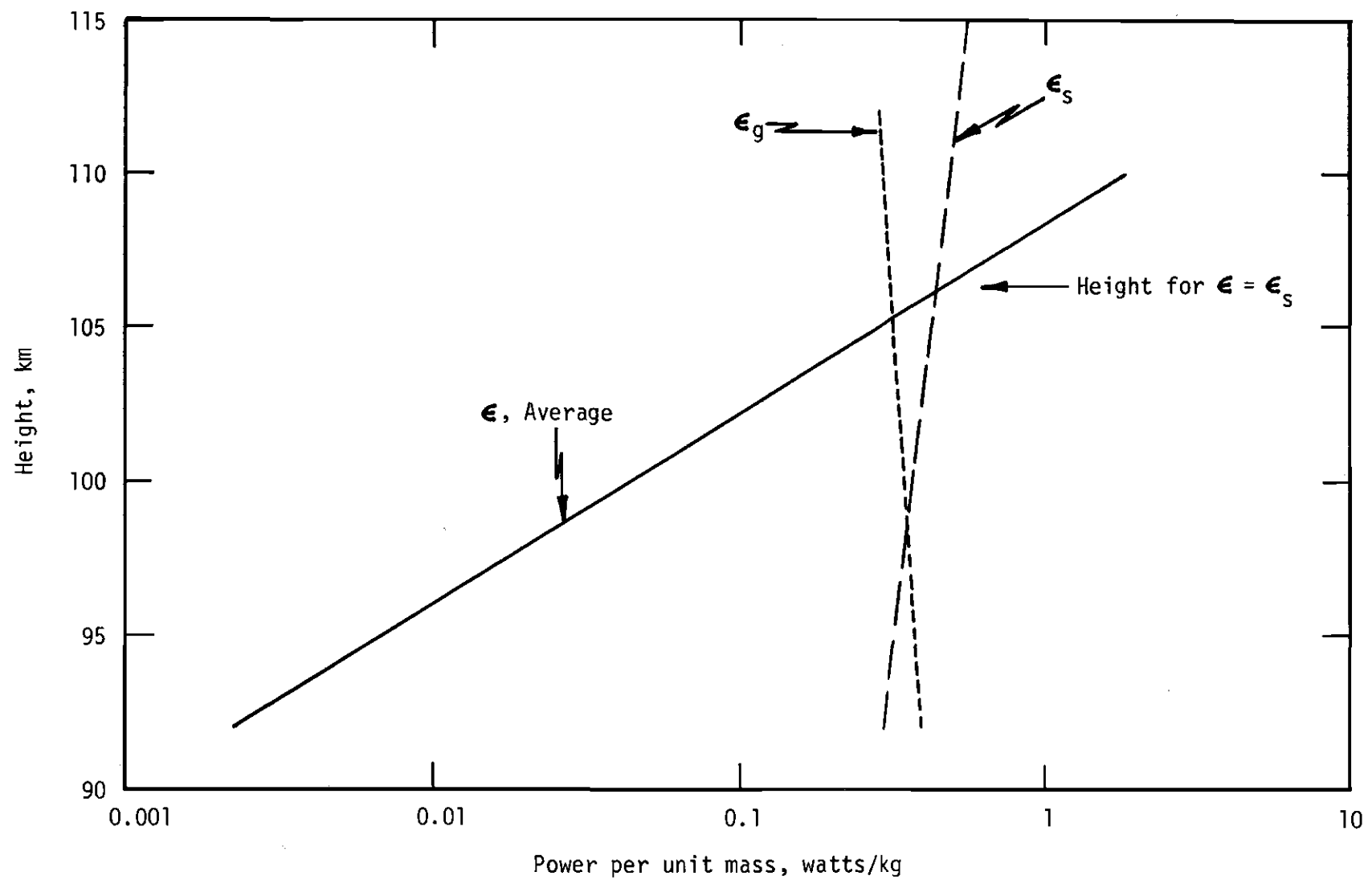
Figure 6. Height Variation of the Three Energy Balance Parameters.
