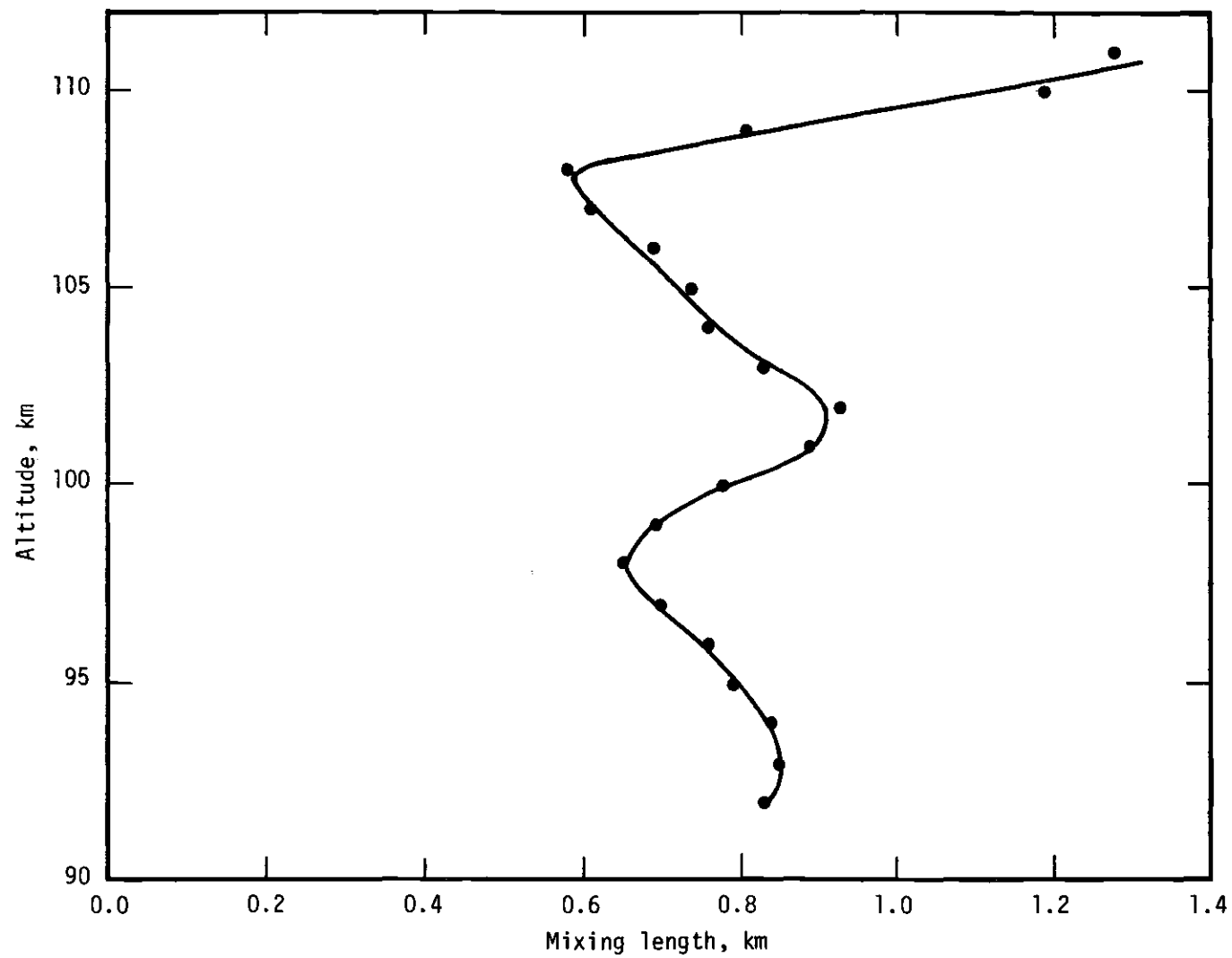
Figure 13. Mixing Length Scale versus Altitude.
