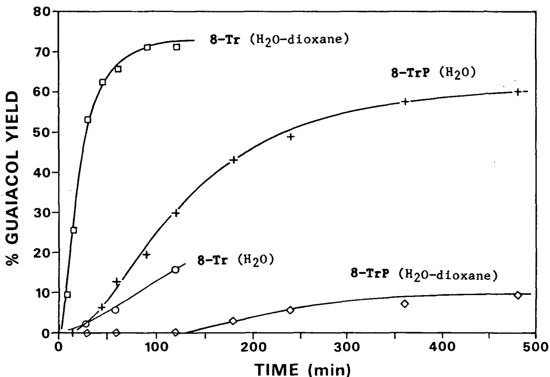
Figure 1. The relative yield of guaiacol from the kraftlike degradation of insoluble model 8-TrP and 8-Tr in aqueous and aqueous/29% p -dioxane systems.
