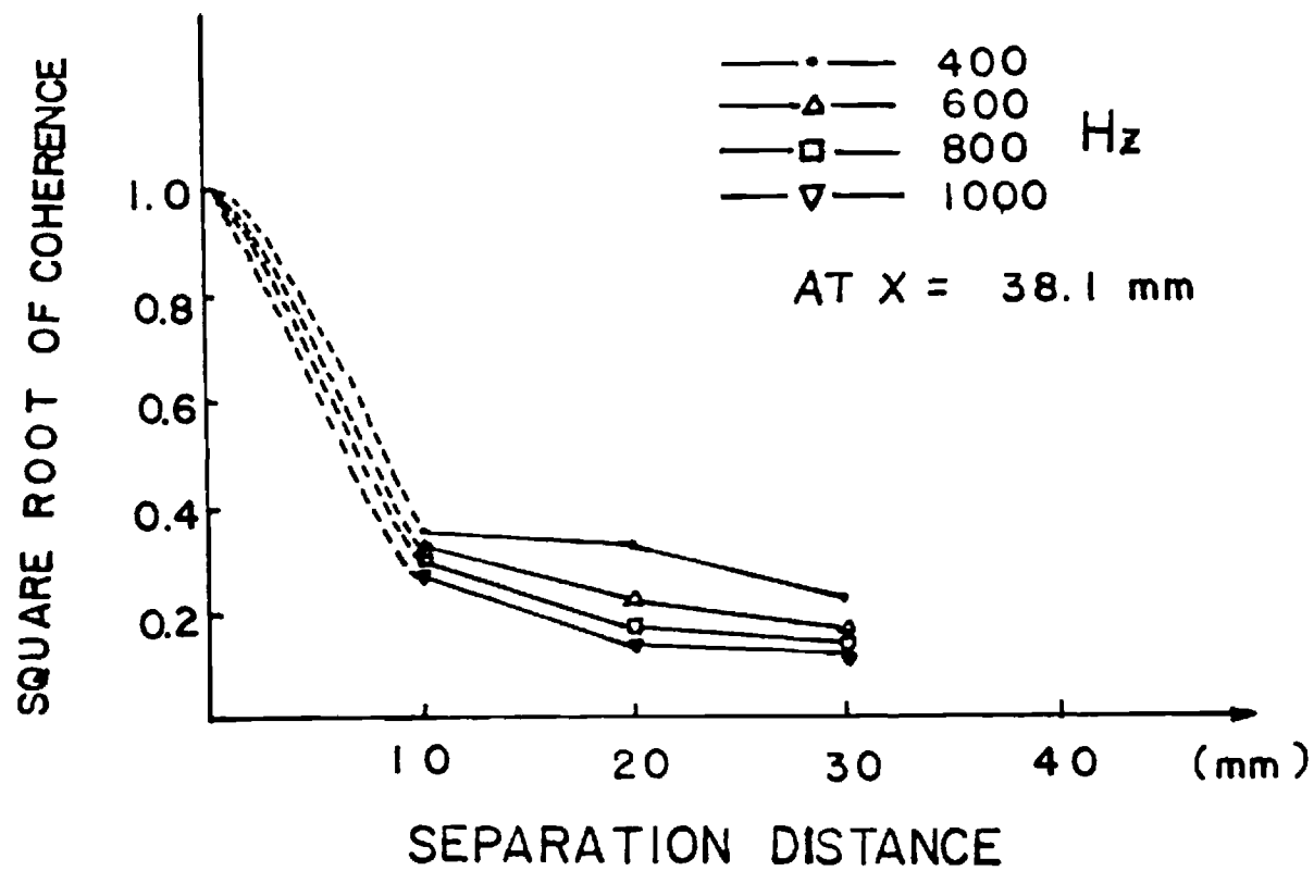
Figure 8. Square root of coherence of two space separated ion signals.
