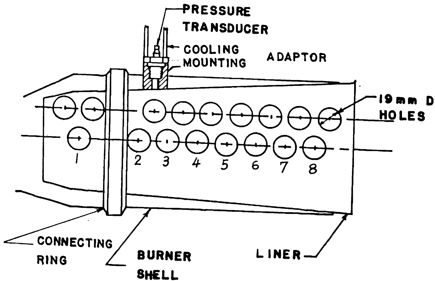
Figure 5. Sites for acoustic measurement.
