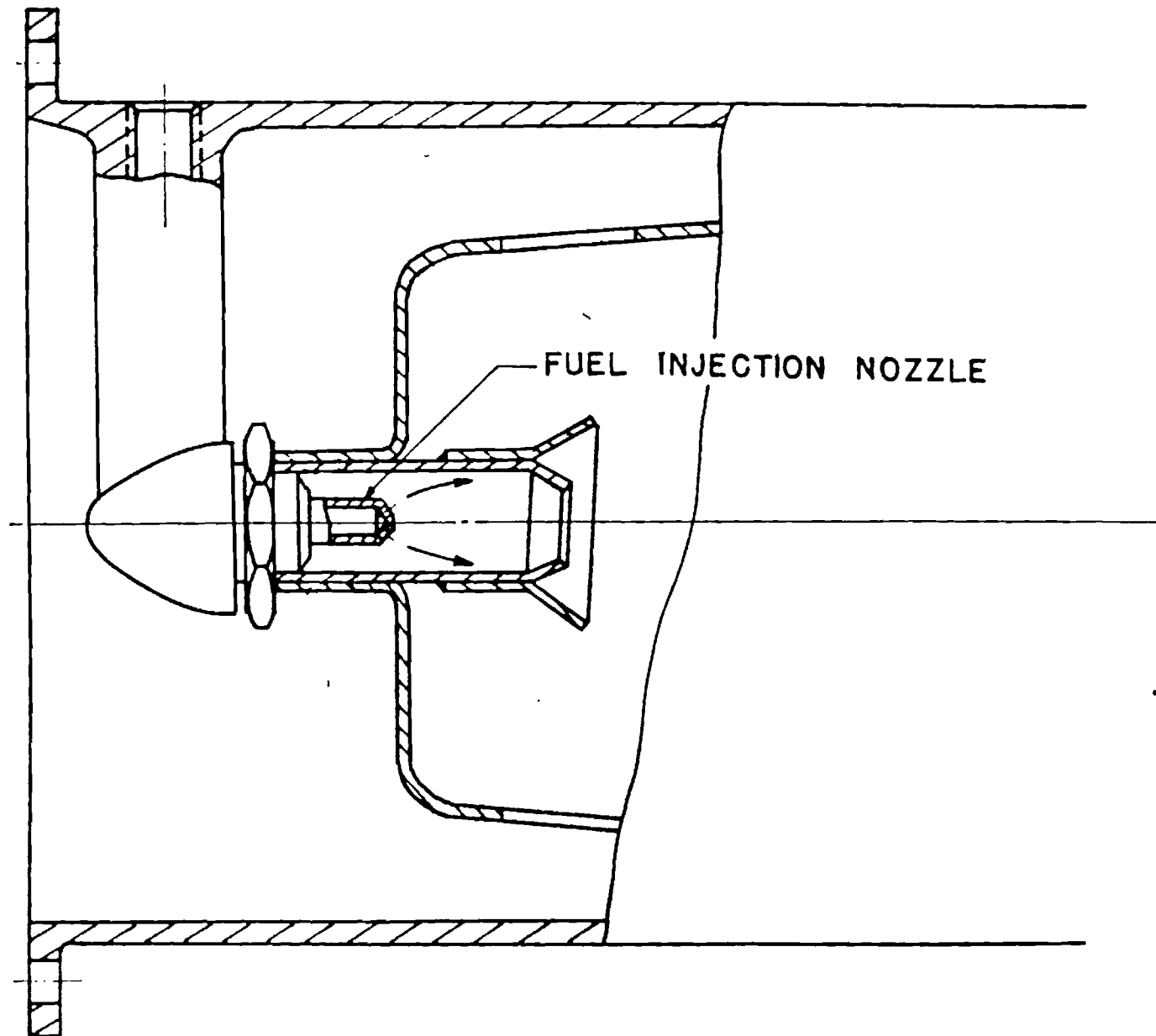
Figure 3. Long flame, no premix injector.
