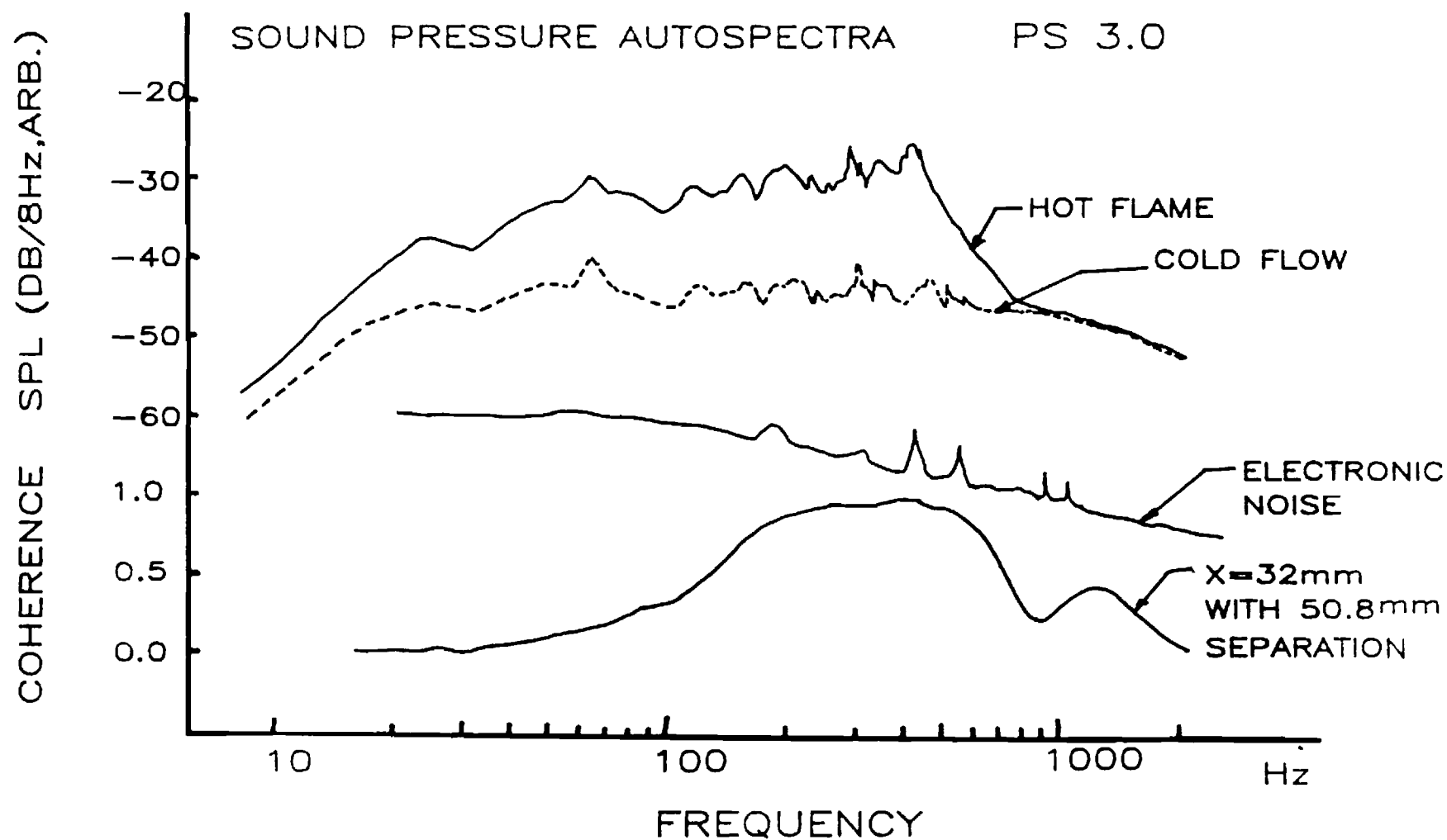
Figure 10. Typical combustion noise and cold flow noise autospectra and the coherence functions between two space-separated pressure transducers.
