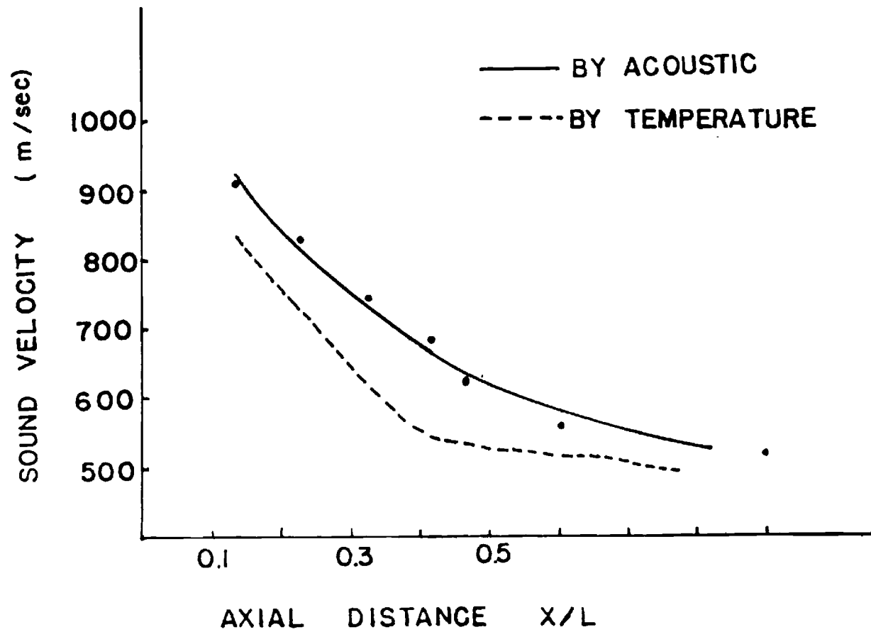
Figure 7. Comparison of speed of sound obtained from pulse technique and temperature measurements.
