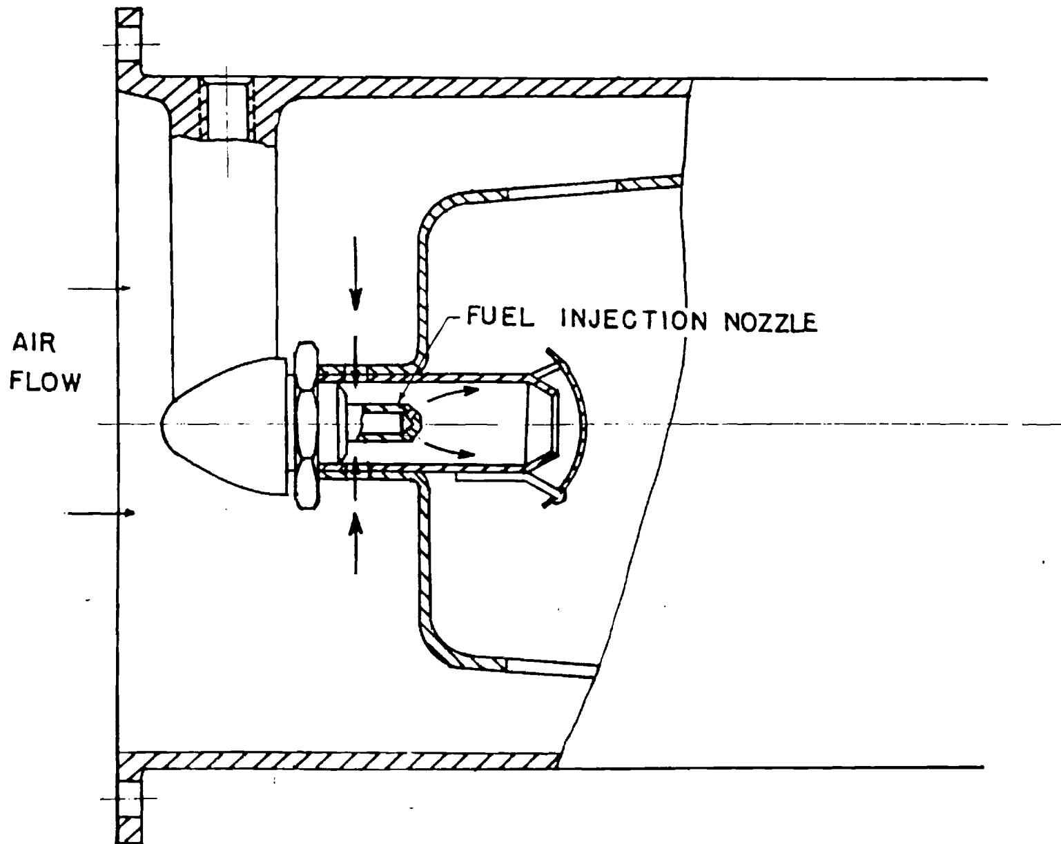
Figure 2. Short flame, partial premix injector.
