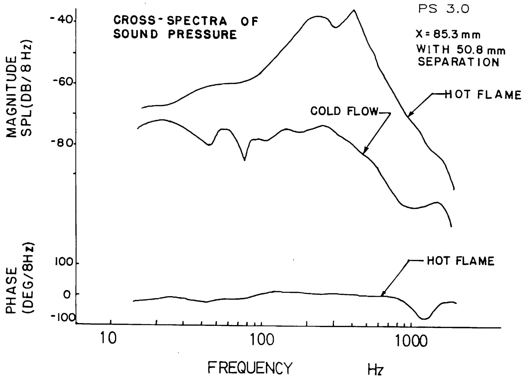
Figure 11. Typical combustion noise and cold flow noise cross-spectra.
