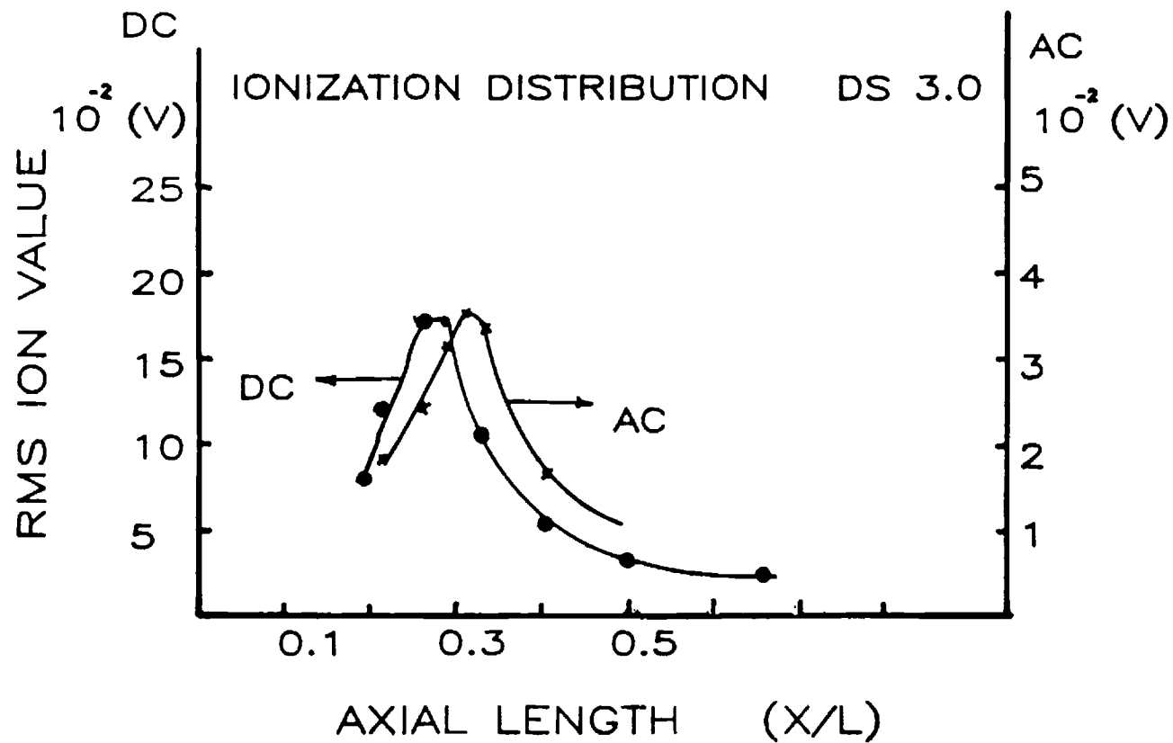
Figure 9. DC and AC ionization concentration distribution.
