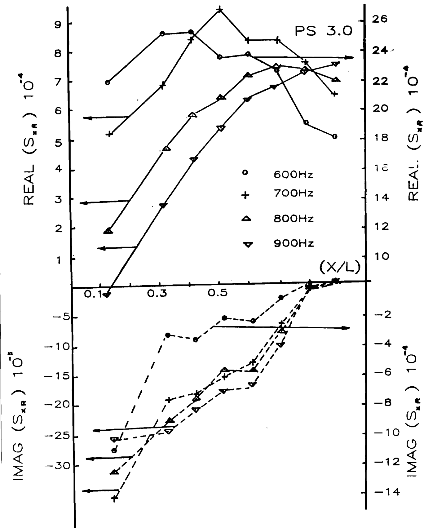
Figure 12. Typical axial variation of cross spectra between position x and a fixed reference microphone.
