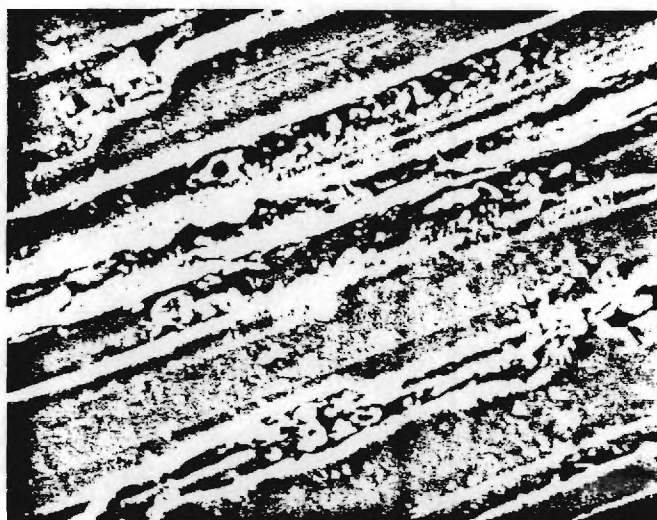
Implanted Region 1500X
