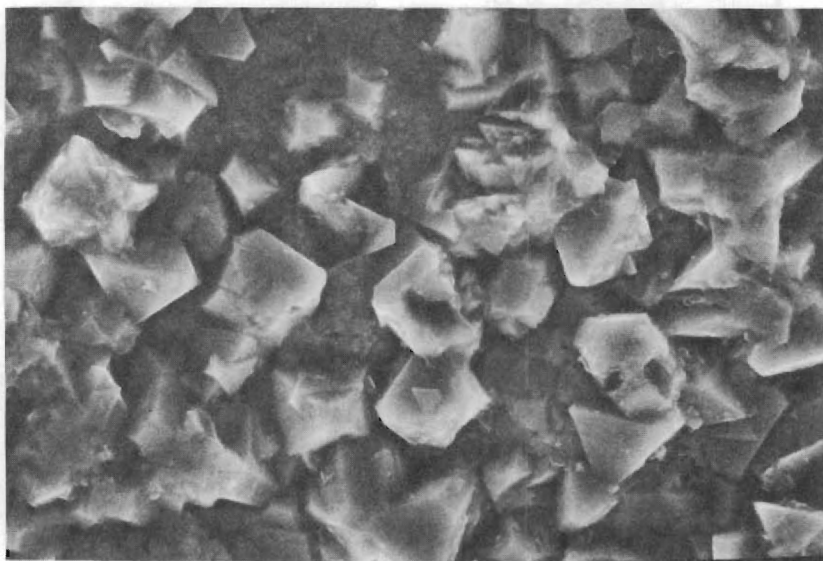
B-Implanted 1400X
