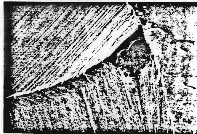
Figure 8. SEM micrographs of unimplanted tap after 50 uses. Third and fourth crest are illustrated at higher magnification.
