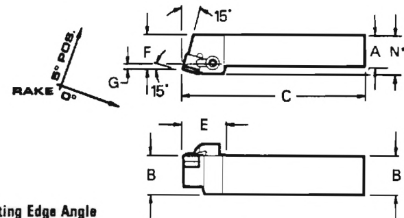
Offset Shank 15° Side Cutting Edge Angle for Straight Turning
