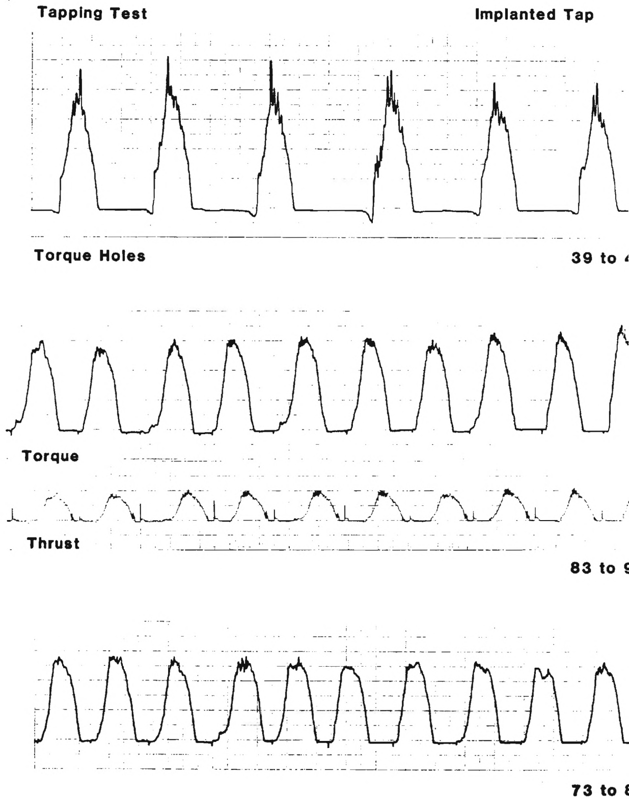
Figure 7. Tapping torque and thrust when implanted taps are used. Note that torque variation with location along test bar dominates.
