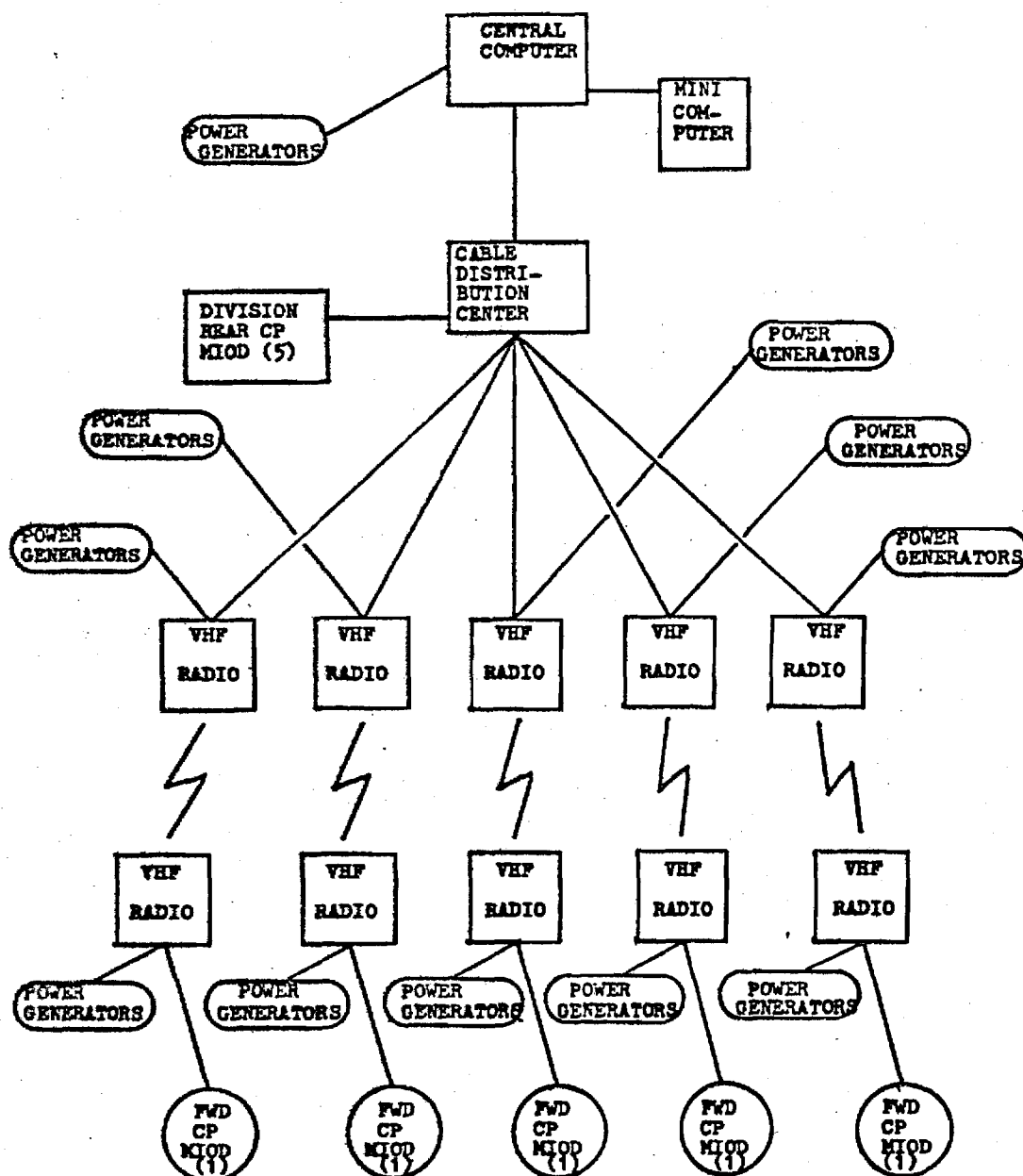
Figure 4. An Example of a Command and Control System
