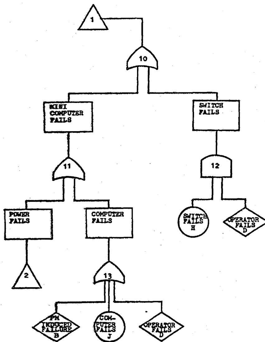
Figure 5. Fault Tree for C & C System, Continued
