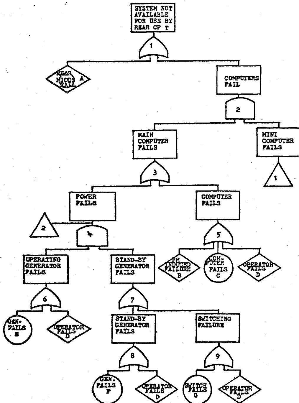
Figure 5. Fault Tree for C &amp; C System
