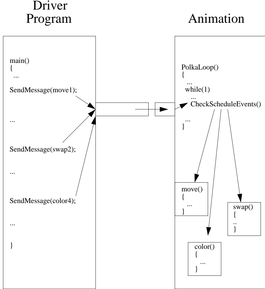
Figure 1: Model of program to animation communication in the Polka-RC framework.
