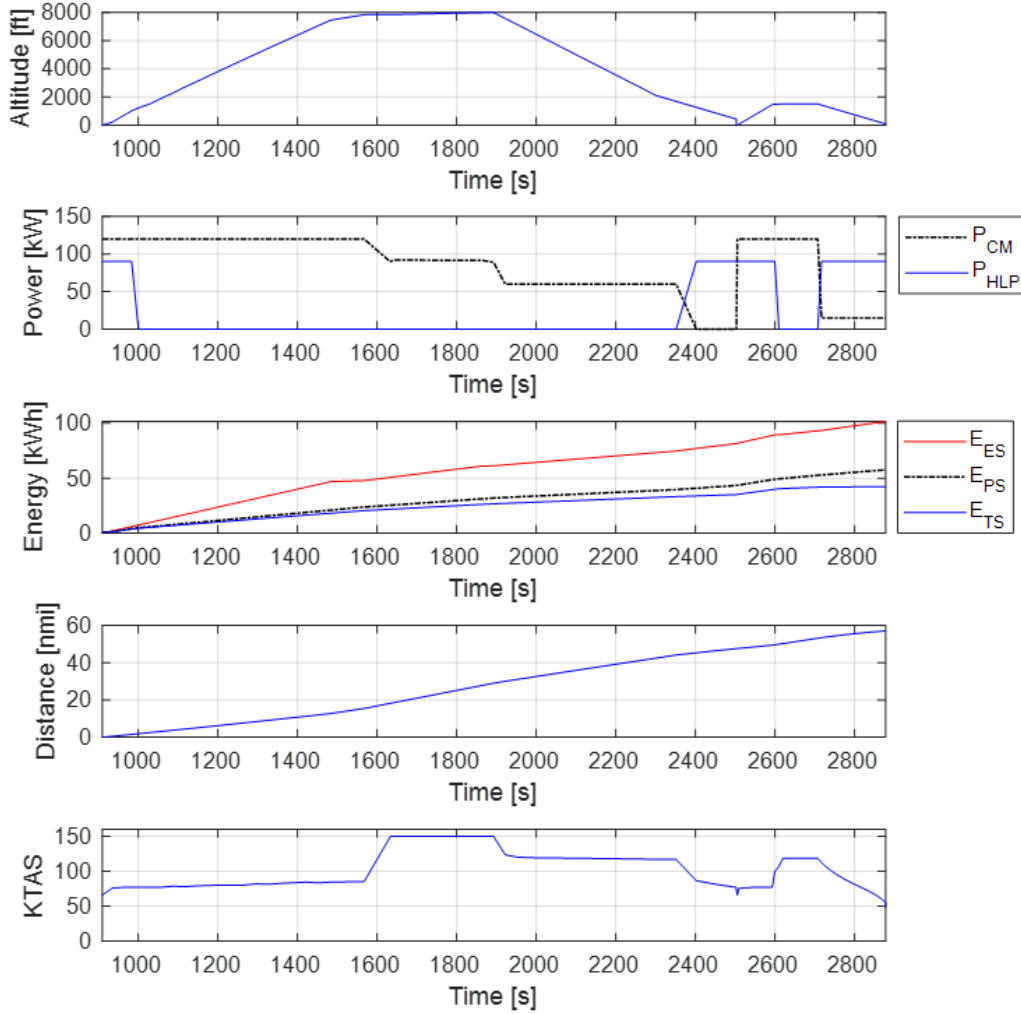
Figure 8 Mission performance analysis results compared to data obtained from Chin et al. (2017).
