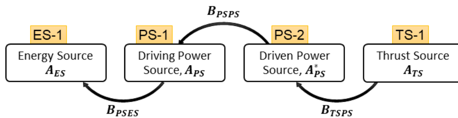
Figure 3 Property propagation from upstream to downstream sources by Interdependency and Property Matrices.
