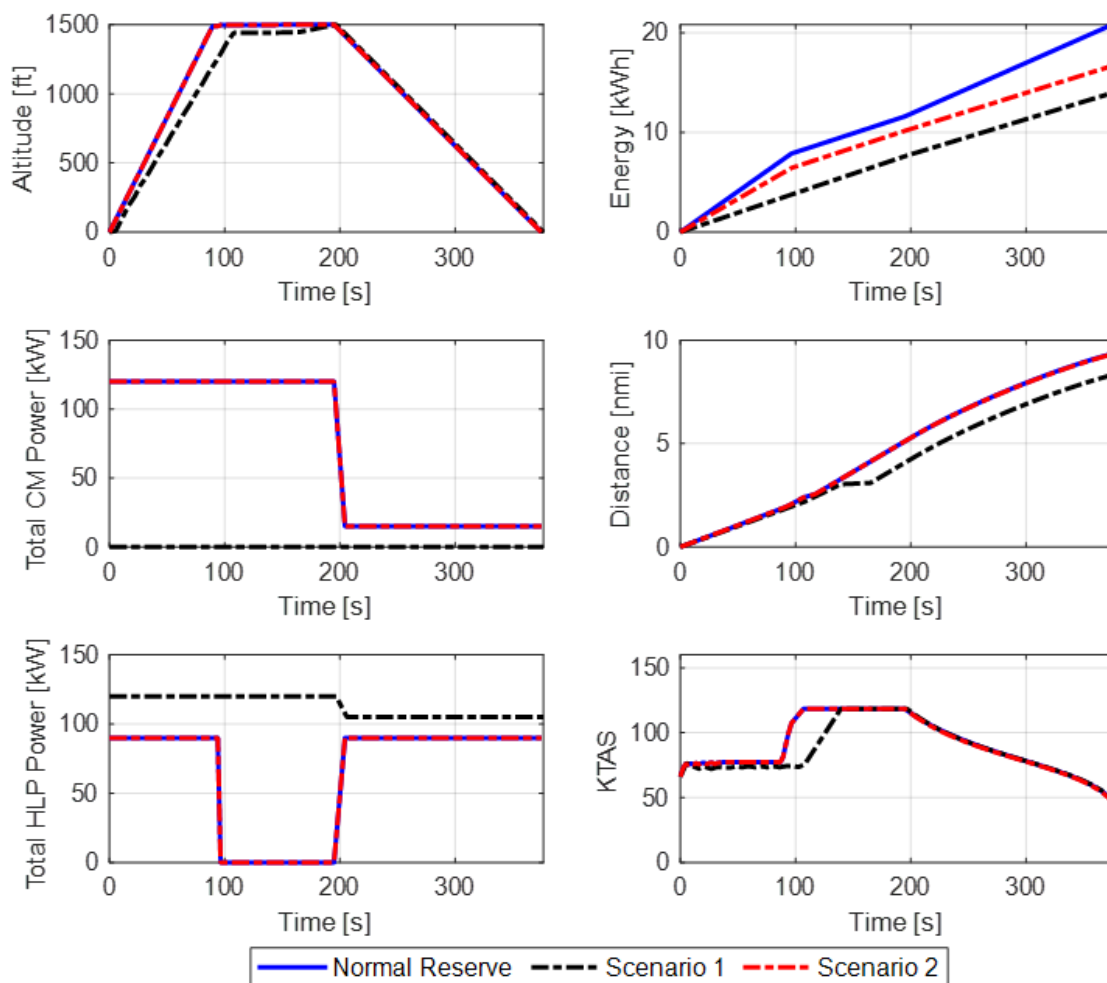
Figure 9 Mission performance and power schedule comparisons of normal reserve mission and motor failure scenarios.
