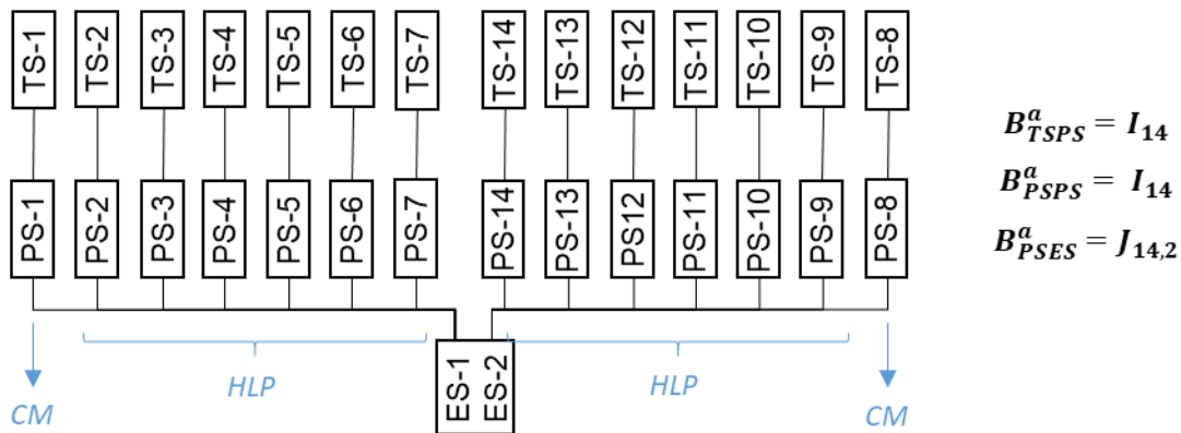
Figure 6 Simplified X-57 architecture based on Clarke et al. (2017) and corresponding Architecture Matrices.
