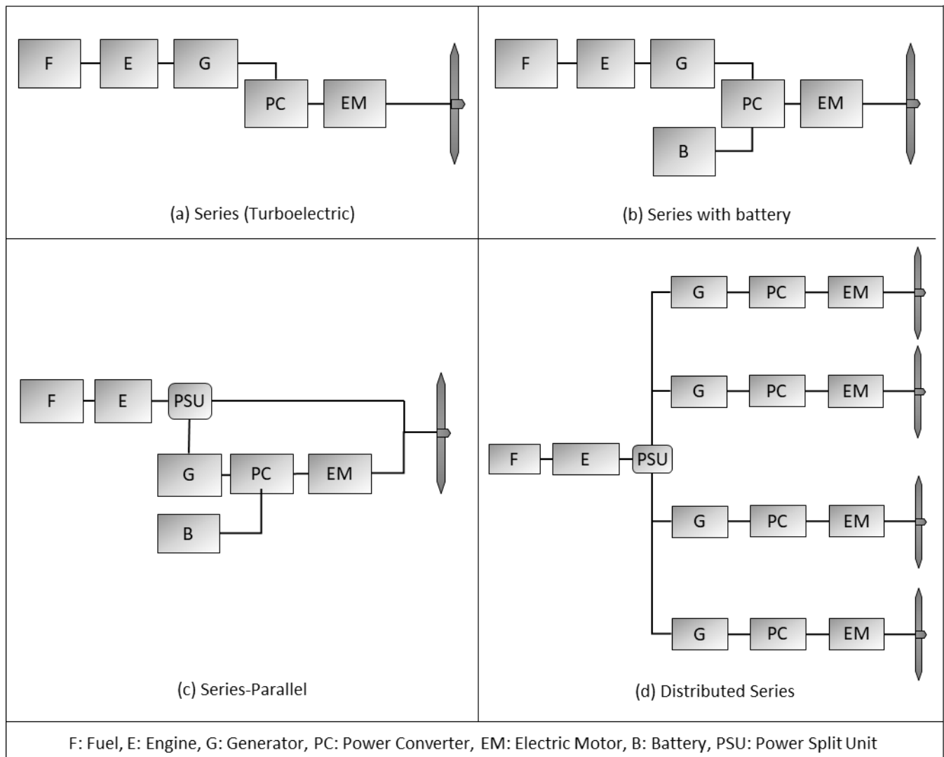
Figure 1 Notional series configurations used in different hybrid electric propulsion architectures.
