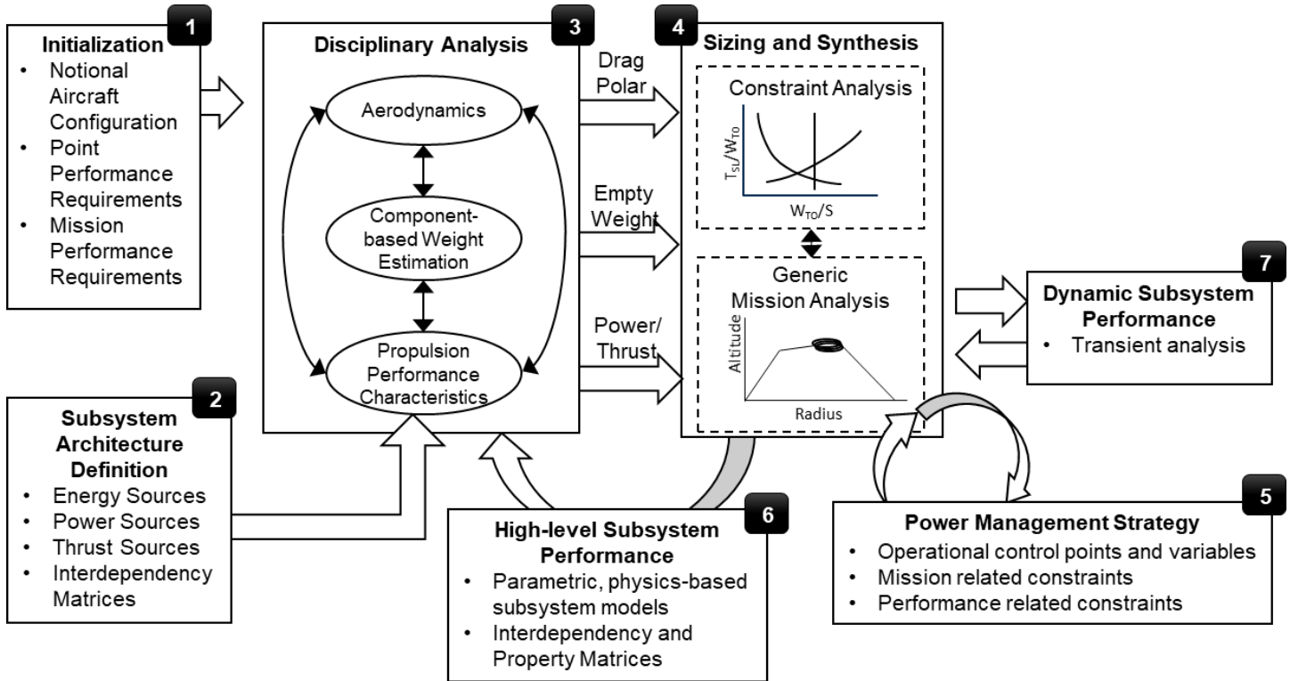
Figure 2 Building blocks of the methodological framework: E-PASS.
