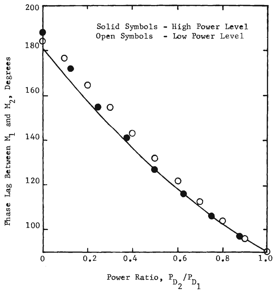
Figure 9. Effect of Driver Power Ratio on the Pressure Phase Lag.
