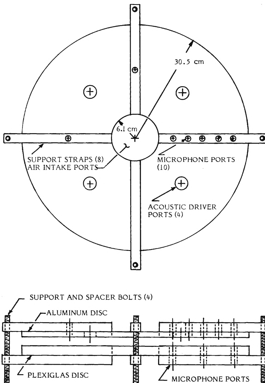
FIGURE 5 SPINNING WAVE ENGINE TEST MODEL
