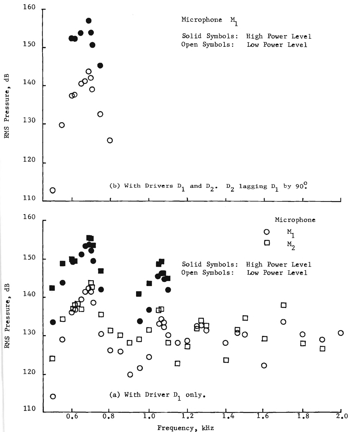
Figure 8. Effect of Driver Frequency Upon the Oscillatory Pressure.
