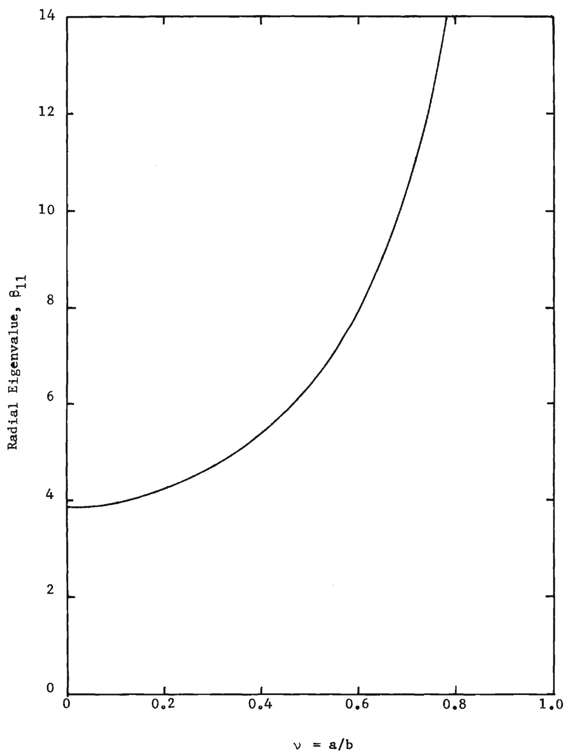
Figure 1. Radial Eigenvalues for Open Annuli for n = 1 .
