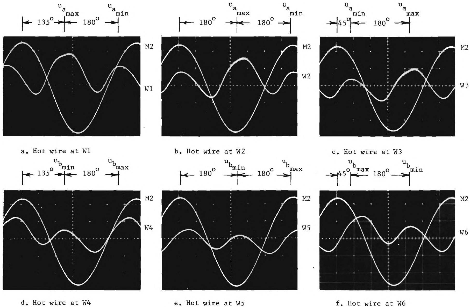
Figure 23. Microphone and Hot-Wire Traces at 6 Hot-Wire Locations. f = 693 Hz.
