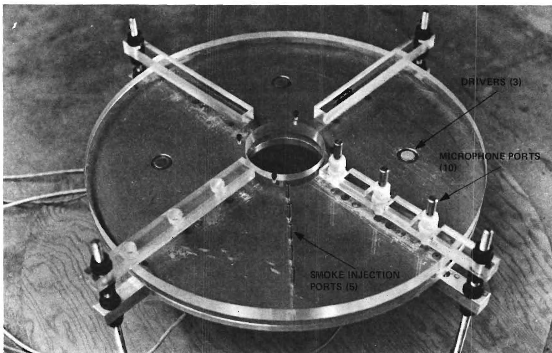
Figure 6. SPINNING-WAVE TEST MODEL
