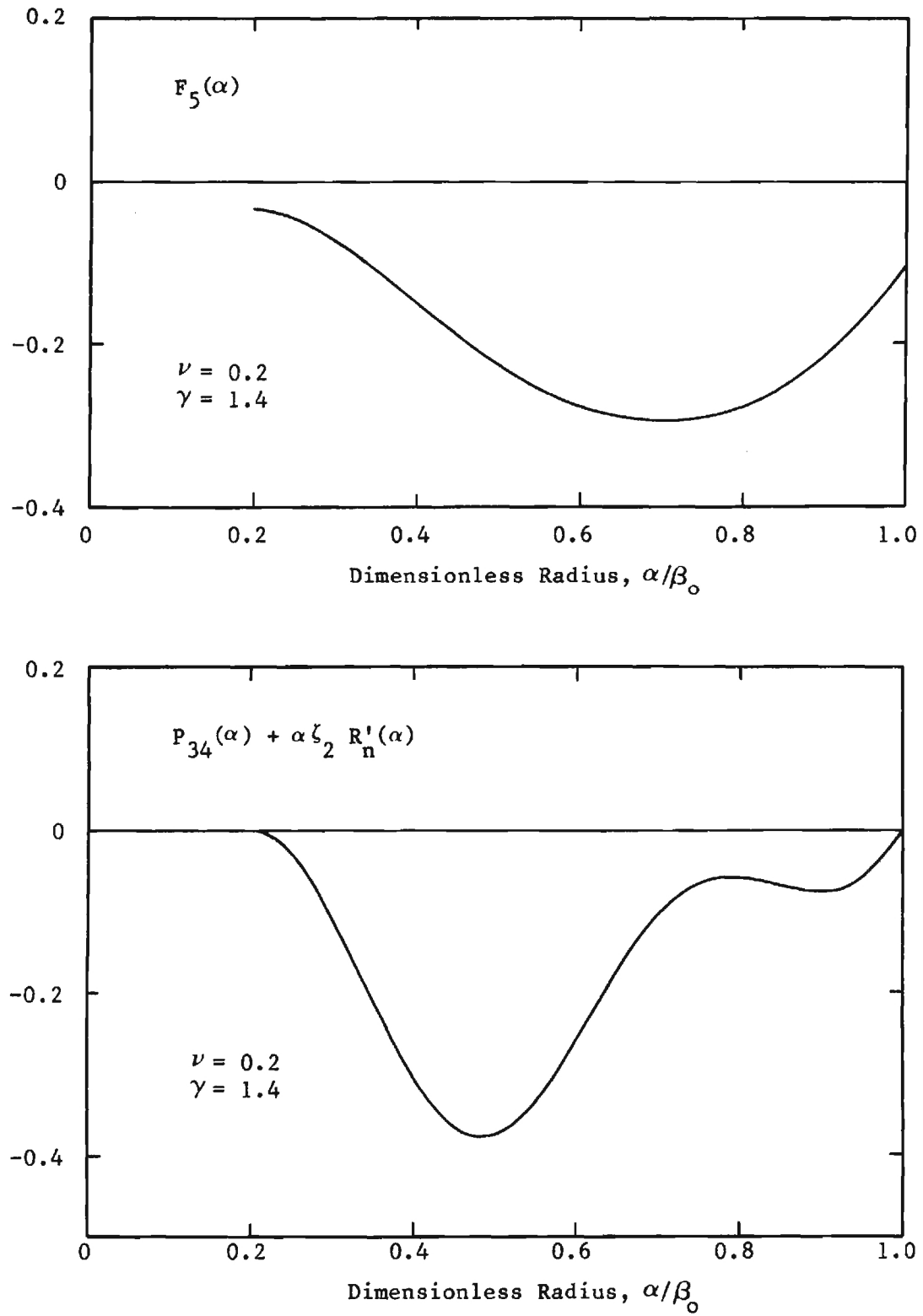
Figure 9. Third Order Function F_5(\alpha) and Corresponding Pressure Function P_{34}(\alpha) for Spinning 1T Mode.
