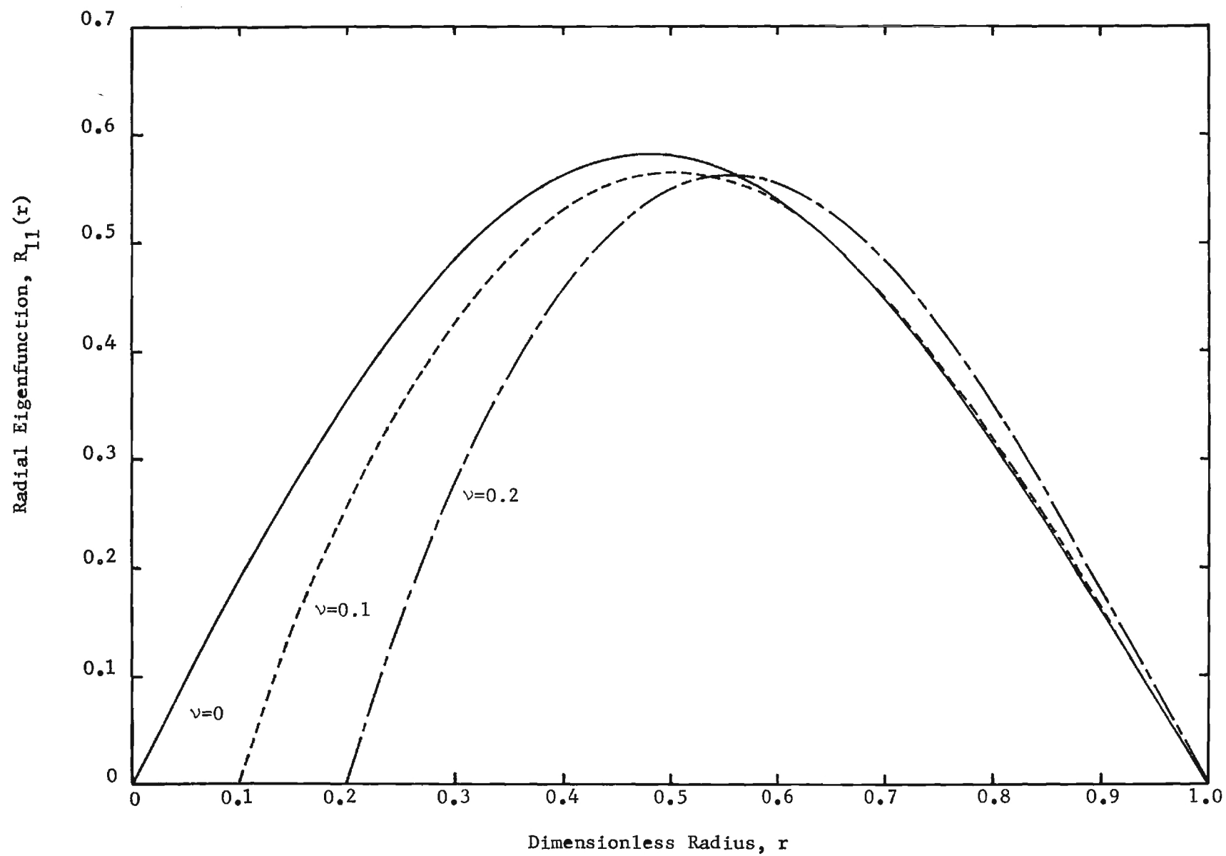
Figure 2. Radial Eigenfunctions for Open Annuli for n = 1 .
