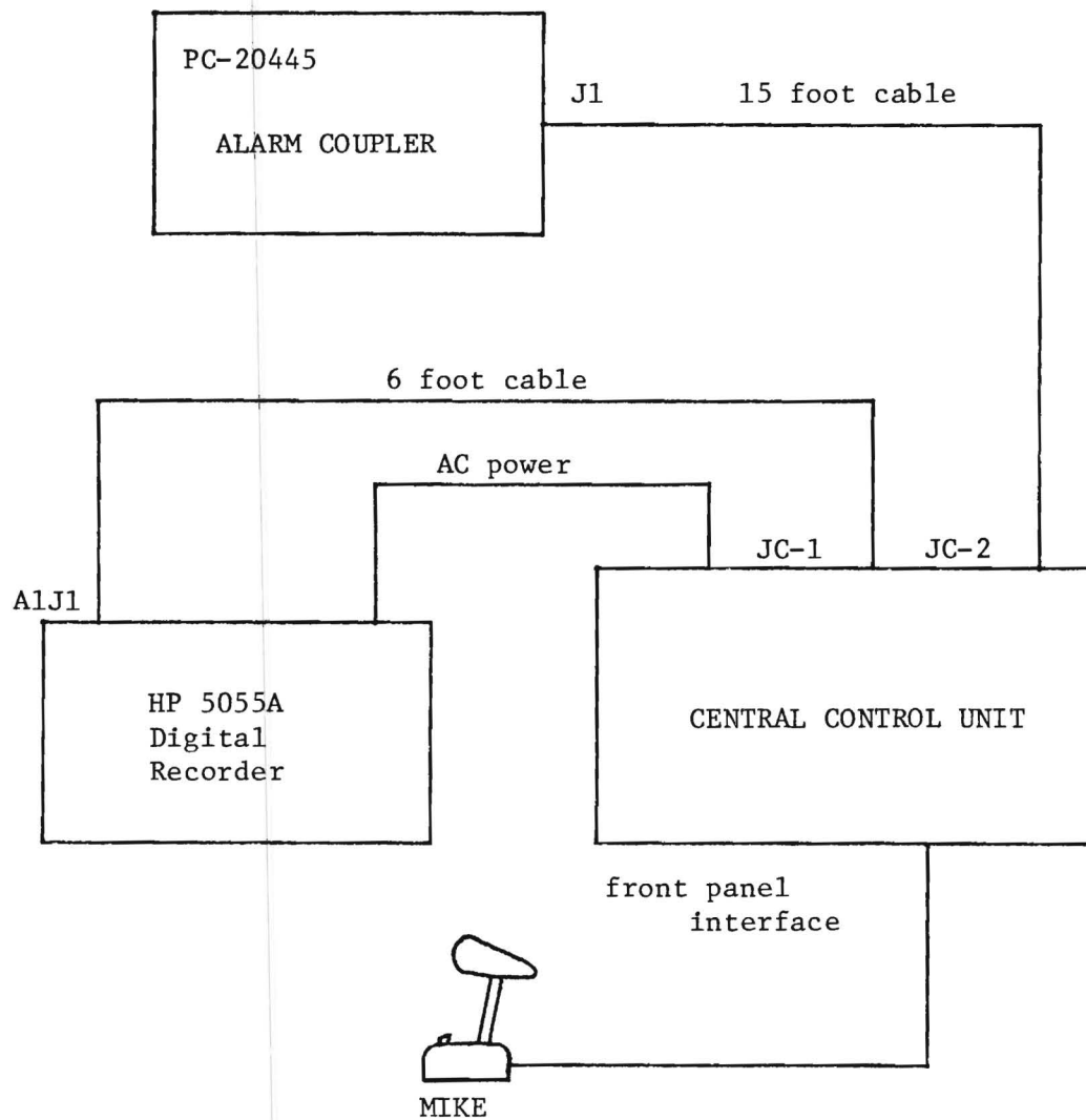
Figure 5. Central Control Unit Cable Interface Diagram
