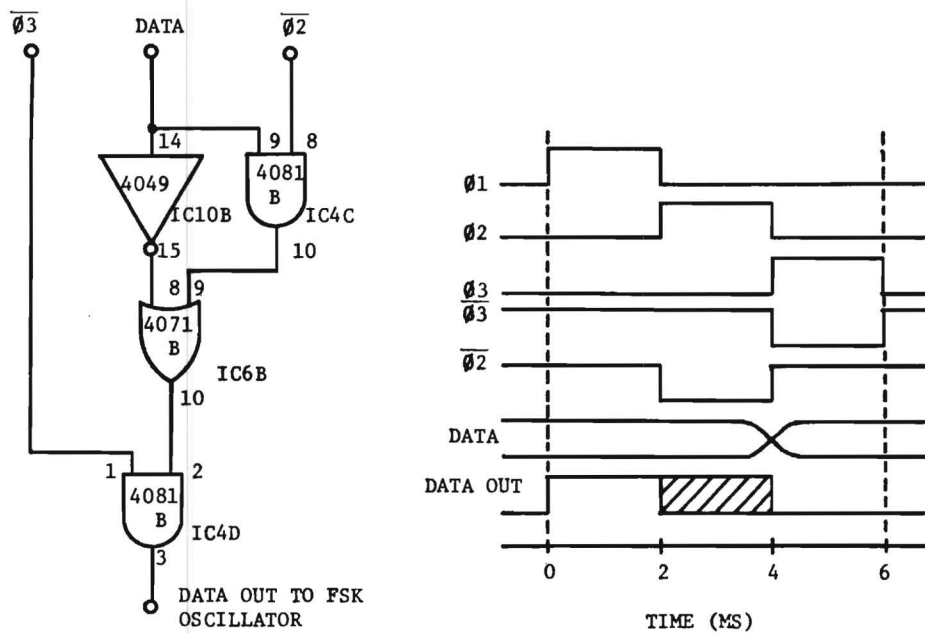
Figure 8. PDM Forming Logic
