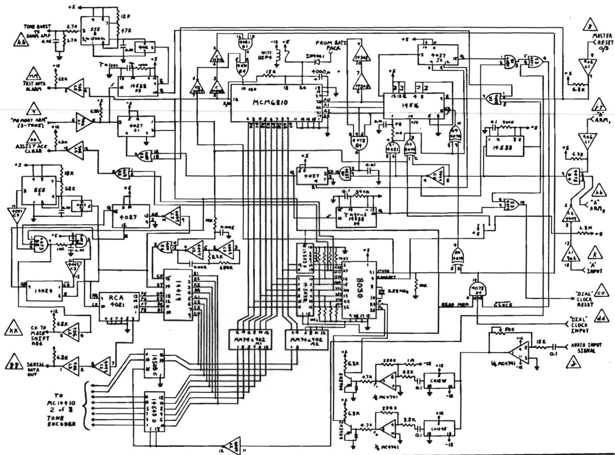
CB-AIDS REMOTE STATION AUTO TELEPHONE DIALER, TELEPHONE INTERCONNECT-4 DRAWING NO: CBRS-5
