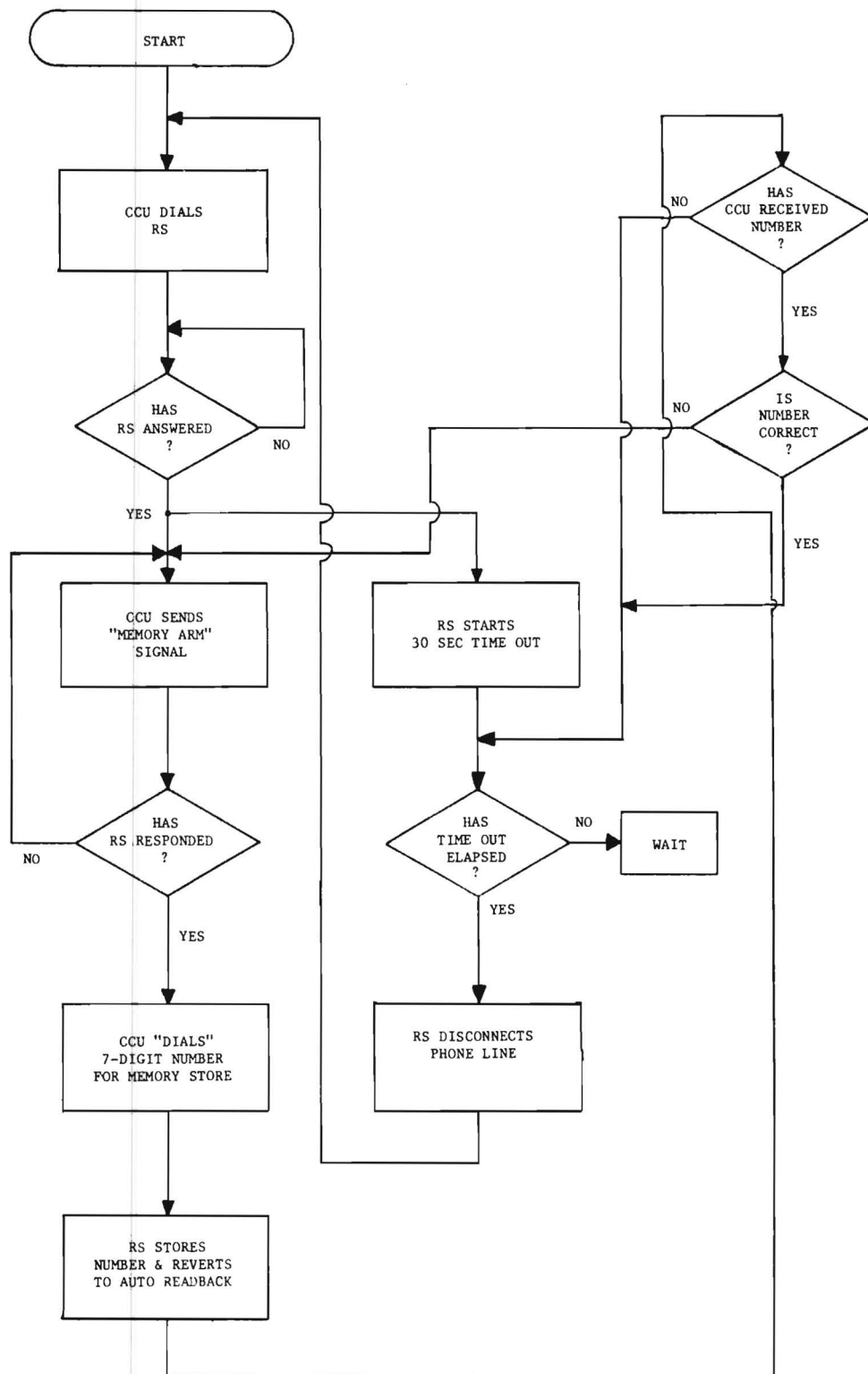
Figure 6. CCU/RS Telephone Number Store Flow Chart.
