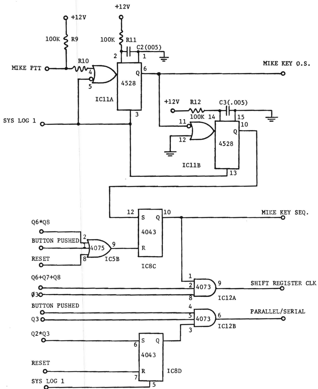
Figure 6. Microphone Derived Control Signals and Shift Register Control Signals
