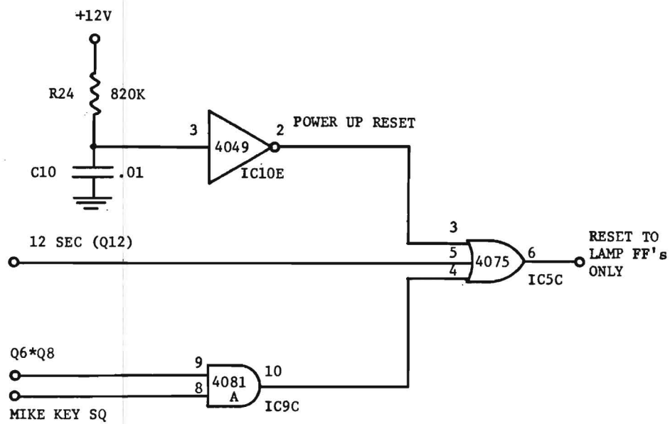
Figure 11. Master Reset Circuit
