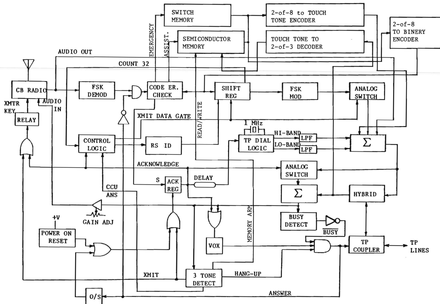
Figure 5. Remote Station Block Diagram.
