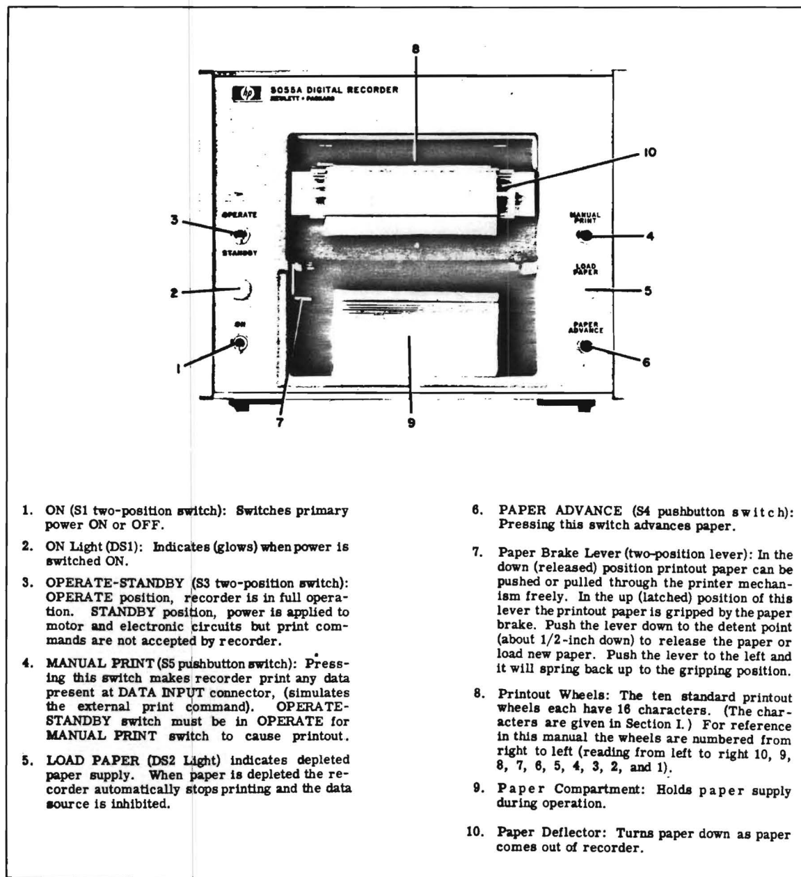
Figure 3. Digital Recorder Front Panel
