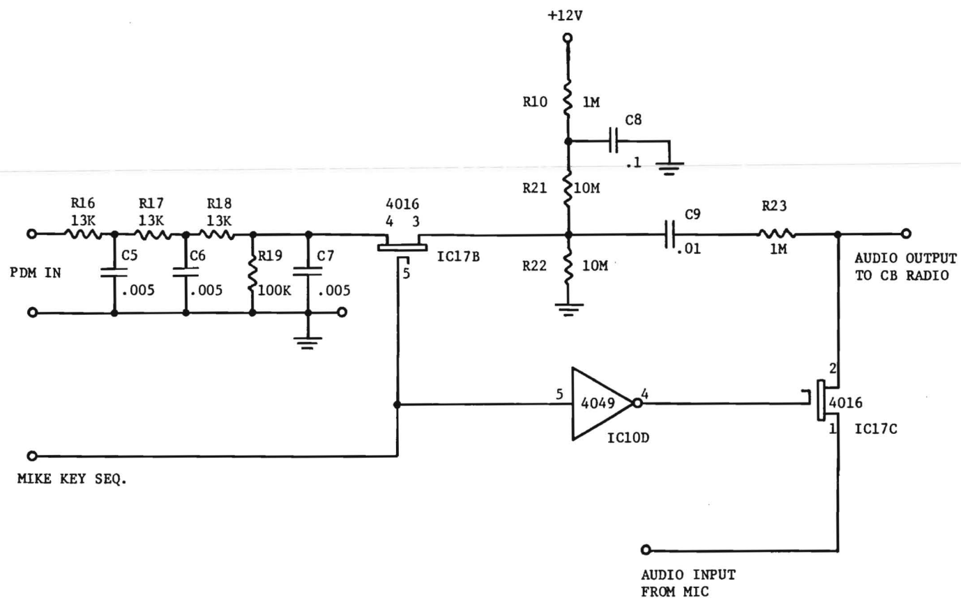
Figure 10. Output Circuit
