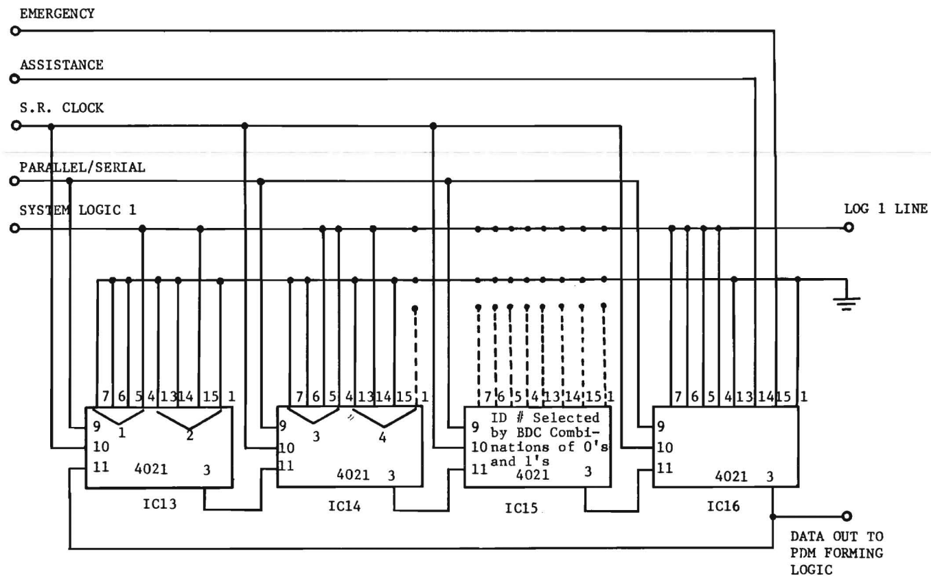
Figure 7. Shift Registers
