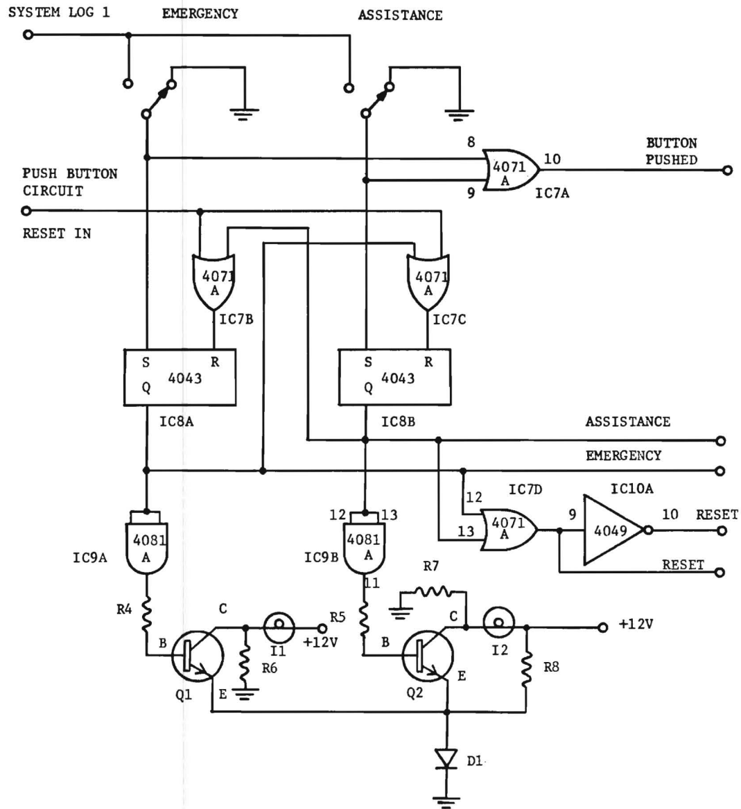
Figure 5. Pushbutton Circuit
