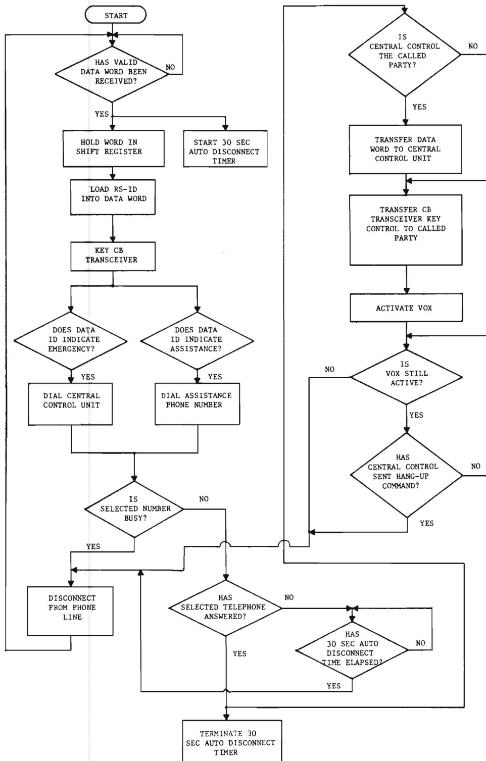
Figure 4. Remote Station Flow Chart.
