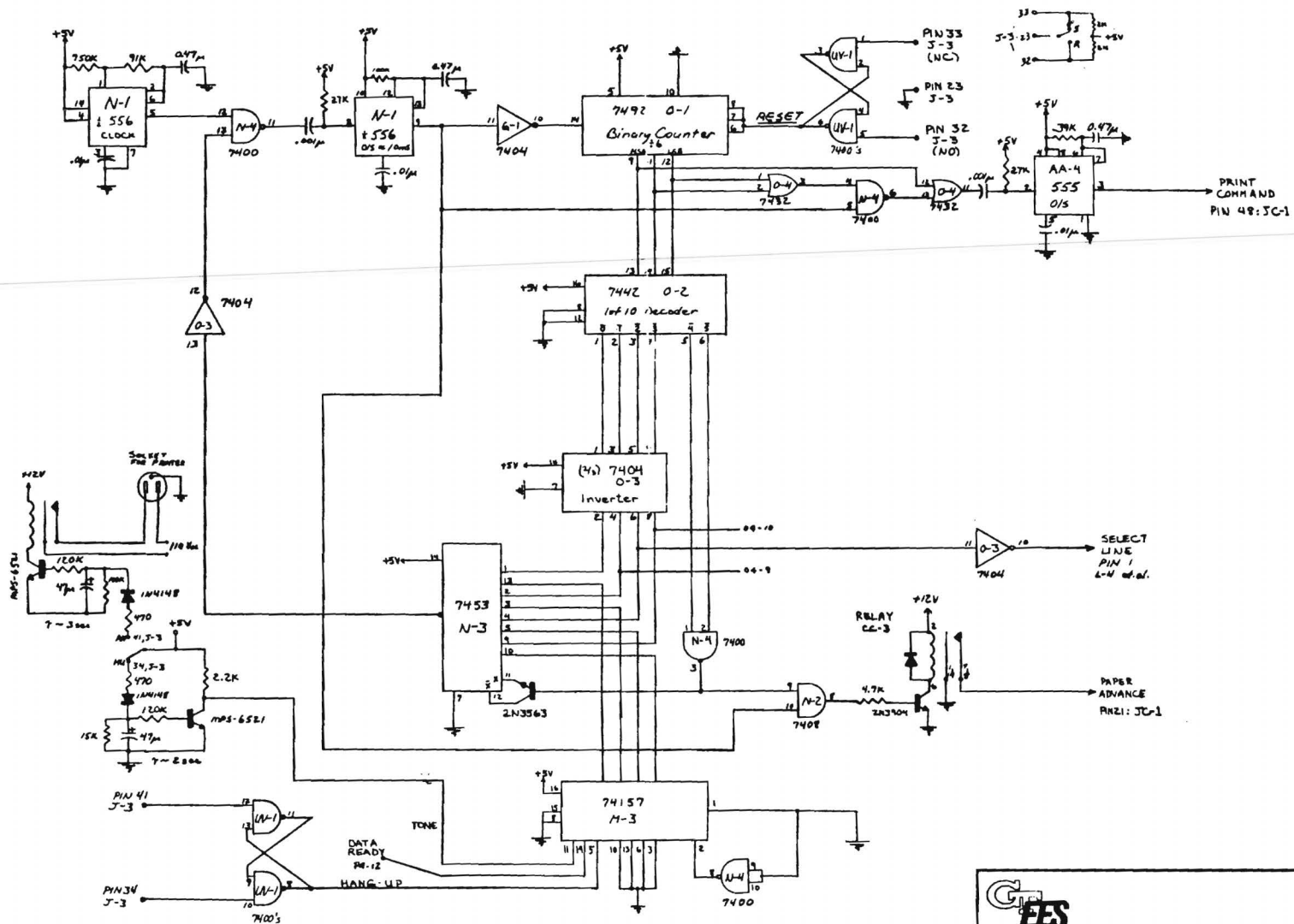
CB-AIDS CENTRAL CONTROL UNIT SEQUENCER DRAWING NO. CBCCU-1
