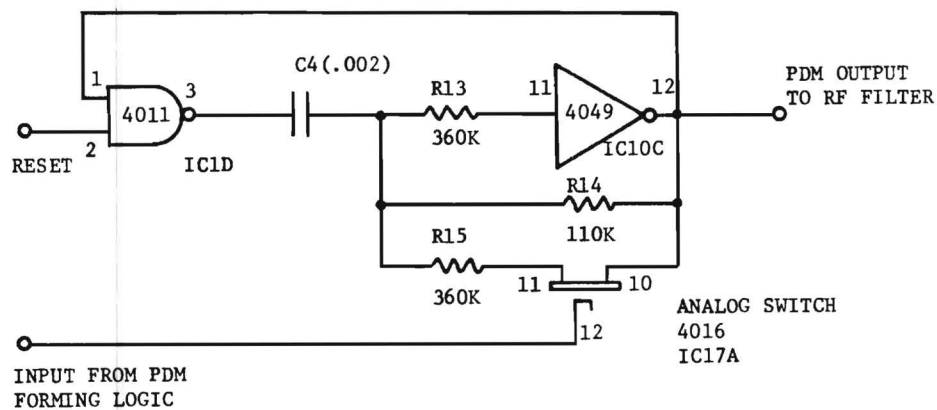
Figure 9. FSK Oscillator
