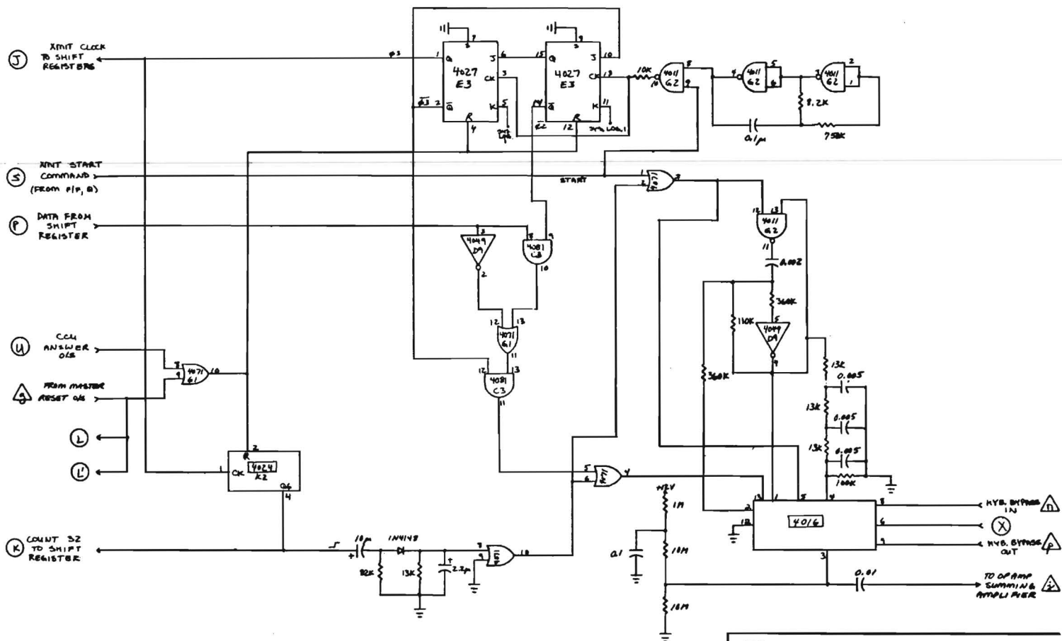
CB-AIDS REMOTE STATION DIGITAL WORD PROCESSOR-3 DRAWING NO: CBRS-9
