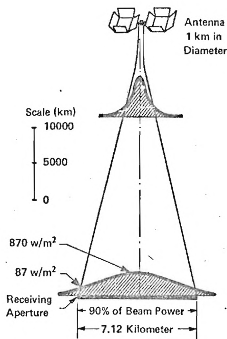
Figure 2. Microwave Transmission to Earth 11
