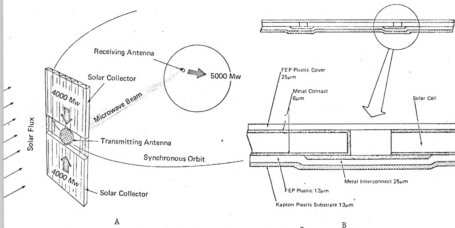
Figure 1. A) Geosynchronous Solar Power Plant 9 B) Solar Cell Array Construction 10
