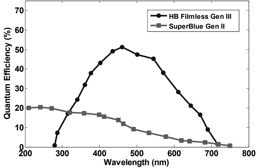
Figure 8. Quantum efficiency variation of the Gen III filmless intensifier used for this work in comparison to the Gen II (Super blue) intensifier used by previous researchers.
