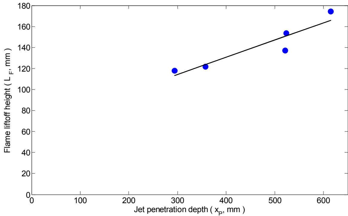
Figure 48. Measured flame liftoff height in all the tested full length SPRF configurations correlated with the corresponding jet penetration estimated from the jet against uniform flow model [26].
