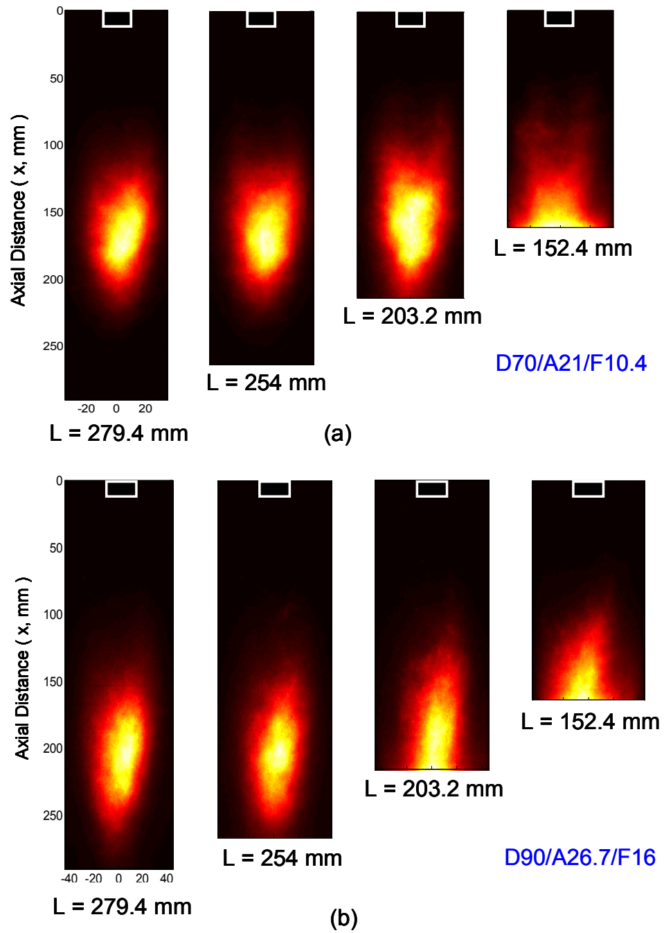
Figure 46. Mean chemiluminescence images acquired in (a) ‘D70/A21/F10.4’ and (b) ‘D90/A26.7/F16’ configurations at different combustor lengths.
