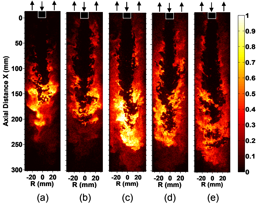
Figure 20. Instantaneous PLIF images covering the whole combustor at \phi=0.65 at loadings of (a) 2 (b) 4.5 (c) 7.2 (d) 9.4 and (e) 10.7 g/s. Reynolds number based on injector diameter ( Re_j ) is estimated to vary from 10,000 to 57,000 for lowest to the highest loading case.
