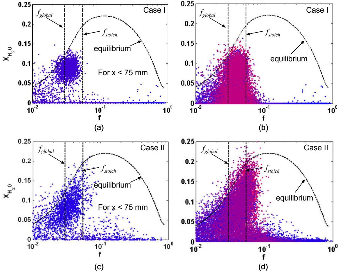
Figure 38. Distributions of instantaneous \text{H}_2\text{O} mole fraction including data points acquired in the combustor (both along the center and radial lines at different axial distances), in the non-premixed SPRF combustor for both cases in Table 7 (loading of 8.1g/s, \phi=0.6 ). Data points color coded based on the distance from the injector (blue at injector and red at the stagnation plate). Equilibrium \text{H}_2\text{O} concentrations along with the global and stoichiometric mixture fractions are shown in dotted lines for reference.
