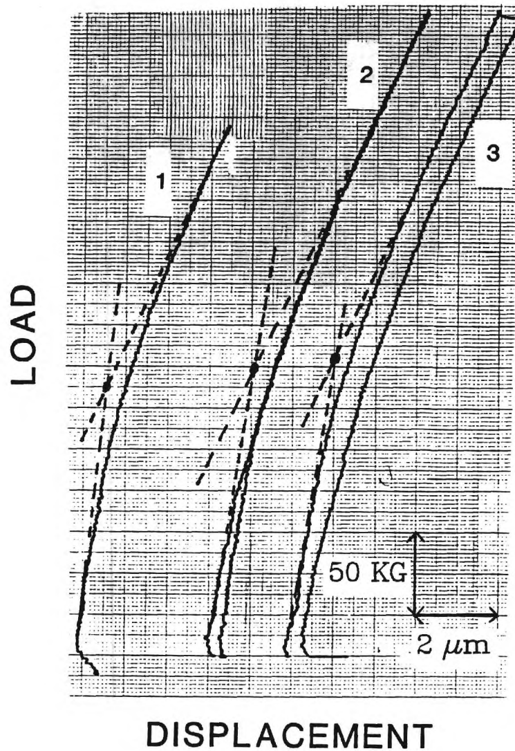
Fig. 19 - Load displacement curves for specimen with notch only. Measurements were taken with 1) back-face strain gage, 2) clip gage, 3) laser extensometer.
