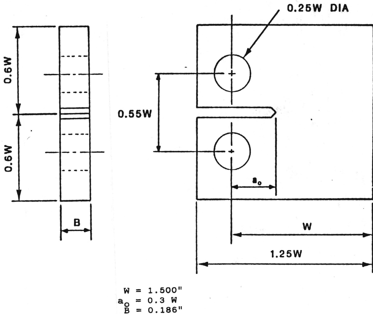
Fig. 5 - Standard ASTM fatigue crack propagation specimen.
