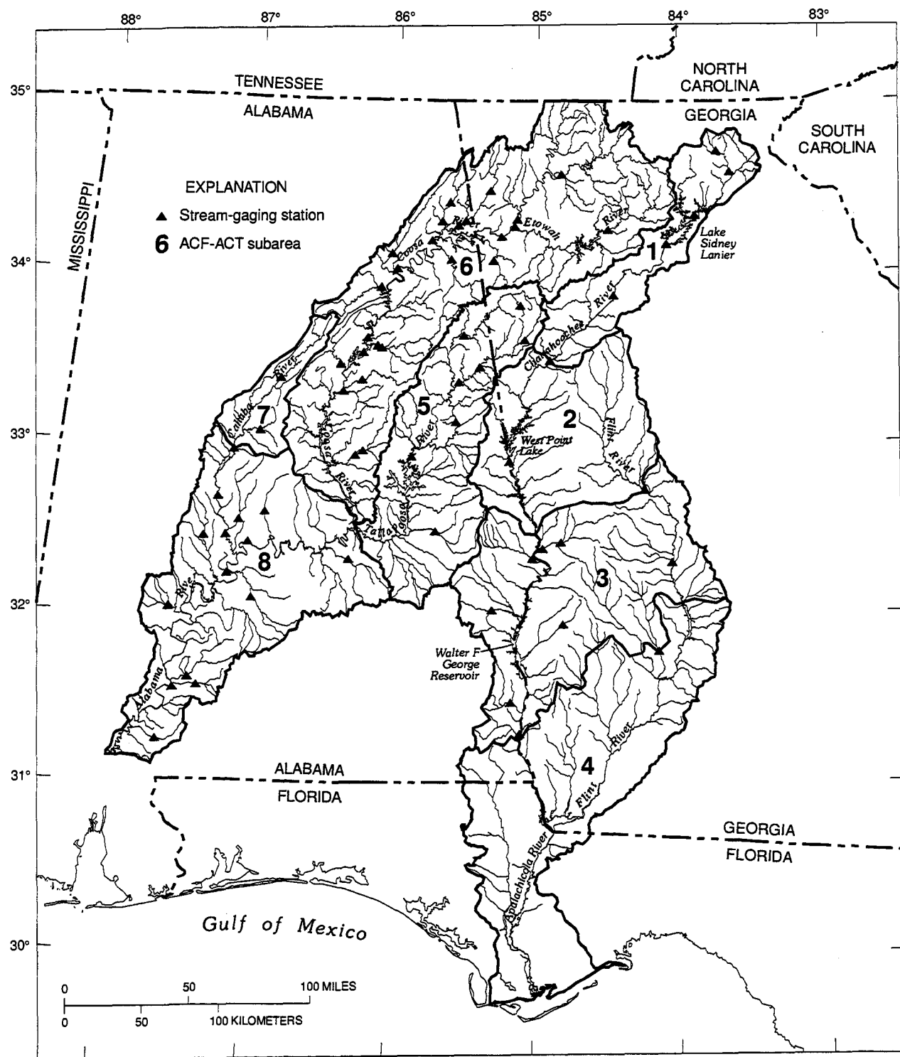
Figure 1. Location of subareas, major streams, and selected gaging stations in the Apalachicola–Chattahoochee–Flint (ACF) and Alabama–Coosa–Tallapoosa (ACT) River basins.
